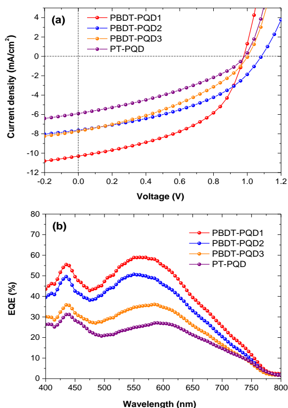
Fig. 4 (a) Current density-voltage characteristics of the four copolymer:PC 71 BM solar cells; (b) External quantum efficiency (EQE) spectra measured under illumination of monochromatic light.
