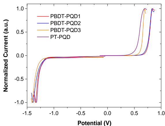
Fig. 2 Square wave voltammeteries (SWV) of the four copolymers.
