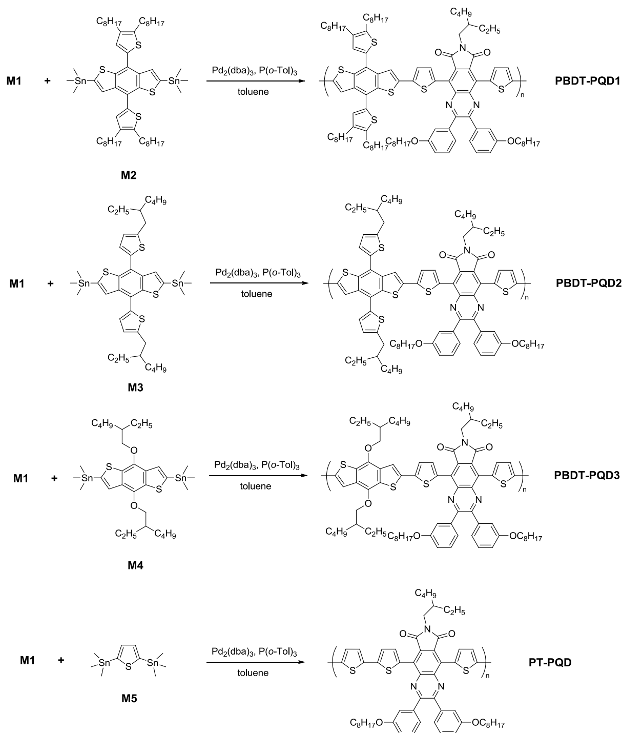
Scheme 3 Synthetic routes of the four copolymers.
