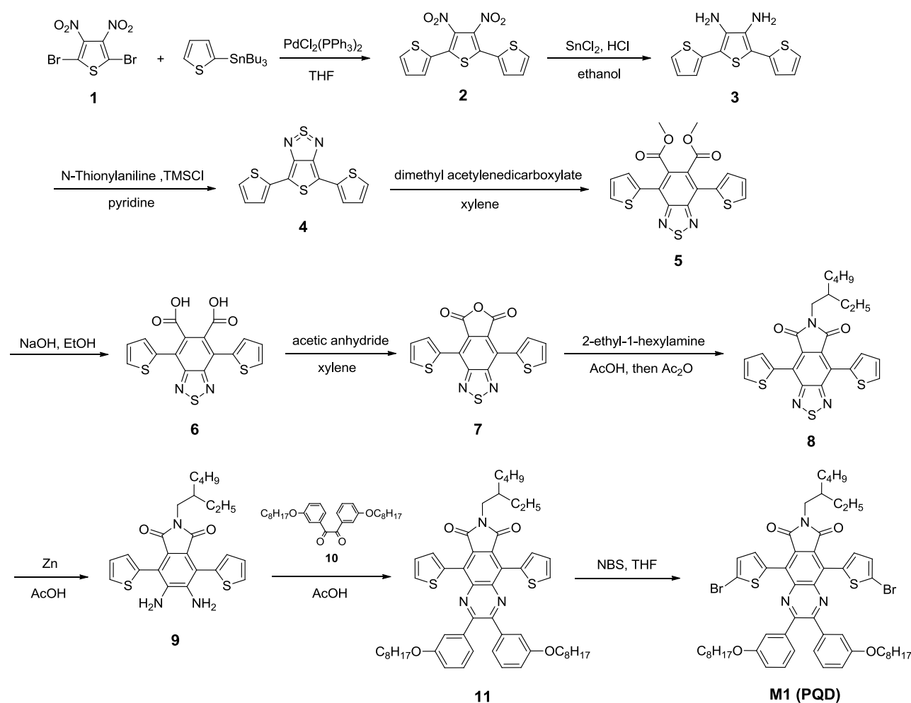
Scheme 2 Synthetic routes of the monomers.
