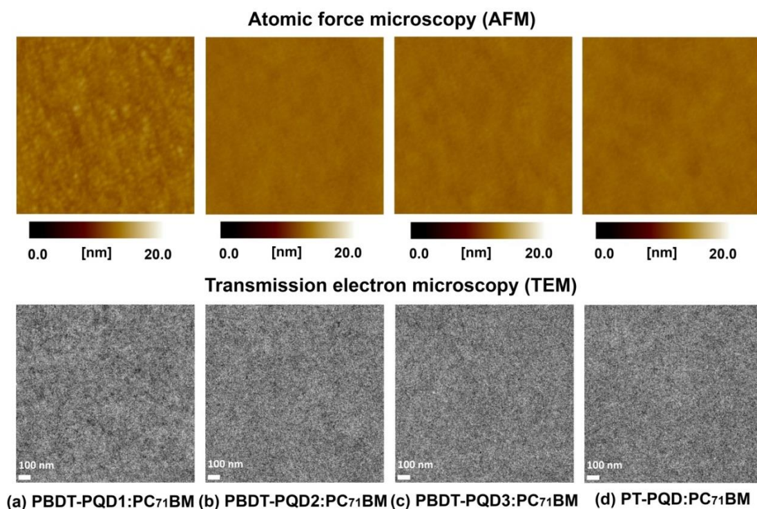
Fig. 5 AFM topography ( 2 \times 2 \mu\text{m}^2 ) and TEM bright field images of the optimized polymer:PC 71 BM
