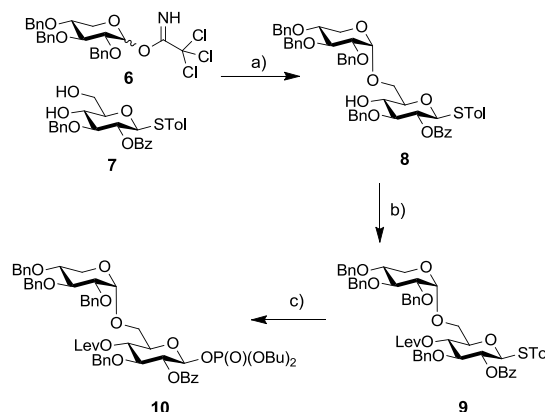
Scheme 2: Synthesis of disaccharide BB 10 . Reagents and conditions: a) TMSOTf, CH_2Cl_2 , -78^\circ C \rightarrow -10^\circ C , 39%; b) LevOH, DIC, DMAP, CH_2Cl_2 , 84%; c) HOP(O)(OBu) 2 , NIS, TMSOH, CH_2Cl_2 , 0^\circ C , 57%.
