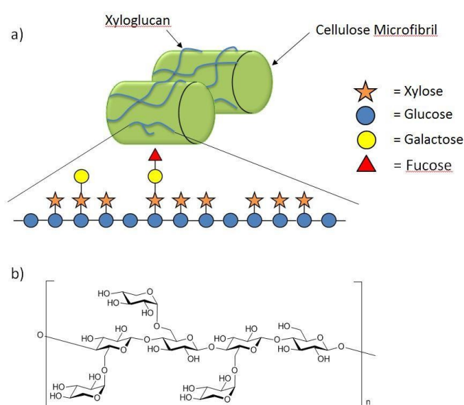
Figure 1: a) The hemicellulose xyloglucan interconnects cellulose microfibrils through hydrogen bonding; b) XXXG-type of XG oligosaccharides.
