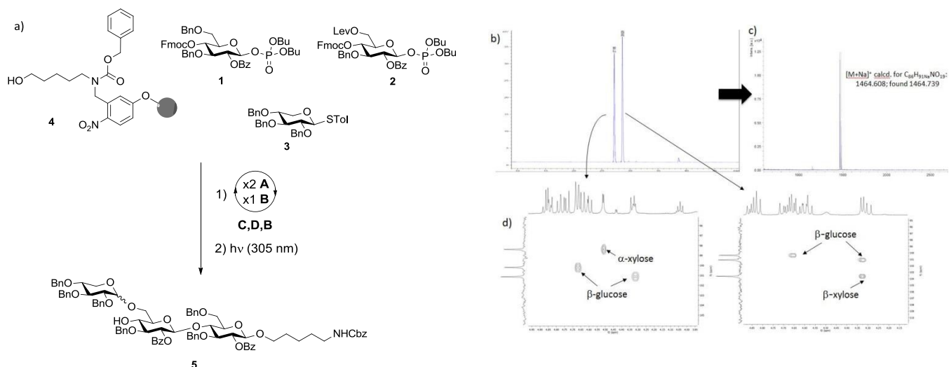
Scheme 1: a) Automated glycan assembly of trisaccharide 5 . Reagents and conditions: 2 x 3.7 equiv. BB 1 or BB 2 , TMSOTf, CH_2Cl_2 , -30^\circ C (5 min) or -35^\circ C (5 min) \rightarrow -15^\circ C (30 min) (Module A); 3 cycles of 20% Et 3 N in DMF, 25^\circ C (5 min) (Module B); N 2 H 4 ·OAc (155 mM) in pyridine/AcOH/H 2 O 4:1:0.25, 25^\circ C (30 min) (Module C); Module D: 2 x 3.7 equiv. BB 3 NIS/TfOH, CH_2Cl_2 /dioxane 2:1, -55^\circ C (5 min) \rightarrow -35^\circ C (40 min) (Module D); b) HPLC-chromatogram of the crude fully protected trisaccharide mixture; c) MALDI-TOF analysis after separation of the diastereomers by preparative HPLC; d) HSQC of the anomeric region of the two isolated stereoisomers.
