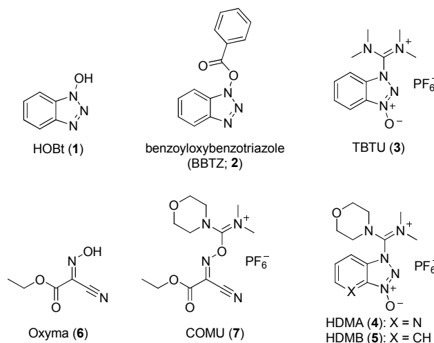
Figure 1. Benzotriazole- and Oxyma-based reagents.
