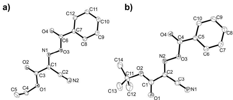
Figure 2. ORTEP representations of the molecular structures of benzoylated oximes a) 13 and b) 14 , determined by single-crystal X-ray crystallography. Ellipsoids are at the 50% probability level.
