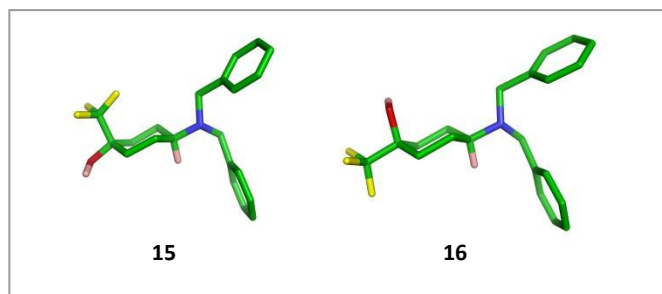
Figure 5. X-Ray crystal structure of 15 and 16
