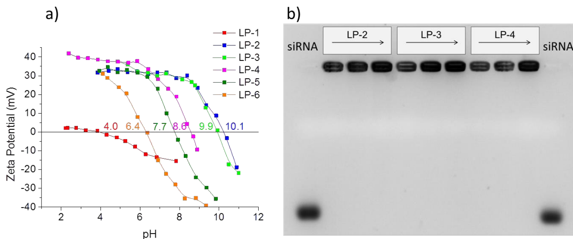
Figure 3: (a) Zeta potential measurements of LP-MSN with varying surface functionalization, (b) gel electrophoresis measurements with samples LP-2, LP-3 and LP-4 loaded with either 2.5, 6.6, or 12 \mu\text{g} siRNA/mg MSN (increasing concentration from left to right).
