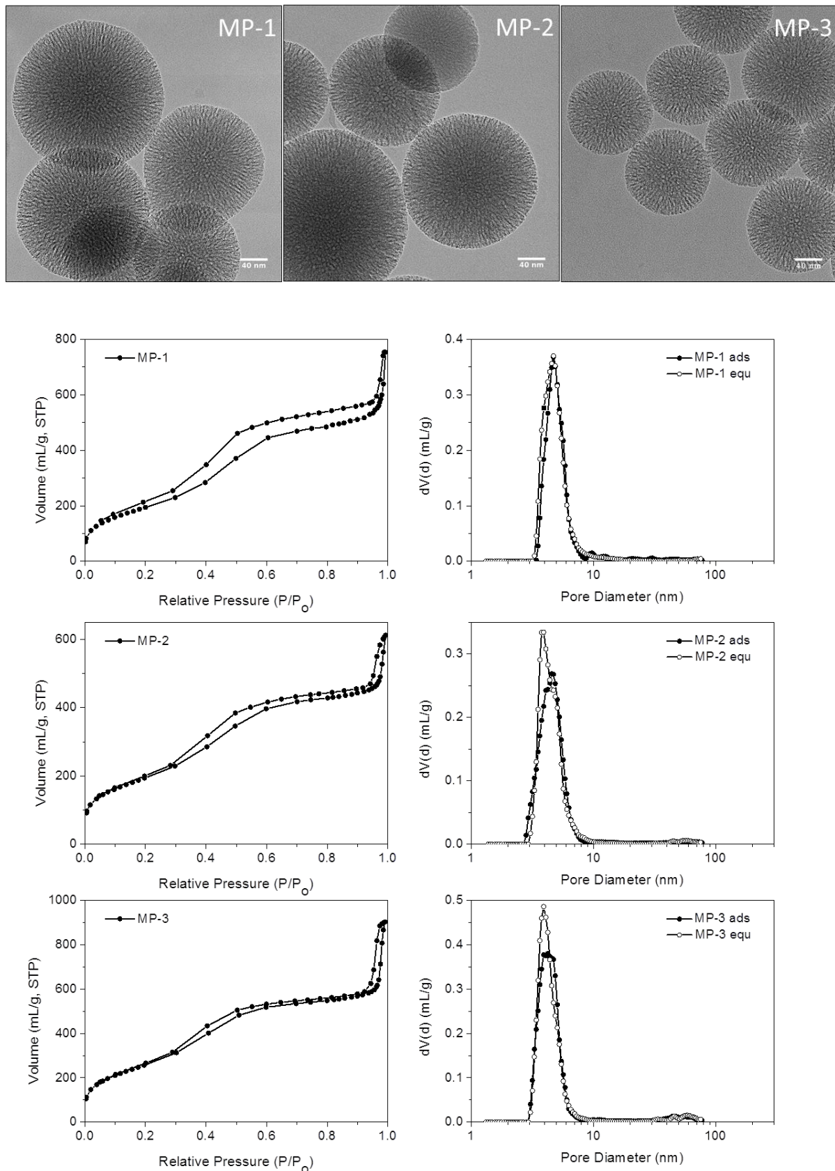
Figure 2: Transmission electron micrographs of core-shell samples MP-1 to MP-3 and the corresponding nitrogen sorption isotherms with pore-size distribution curves derived from the NLDFT equilibrium kernel for cylindrical pores (the NLDFT adsorption branch model and NLDFT equilibrium model superimposed).
