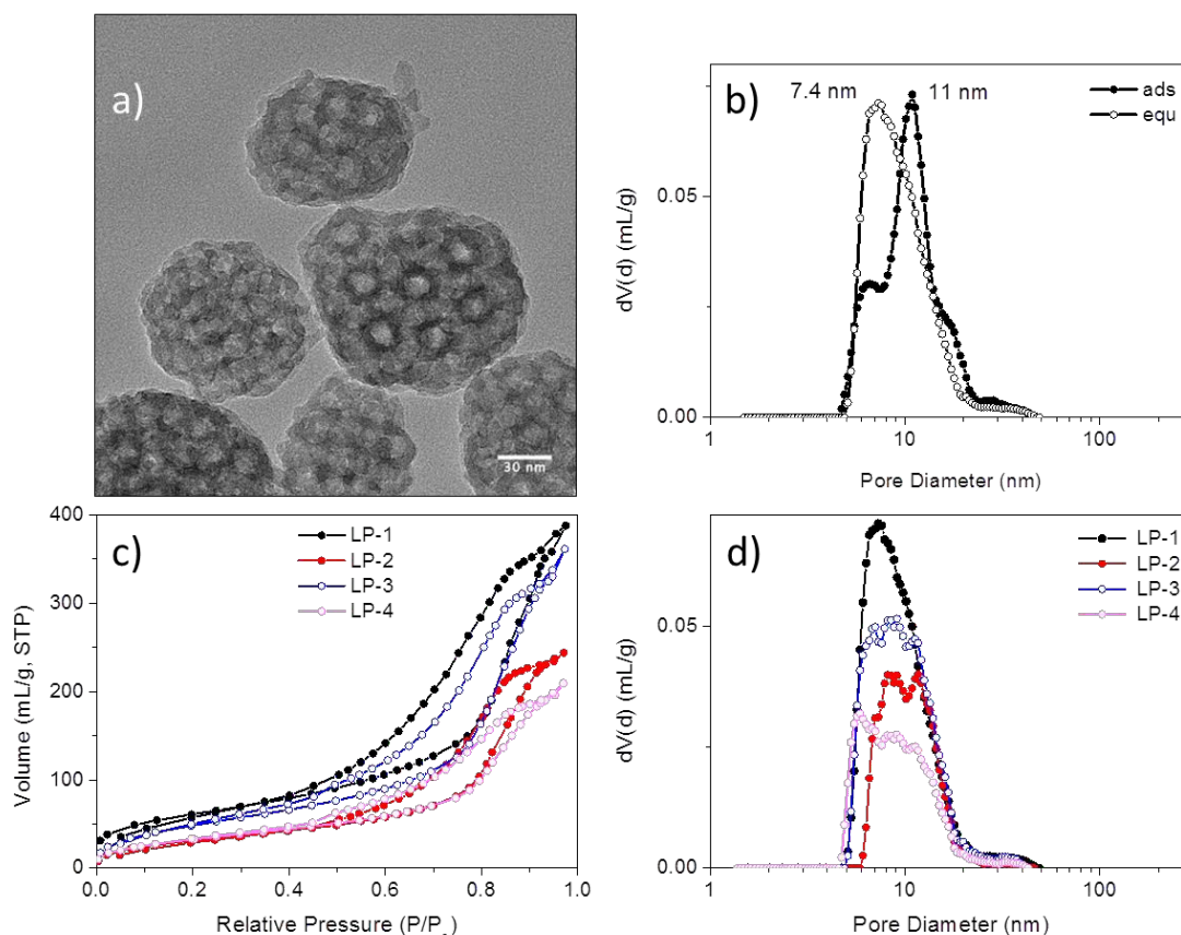
Figure 1: Characterization of large-pore silica nanoparticles (LP-MSN). a) Transmission electron micrograph, b) pore-size distribution of sample LP-1 derived from the NLDFT adsorption branch model and NLDFT equilibrium model of the respective nitrogen sorption isotherm, c) nitrogen sorption isotherms derived from parent siliceous sample LP-1 and samples LP-2 to LP-4 after grafting of different amounts of PhTES and APTES (see Table 1), and d) corresponding pore-size distributions derived from the NLDFT equilibrium kernel for cylindrical pores.
