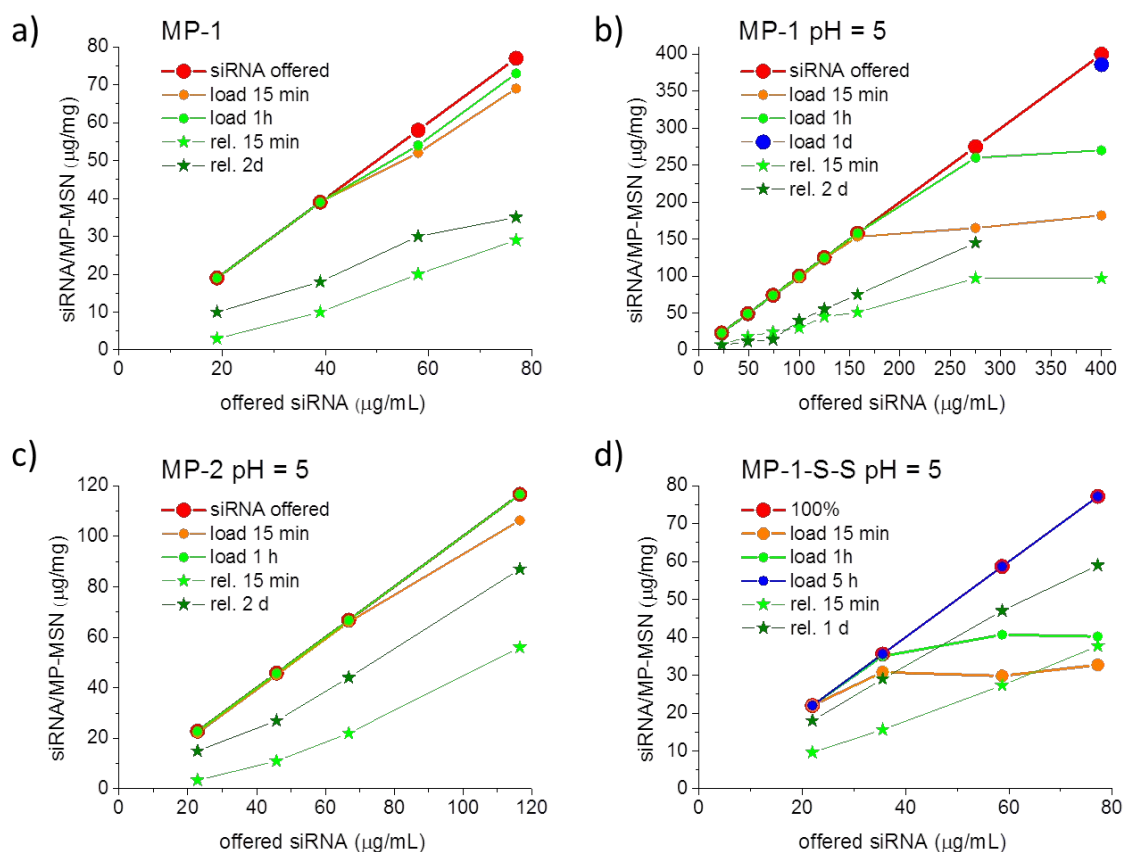
Figure 4: kinetic development of siRNA uptake and release with stellate MP-MSN. Aliquots of 100 µg of MSN were exposed to 100 µL of siRNA solutions with increasing concentrations. (a) Uptake in MP-1 from water, and (b-d) uptake from MES buffer at pH = 5 into samples (b) MP-1, (c) MP-2, and (d) MP-1-S-S. Release experiments were performed in 100 µL PBS buffer at pH = 7.4 in all samples. The red curve indicates the offered siRNA amount, and orange and green dots indicate the adsorbed siRNA after 15 minutes and 1 h, respectively. Light green and dark green stars are the cumulatively released amounts of RNA after 1 h and 2 days, respectively.
