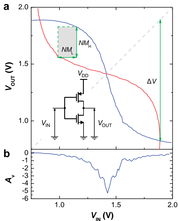
Fig. 3 Voltage gain and NMs in short-gated graphene inverters at V_{DD} = 2.5\ \text{V} . (a) Static voltage transfer characteristic (blue) and its mirrored reflection (red) of an inverter with L = 0.8\ \mu\text{m} , W = 5\ \mu\text{m} , and L_a = 250\ \text{nm} . The output voltage swing \Delta V = 1\ \text{V} . The low ( NM_L = 0.17\ \text{V} ) and high ( NM_H = 0.27\ \text{V} ) static NMs are determined by the rectangle of the largest area that can be drawn inside the loops. The actual static NM is smaller of the two, i.e., NM = NM_L . Inset: schematic of an inverter. (b) Low-frequency voltage gain obtained as the first derivative of the static transfer curve shown in (a).
