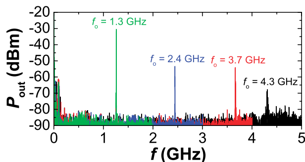
Fig. 4 The power spectra of the output signals with the highest oscillation frequency for each of the investigated RO layouts (coded in the same colors as in Figure 2). The finite capacitance of the output pad results in signal attenuation which is stronger at higher frequencies, as described in the main text. In the fastest two RO layouts (red and black curves) the surface area of the output pad was reduced from (150 \mu\text{m})^2 to (80 \mu\text{m})^2 because of which the attenuation of the signal in red is almost the same as for the signal in blue. A pure sine wave with a voltage swing \Delta V = 1 V (as in Figure 3) has a power level of 4 dBm.
