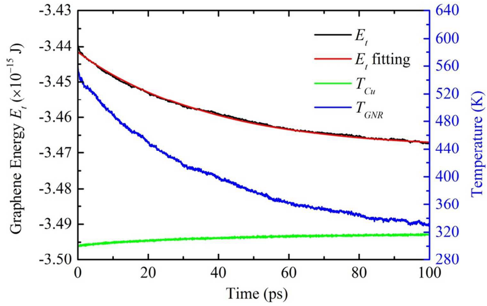
Figure 2. Energy fitting of the supported graphene system for thermal resistance calculations.
