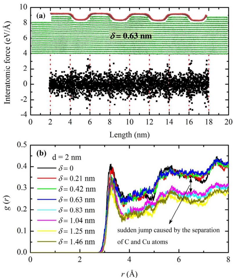
Figure 6. (a) Interatomic force distributions in the GNR system at out-of-plane ( z ) direction for d = 2 nm, \delta = 0.63 nm hybrid system. Significant attractive and repulsive forces are detected in the suspended and supported regions, respectively. (b) Radial distribution function between GNR and copper for different \delta cases at d = 2 nm. A sudden separation between GNR and copper atoms is observed when \delta increases from 0.63 nm to 0.83 nm, corresponding to the thermal contact resistance increase shown in Fig. 5(a).
