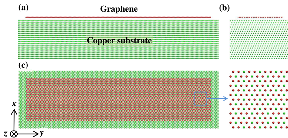
Figure 1. Atomic configurations of the graphene-copper hybrid system. The GNR honeycomb lattice (red) is positioned to match the triangular lattice of Cu (111) surface (green) with one carbon atom on top of a Cu atom and the second carbon on a hollow site.
