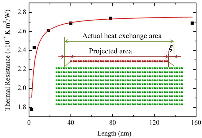
Figure 3. Thermal resistance variations with GNR length. Width of the supported GNR is 4.2 nm and flat surface copper substrate is used in all calculations.
