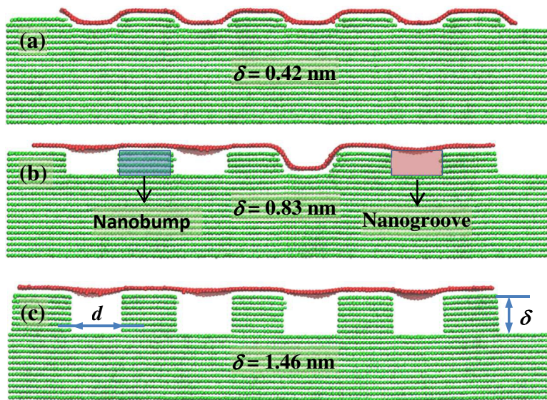
Figure 4. Atomic structures at steady state for d = 2 nm cases with \delta = 0.42, 0.83 and 1.46 nm. (a) The suspended GNR regions are bent to fit the surface nanogrooves on the Cu substrate. (b) GNR is partially in contact with Cu in suspended regions. (c) All suspended areas of GNR are separated from the Cu substrate.
