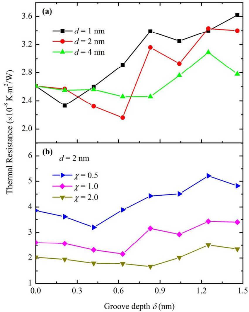
Figure 5. (a) Thermal contact resistance variations with nanogroove width and depth. (b) Effects of the interaction strength ( \chi ) on the interfacial thermal resistances.
