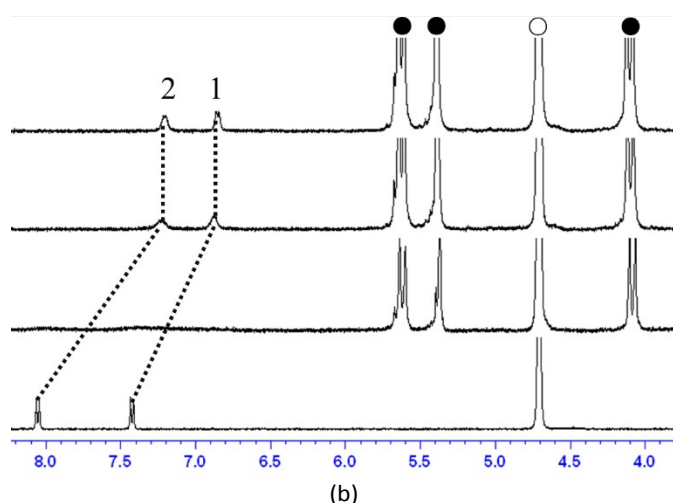
Fig. 2. (a) The ^1\text{H} NMR titration spectra of BZC (1 mM) in the presence of increasing amounts (0, 0.5, 1.2, 2.2 3.1 equiv.) of CB[7] at pD = 2; (b) The ^1\text{H} NMR titration spectra of PABA (1 mM) in the presence of increasing amounts (0, 0.7, 1.5, 3.0 equiv.) of CB[7] at pD = 2. The peaks labelled as (●) and (○) are CB[7] and HOD protons, respectively.
