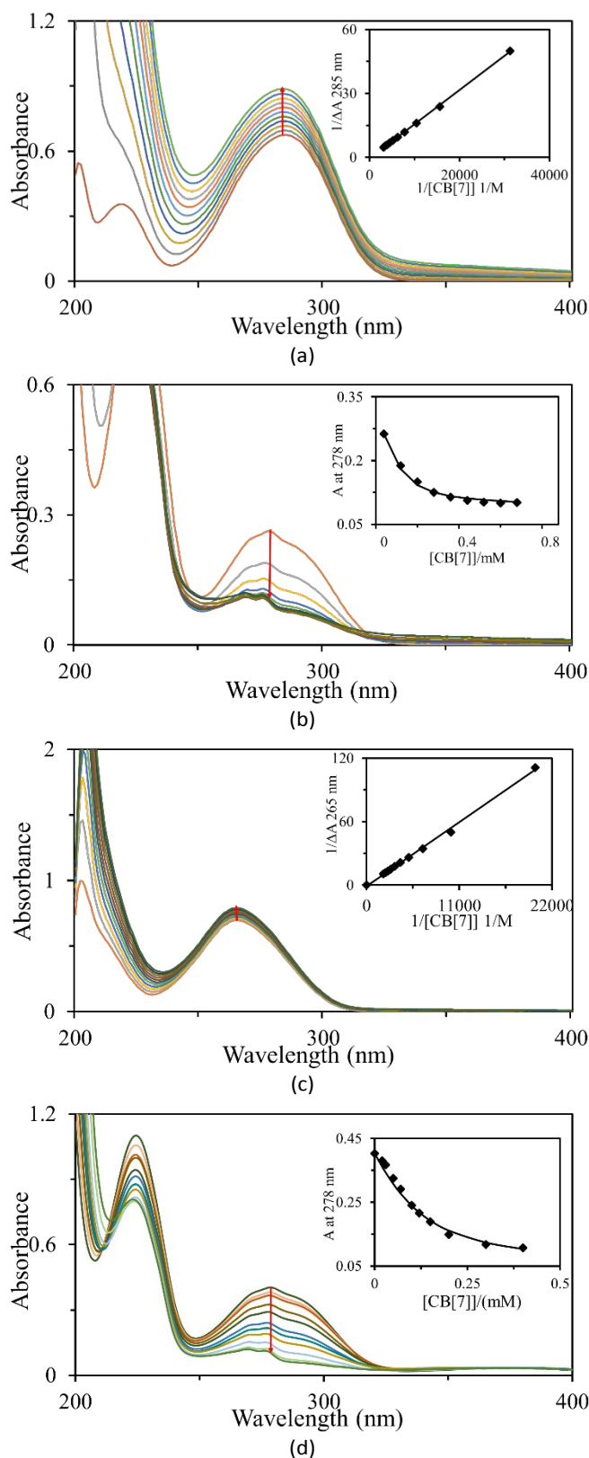
Fig. 5. UV-vis titration of BZC (0.04 mM) in PBS buffer (pH = 7.4) (a), and BZC (0.08 mM) in HCl solutions (pH = 2) (b), with increasing amounts of CB[7]. UV-vis titration of PABA (0.05 mM) in PBS buffer (pH = 7.4) (c), and PABA (0.10 mM) in HCl solution (pH = 2) (d), with increasing amounts of CB[7]. The insets in the four figures show the best fit between experimental points and a 1:1 binding model affording a binding constant K_a of \sim 300 \text{ M}^{-1} , 2.2 \pm 0.2 \times 10^4 \text{ M}^{-1} , 200 \text{ M}^{-1} and 1.5 \pm 0.2 \times 10^4 \text{ M}^{-1} respectively.
