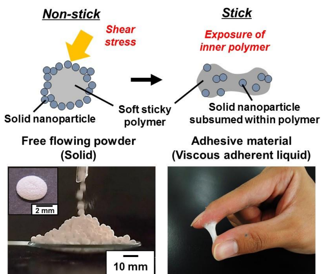
Figure 1. Schematic representation of pressure-sensitive adhesive (PSA) powder consisting of particles with a soft sticky polymer core and a solid nanoparticle shell morphology. After application of shear stress, adhesive nature appeared because of outflow of the inner soft polymer. Optical photographs of such PSA materials are also shown. The PSA shows no adhesion in its original form and flows freely like a powder. (Inset shows single PSA particle.) Only after application of shear stress, it acts as an adhesive.
