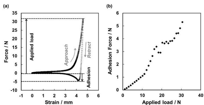
Figure 3. (a) Example of force vs. strain curves obtained for PSA liquid marble, from which the dependence of adhesion on load was obtained: □, Approach; ○, Retract. (b) Dependence of adhesion on applied load.
