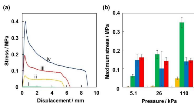
Figure 4. (a) Stress-displacement tack curves obtained for PSA liquid marble: (i) before and (ii-iv) after application of shear stress. Pressure applied to PSA liquid marbles: (i, ii) 5.1, (iii) 26 and (iv) 110 kPa. (b) Relationship between pressure applied to PSA materials and maximum stress in tack measurement. Samples: Liquid marble PSA (yellow bar) before and (green bar) after application of shear stress, (blue bar) PBA latex film with a thickness of 45 μm and (red bar) commercially available PSA tape (Scotch® Magic™ Tape 810)
