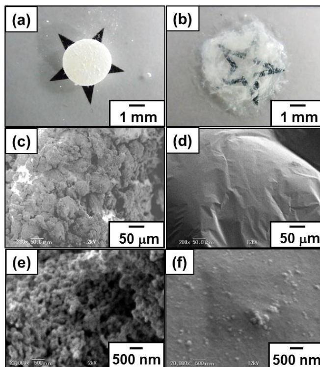
Figure 2. (a, b) Digital photographs and (c-f) SEM images of a particle with a soft adhesive PBA core and a CaCO 3 hard nanoparticle shell morphology (a, c, e) before and (b, d, f) after application of shear stress.
