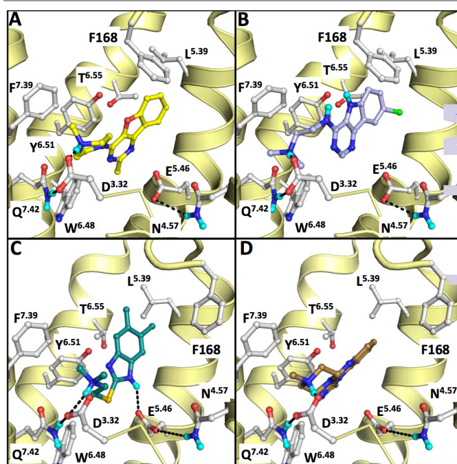
Fig. 7 Binding modes of the validated hits VUF13686 ( 9b , yellow, panel A) and VUF13694 ( 10b , purple, B) in the \beta_2 R-based H 4 R model, compared to the binding modes of VUF13848 ( 12 , darkgreen, C), and VUF13860 ( 13 , brown, D) in the H 1 R-based H 4 R model. Rendering is similar to Fig. 2.
