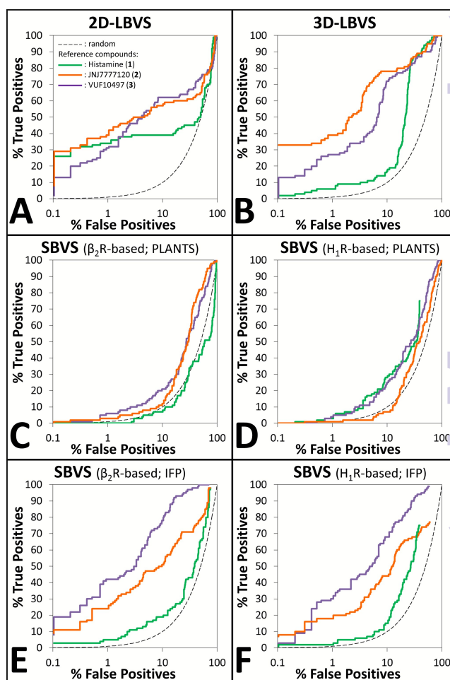
Fig. 3 Graphs of % true positives (fragment-like H_4 R ligands) vs % false positive (fragments that do not bind H_4 R) in the ranked database resulted from 2D-LBVS (A), 3D-LBVS (B), \beta_2 R-based SBVS ranked by PLANTS ChemPLP score (C), H_1 R-based SBVS ranked by PLANTS ChemPLP score (D), \beta_2 R-based SBVS re-ranked by Tc-IFP score (E), and H_1 R-based SBVS re-ranked by Tc-IFP score (F) based on histamine ( 1 , green), JNJ-777120 ( 2 , orange), and VUF10497 ( 3 , purple) reference ligands (A-B) and ligand- H_4 R IFPs (C-F).
