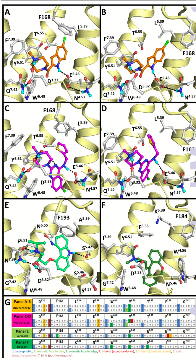
Fig. 2 Comparison of \beta_2 R-carazolol (light green) crystal structure 64 (E) based H 4 R models (A, C) and H 1 R-doxepin (dark green) crystal structure (F) based H 4 R models 45 (B, D). H 4 R models are constructed with JNJ7777120 (2, orange carbon atoms, A and B) and VUF10497 (3, magenta, C and D). Protein-ligand interaction fingerprints (IFPs) of the binding modes in A-F are presented in G. The backbone of TM helices 4, 5, and 6, and part of TM3 is shown as ribbon (the top of the helix is not shown for clarity). Important binding residues identified previously 4, 55, 56, 59, 61, 82 are depicted in grey.
