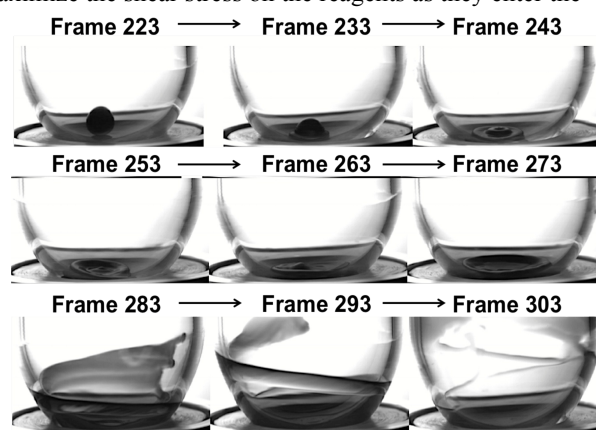
Fig. 2. High-speed images of a droplet of water colliding with the hemisphere of a 17.7 mm internal diameter dry borosilicate glass VFD sample tube. The tube is orientated at 90° relative to the horizontal position and rotating at 5250 rpm. Frame 253-263 - the thickening of the drop edge forming after initial impact. Frame 273 - the instability of the drop edge, leading to viscous fingering instability, frame 283-303. To generate these photographs a droplet of water mixed with blue dye was dropped from a height of 2.0 cm into the hemisphere of a sample tube at a 90° tilt angle. A high-speed camera was operating at 5400 fps, shown are non-consecutive frames.
