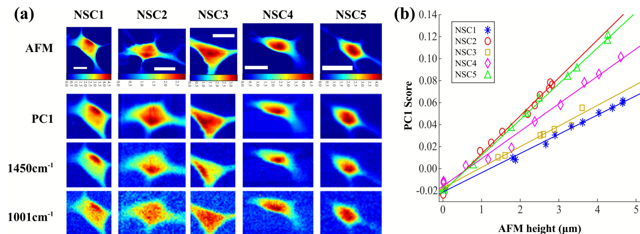
Figure 5. Cell normalization comparison. (a) shows AFM maps (scale bar 20 μm) for five different NSCs, with corresponding maps from Raman data, based on PC1 scores, and normalization by peak area for 1450 cm -1 and 1001 cm -1 peaks. (b) Correlation of AFM height with co-localized PC1 scores.
