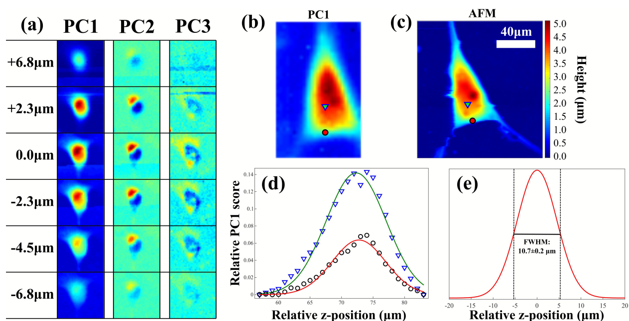
Figure 6. (a) Raman z-profiling images. (b) PC1 map and (c) AFM for an NSC for which 25 line scans at different z -positions were obtained. (d) shows the variation in the value of the PC1 score as the sampling z -position is varied at two locations on the cell of different thickness (indicated in (c) and (d)). Several PC1 z -profiles were fitted to a Gaussian function, matched to a top-hat function of width given by the corresponding AFM height, and de-convolved to obtain an estimate for the PSF_z . (e) shows the resulting average PSF_z measured from 13 de-convolution measurements.
