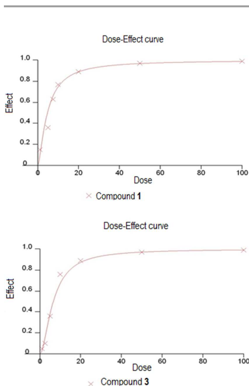
Figure 2 Dose/Effect curve for compound 1 and 3 against HCT116 cells (after 48 h of incubation) calculated by fitting the data points with a sigmoidal curve using Calcsyn software
