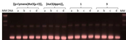
Figure 3 Electrophoresis mobility shift assays for [\text{Ru}(\text{p-cymene})\text{Cl}(\mu\text{-Cl})_2] , [\text{AuCl}(\mu\text{-dppm})_2] and compounds 1 and 3 (see Experimental Section for details). DNA refers to untreated plasmid pBR322. Lanes a, b, c, and d correspond to metal/DNA ratios of 0.25, 0.5, 1.0, and 2.0, respectively
