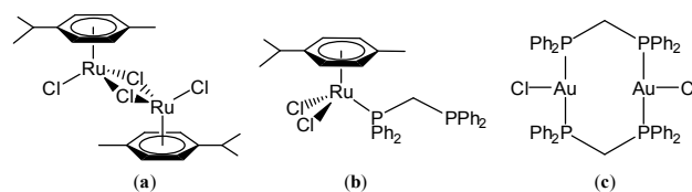
Chart 2 Ru and Au reference compounds; (a) [\text{Ru}(\text{p-cymene})\text{Cl}(\mu\text{-Cl})]_2 26 (b) [\text{Ru}(\text{p-cymene})\text{Cl}_2(\eta^1\text{-dppm})]_2 28,29 (c) [(\text{AuCl}(\mu\text{-dppm}))]_2 30
