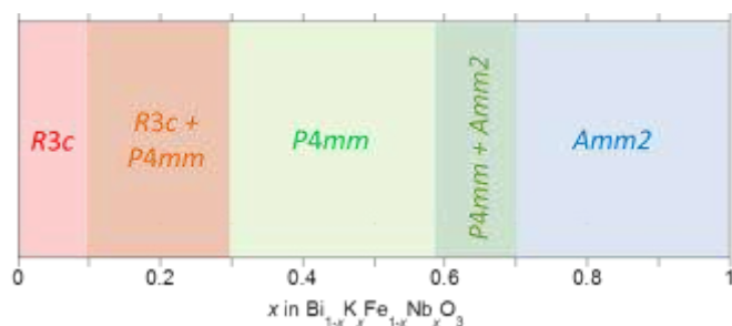
Figure 4: Proposed phase diagram for \text{Bi}_{1-x}\text{K}_x\text{Fe}_{1-x}\text{Nb}_x\text{O}_3 materials based on powder diffraction studies.
