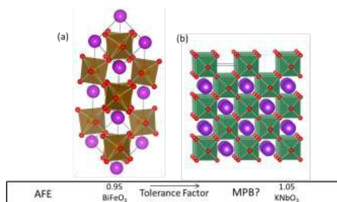
Figure 1: Schematic representation of (a) BiFeO 3 in the hexagonal setting of the R3c space group where the brown squares represent the FeO 6 octahedra, the purple spheres represent the Bi 3+ ions and the red spheres represent the oxygen ions respectively, (b) orthorhombic Amm2 , KNbO 3 where the green squares represent the NbO 6 octahedra, the purple spheres represent the K + ions and the red spheres represent the oxygen ions respectively and phase diagram showing the relationship with tolerance factor, t , with the PZT phase diagram showing the regions of antiferroelectric (AFE) behaviour and the potential for morphotropic phase boundaries (MPB) with decreasing and increasing t respectively.
