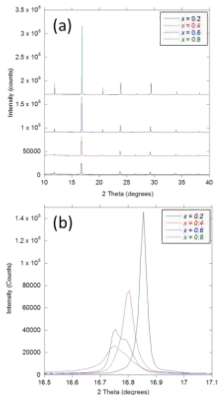
Figure 2: (a) and (b) Synchrotron diffraction patterns collected for \text{Bi}_{1-x}\text{K}_x\text{Fe}_{1-x}\text{Nb}_x\text{O}_3 materials with x = 0.2, 0.4, 0.6 and 0.8 showing the shift in peak position and thus lattice parameters with increasing values of x .
