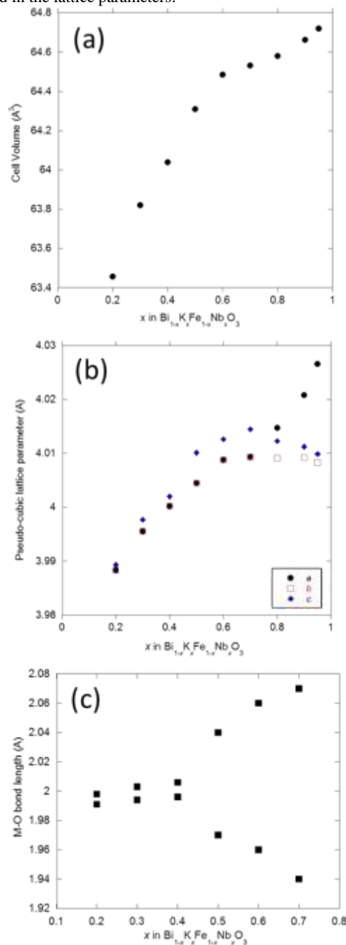
Figure 3: Neutron powder diffraction results for (a) Pseudo-cubic cell volume, (b) pseudo-cubic lattice parameters and (c) apical Fe/Nb-O bond length as a function of x in \text{Bi}_{1-x}\text{K}_x\text{Fe}_{1-x}\text{Nb}_x\text{O}_3 materials. (Note: error bars are smaller than the symbol size. Error values are given in the ESI † )
