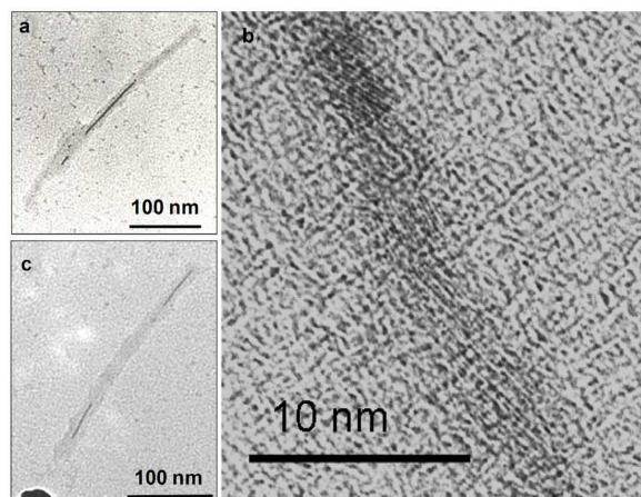
Figure 5. (a) TEM micrograph of CoFe alloy NWs within the channel of a TMV particle (dark gray). The black line in the center corresponds to an alloy wire of \sim 3 nm in diameter and approximately 100 nm in length. In the lower part of the same virion a second small nanowire ( \sim 10 nm long) is located. Another short virion ( \sim 100 nm long) is attached to the lower portion of the metallized virion. (b) High-resolution TEM image of a CoFe nanowire inside TMV. Crystal planes of various orientation and spacing are visible, all compatible with various orientations of CoFe. The image was calibrated by imaging Au particles at the same magnification. (c) TEM image of two short CoFe(Ni) wires located in a single virion cavity. The dark nodule at the bottom part stems from bulk deposition of the alloy. Reprinted with permission from ref.117. Copyright © 2012, Institute of Physics.
