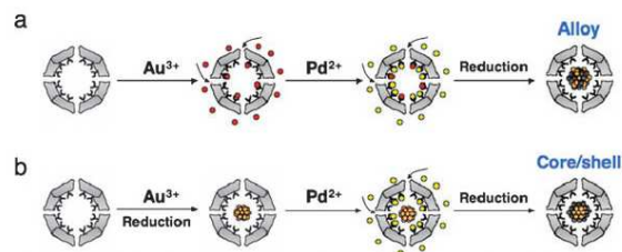
Figure 11. Schematic illustrations of the two different synthesis methods of Au/Pd NPs in apo-Fr solution. (a) the synthesis of Au/Pd alloy structure; (b) the synthesis of Au@Pd core-shell structure. Au(III), Au(0), Pd(II) and Pd(0) atoms are colored red, orange, yellow and brown, respectively. Reprinted with permission from ref.209. Copyright © 2014, Royal Society of Chemistry.
