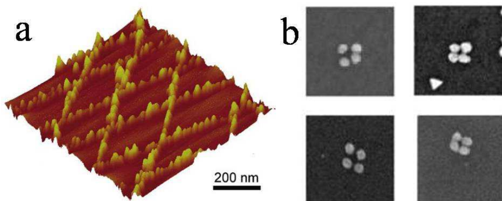
Figure 17. (a) AFM image of 2D array of Pd NWs (b) SEM images of four Au NPs assembling on per origami. Reprinted with permission from ref. 255 and 260. Copyright © 2003 and 2014, American Chemical Society, respectively.
