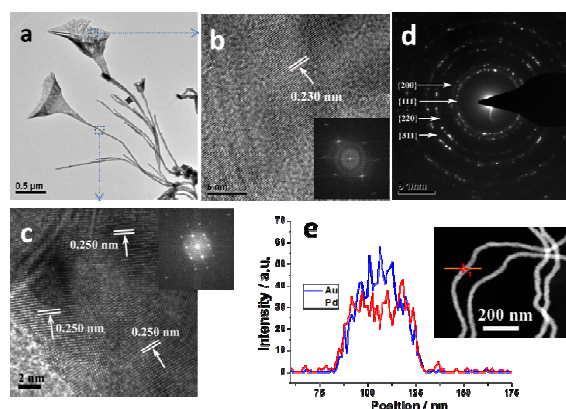
Figure 4. (a) TEM image of AuPd NFs, (b) HRTEM image of blossom, (c) HRTEM image of pedicel, (d) SAED pattern of AuPd NFs, and (e) EDX line profiles of an individual AuPd nanowire (pedicel) corresponding to the framed part (dash) in (a). The insets indicate the corresponding fast Fourier transform (FFT) pattern. Reprinted with permission from ref.106. Copyright © 2014, Royal Society of Chemistry.
