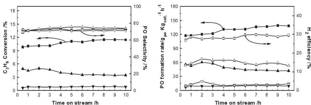
Figure 19. Epoxidation of propylene over Au/TS-1; ■□: 0.5Au/TS-1(35)-IL, ▲△: 0.5Au/TS-1(35)-pH, ▼▽: 0.5Au/TS-1(35). Reprinted with permission from ref.306. Copyright © 2011, Academic Press Inc Elsevier Science.
