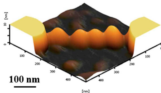
Figure 16. AFM image of Au NP chain between the two electrodes. Reprinted with permission from ref. 235. Copyright © 2010, Institute of Electrical and Electronics Engineers.
