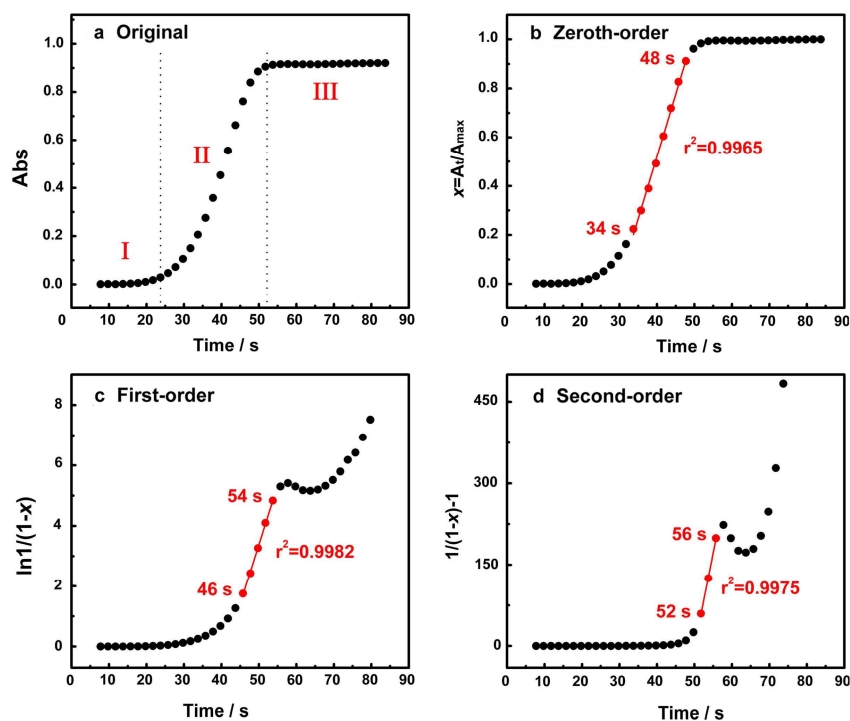
Figure 10. (a) Typical sigmoidal Abs- t profile and its responding x - t profiles obtained by treating the Abs- t profile with (b) zeroth-order, (c) first-order and (d) second-order rate laws for Au NPs synthesized by L-ascorbic acid reduction. Reprinted with permission from ref.198. Copyright © 2013, Academic Press Inc Elsevier Science.
