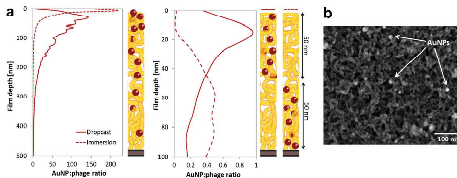
Figure 7. Tight spatial distribution control of the bacteriophage-mediated incorporation of Au NPs. A) XPS depth profiling analysis of the Au distribution as a function of the film depth, converted to NP to phage ratio for different film architectures. The top panel shows the distribution for NPs infiltrated post-assembly, while the bottom panel shows films that were assembled with phage-NP complexes. B) SEM image of a phage film infiltrated with Au NPs, and coated with titania. Bright circles are imaged Au NPs dispersed within the nanowire mesh. Reprinted with permission from ref.146. Copyright © 2014 Wiley-VCH Verlag GmbH & Co. KGaA, Weinheim.
