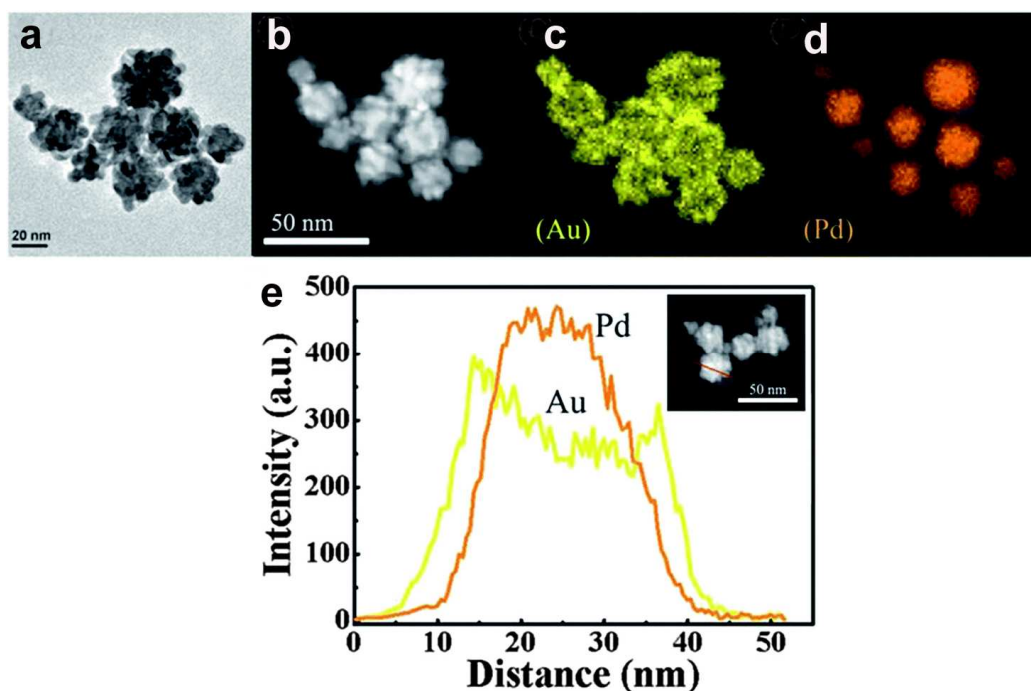
Figure 9. (A) TEM image and (B) high-magnification STEM image of the flower-shaped AuPd NPs with an initial AuPd ratio of 1:1; energy dispersive X-ray (EDX) elemental maps of (C) Au and (D) Pd concentrations in the NPs and (E) the distribution of the Au and Pd components along the cross-sectional line profiles of a single AuPd NP. Reprinted with permission from ref.192. Copyright © 2014, Royal Society of Chemistry.
