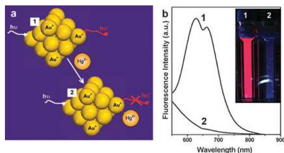
Figure 24. (a) Schematic illustration of the Hg(II) sensing mechanism based on BSA-templated Au NCs. (b) Photoemission spectra and (inset) photographs of Au NCs under UV light in the absence and presence of Hg(II) ions. Reprinted with permission from ref. 328. Copyright © 2010, Royal Society of Chemistry.
