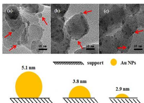
Figure 21. TEM images of Au/TiO 2 catalysts with different Au NPs sizes, (a) 5.1 ± 0.9 nm, (b) 3.8 ± 0.6 nm (c) 2.9 ± 0.6 nm. Reprinted with permission from ref. 313. Copyright © 2014, American Chemical Society.
