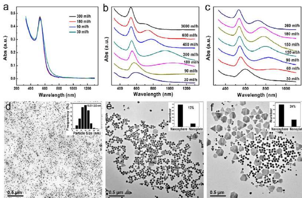
Figure 8. (a–c) UV–vis–NIR spectra of Au sols prepared by addition modes (a) A, (b) B, and (c) C. (d–f) Representative TEM images of the Au NPs prepared by (d) mode A at an addition rate of 300 mL/h, (e) mode B at an addition rate of 450 mL/h, and (f) mode C at an addition rate of 90 mL/h. The reaction temperature and pH for all samples were 90 °C and 3.41, respectively. Three different mixing modes were adopted: mode A, involving the addition of Au precursor to C. Platycladi extract; mode B, involving an inverted addition of the extract to the Au precursor; and mode C, involving the simultaneous injection of the two feed solutions ( C. Platycladi extract and Au precursor) with equal addition rates. Reprinted with permission from ref.180. Copyright © 2012, American Chemical Society.
