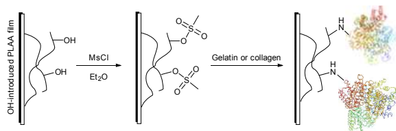
Fig. 13. Schematic representation of the reaction protocol for immobilisation of protein of PLLA film surfaces describe by Ma et al. 181
