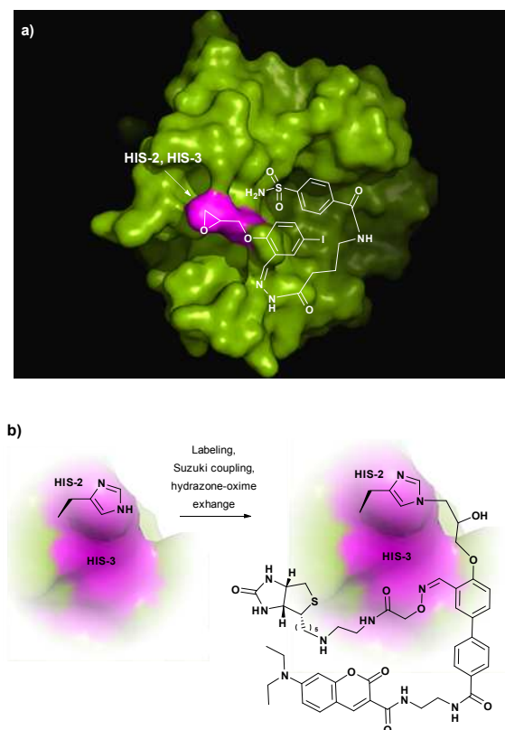
Fig. 49. Affinity labelling, hydrazone-oxime-exchange reaction, and Suzuki coupling reaction on the surface of bCA (pdb: 1V9E) described by Hamachi and collaborators. 463 a) Principal structural fragments of the probe: a benzenesulfonamide ligand responsible for targeting bCA; an electrophilic epoxide responsible for reactivity towards vicinal His residues HIS-2 and HIS-3 (shown in magenta), cleavable hydrazone bond, responsible for the recovering of the enzymatic activity; an iodoaryl moiety, utilised for the further bioorthogonal transformation via Suzuki coupling. b) Dual labelling of bCA in situ : fluorescent labelling of the HIS-2 or HIS-3 alkylated intermediate by Suzuki coupling with a coumarine derivative, followed by biotinylation by hydrazone/oxime-exchange.
