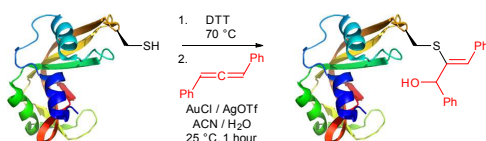
Fig. 40. Cysteine modification of RNase A (pdb: 7RSA) via gold-mediated coupling with allenes. 420
