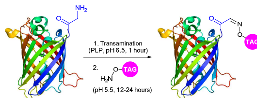
Fig. 69. Site-specific N -terminal labelling of EGFP (pdb: 2Y0G). Proteins possessing N -terminal carbonyl groups obtained by in the first step PLP-mediated transamination were labelled with hydroxylamine probes in the second step. 601
