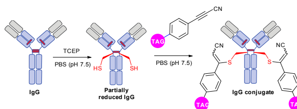
Fig. 42. Preparation of IgG (pdb: 1IGY, red sticks represent four interchain disulfide bonds) conjugates with increased plasma stability using 3-arylpropionitriles (APN) described by Wagner and collaborators. 429
