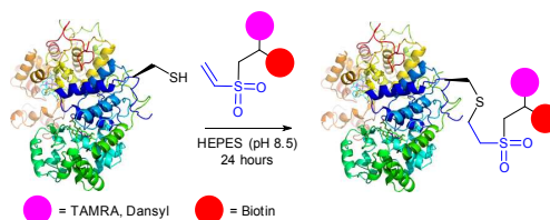
Fig. 25. Bifunctional labelling of horseradish peroxidase (HRP, pdb: 2ATJ) with vinyl sulfone-functionalised tags described by Morales-Sanfrutos et al. 330
