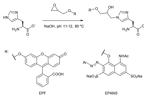
Fig. 48. Fluorescent probes, described by Li et al. for selective labelling of histidine. 459,460
