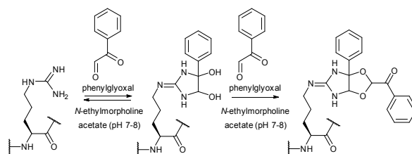
Fig. 61. Reaction of phenylglyoxal with arginine moiety (reaction condition: 0.2M N -ethylmorpholine acetate buffer, pH 7-8).
