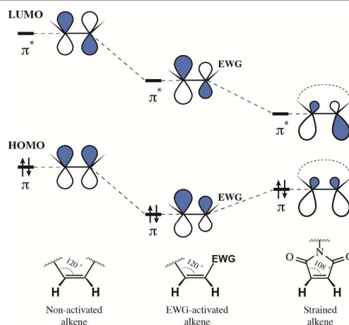
Fig. 21. Influence of an electron-withdrawing group (EWG) and cycle strain on the frontier orbitals of alkenes, \sigma -orbitals omitted (the form of the orbital is presented approximately, based on the publication of Merchan et al. 268 ). Decreasing the energy of LUMO (lowest unoccupied molecular orbital) results in higher reactivity of the electrophile towards nucleophiles. Although via different mechanisms, both EWG and strain of the cycle activate alkene for the attack by nucleophiles.
