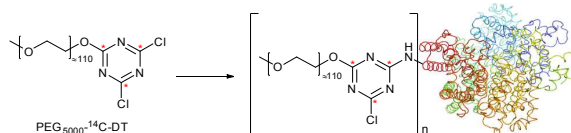
Fig. 17. Modification of BSA (pdb: 3V03) by PEG-[ 14 C]dichlorotriazine probe reported by Abuchowski and colleagues ( 14 C atoms are marked with red stars). 220
