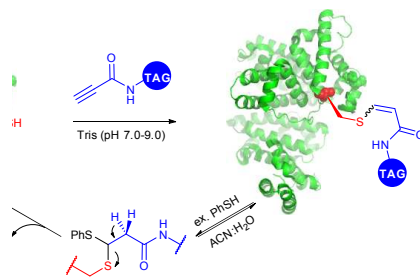
Fig. 41. Cleavable labelling of BSA (pdb: 3V03) with arylalkynone reagents elaborated by Che and associates. 417
