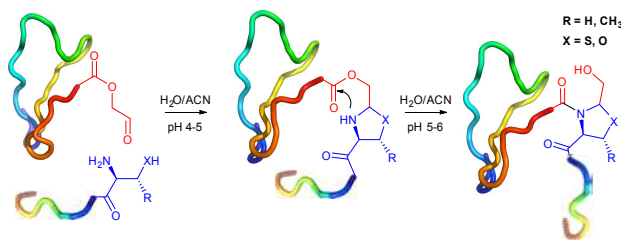
Fig. 73. General scheme of the ligation strategy proposed by Liu and Tam. 635 A model 50-residue peptide was obtained in good yield in ligation reaction between a 32-mer peptide VVSHFNDPCDSHTQFEFHGTCTRFLVQEDKPAR containing C -terminal aldehyde function and a 17-mer peptide CHSGYVGARC(Ac-m)EHADLLA containing N -terminal cysteine; in the case of Thr- and Ser-peptides, the reaction was moderately efficient. The peptides structures were simulated using RaptorX web server. 447
