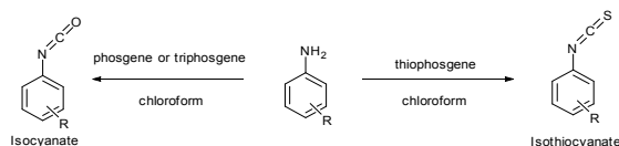
Fig. 3. Synthesis isothiocyanates and isocyanates from the corresponding aromatic amines. 36
