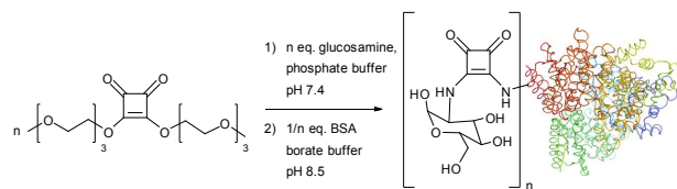
Fig. 16. One-pot, two-step squaric acid diester mediated glycosylation of BSA (pdb: 3V03) described by Wurm et al. 217 Up to 22 lysine residues of the 59 present in BSA (30-35 are available for post-modification) could be glycosylated with 25-fold excess of squaric diester and glucosamine in 12 hours.
