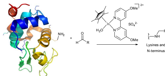
Fig. 11. Modification of lysozyme (pdb: 2LYZ) using reductive alkylation with water-stable iridium catalyst developed by McFarland and Francis. 161
