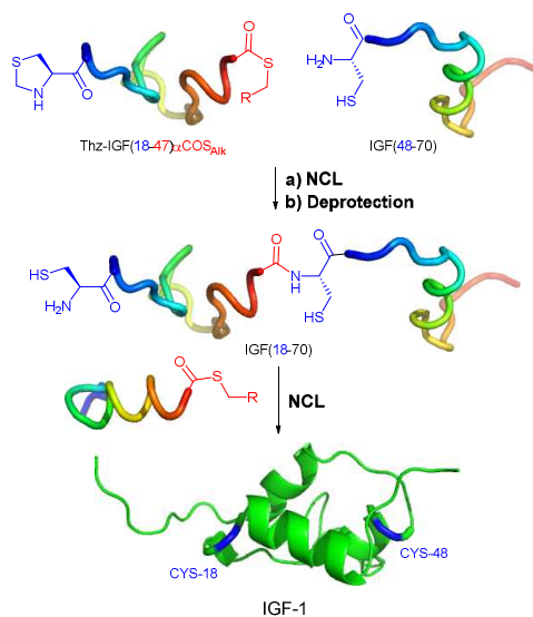
Fig. 79. Synthesis of insulin-like growth factor 1 (IGF-1) via sequential native chemical ligation described by Sohma et al. 672 The reversible protection of the \alpha -amino group of the central peptide fragment IGF(18-47) prevents its self-reaction with the \alpha -thioester moiety present in the same molecule. Thiazolidine protecting group can be easily removed by brief treatment with NH 2 OMeHCl at pH 4. NCL reaction condition used: PB (pH 6.7), 6M GndCl, 10 mM MPPA, 20 mM TCEP.
