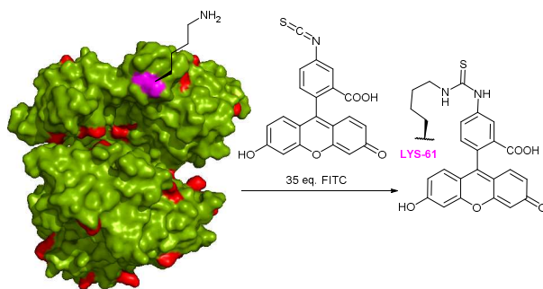
Fig. 5. Selective fluorescent labelling of LYS-61 residue (shown in magenta) of rabbit skeletal muscle G-actin (pdb: 2VYP) reported by Butnick. 43
