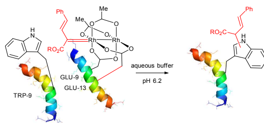
Fig. 46. Selective covalent labelling of TRP-9 residue of the peptide QEISALEKWISALEQEISALEK with its complementary dirhodium metallopeptide KISALQKQKESALEQKISALKQ described by Popp and Ball. 454 Rhodium cluster, chelated with two glutamate residues, is brought to a proximity of the reactive Trp residue by peptides coils self-assembling, resulting in selective peptide modification on TRP-9. Peptide structures were simulated using RaptorX web server. 447
