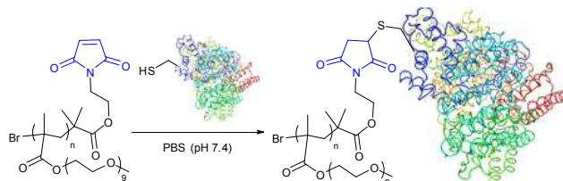
Fig. 22. Conjugation of maleimide-functional poly(PEGMA) to the only free CYS-34 residue of BSA (pdb: 3V03). 311
