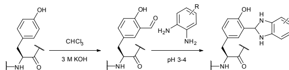
Fig. 54. Two-step tyrosine modification by selective formylation of tyrosyl residue at the ortho position of its phenolic moiety (reaction with chloroform in potassium hydroxide solution) and further derivatisation of the resulting aldehyde described by Kai et al. 493,494
