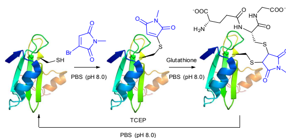
Fig. 23. Conjugate addition of L111C mutant of SH2 domain of Grb2 (wild-type pdb: 1JYU) to bromomaleimide followed by second addition of glutathione resulting in generation of the vicinal bis-cysteine adduct. 316
