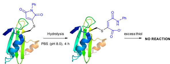
Fig. 24. “Switching off” the linker's reactivity for second thiol addition achieved by hydrolysis of the thiomaleimide linkage on L111C mutant of SH2 domain of Grb2 (wild-type pdb: 1JYU). 317
