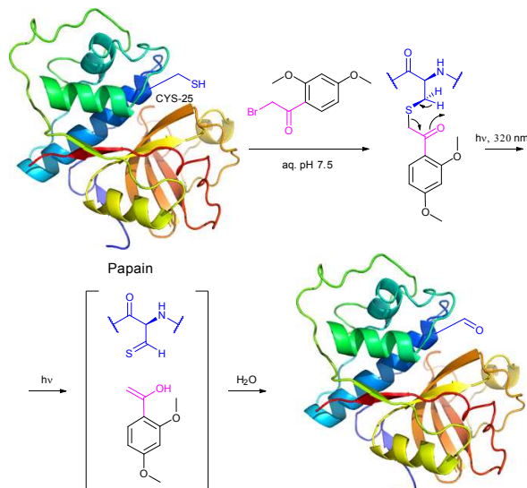
Fig. 20. Photolysis of CYS-25 residue located in papain's active site (pdb: 1PPN) after its labelling with 2-bromo-2',4'-dimethoxyacetophenone results in the formation of the unstable thioaldehyde, which readily hydrolyses to give the corresponding aldehyde. 254,255
