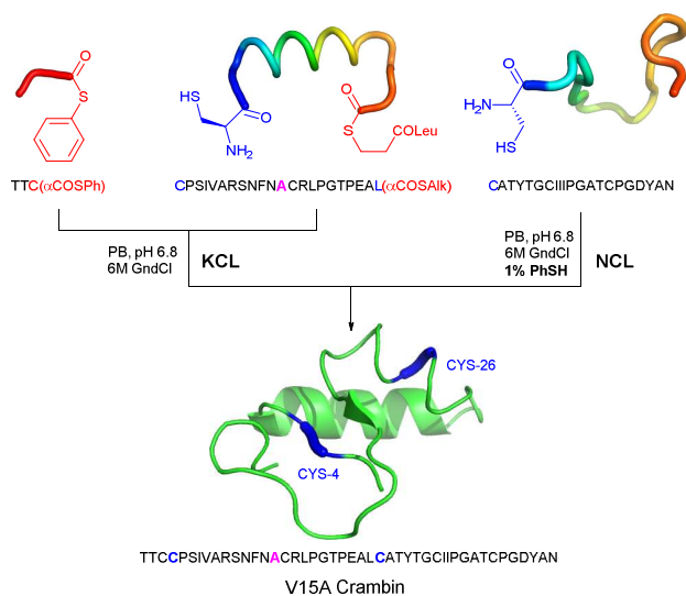
Fig. 80. Two final steps of the synthesis of V15A crambin (pdb: 3NIR) described by Bang and associated 675 . The mutation was introduced for simplifying the prior KCL step of assembling the second peptide. Kinetically controlled ligation of S Ar thioester spontaneously occurs in aqueous media in the absence of exogenous thiophenol, while native chemical ligation of S Alk thioester must be accelerated by the addition of 1% PhSH.
