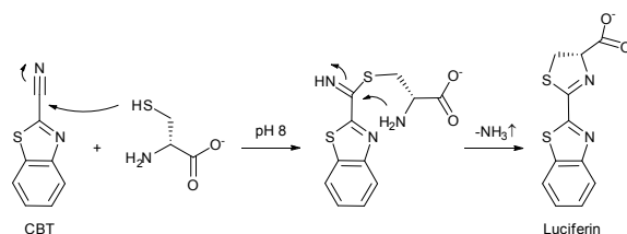
Fig. 87. Synthesis of luciferin by the reaction between cyanobenzothiazole (CBT) and D-cysteine. 774
