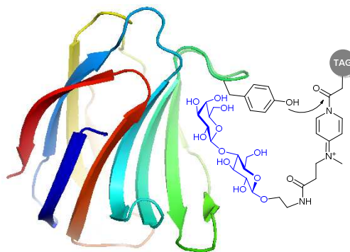
Fig. 52. Sugar-DMAP (4-dimethylaminopyridine) assisted Y51-specific acylation of Congerin II described by Hamachi et al. 486 Schematic representation is made using Lactose-ligated Congerin II crystal structure published by Muramoto et al. 488 (pdb: 1HS4).
