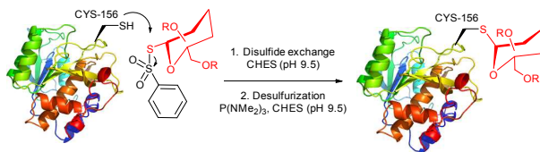
Fig. 30. Two-step protocol for the preparation of thioether linkage via disulfide exchange reaction followed by HMPT-mediated desulfurisation ( P(NMe_2)_3 , hexamethylphosphotriamide) of glycosylated mutant S156C SBL (wild-type pdb: 1GCI). 362
