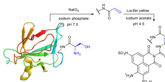
Fig. 74. N -terminal serine labelling of recombinant murine interleukin-1 \alpha (pdb: 2KK1) with Lucifer yellow dye described by Geoghegan and Stroh. 641 The method is also applicable if N -terminal threonine is present.
