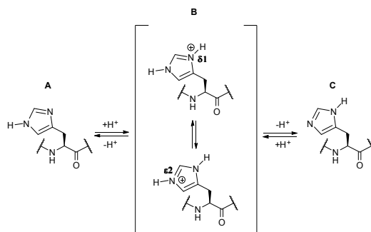
Fig. 47. Tautomerisation equilibrium of the neutral imidazole side chain (base forms A and C ) occurring through the acid form B . 457 Form A is somewhat favoured over C at neutral and acidic pH, while at basic pH the form C is preferred. 458
