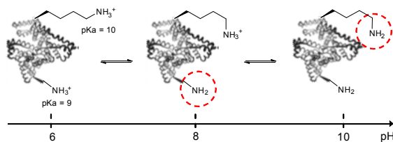
Fig. 1. Deprotonation of different types of amino groups present in protein structure (more nucleophilic amine is encircled in red). Lysine \epsilon -amino groups are more nucleophilic, but also more difficult to deprotonate. Generally, a pH of 8.5–9.5 is optimal for modifying lysine residues, while near neutral pH favours selective modification of N -termini.
