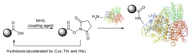
Fig. 6. Preparation of activated NHS-esters and their reaction with nucleophilic amino acid residues present in proteins. Similarly to isothiocyanates, the reversible reactions of thiol and alcohol groups with NHS-esters largely increase the rate of hydrolysis thereof.
