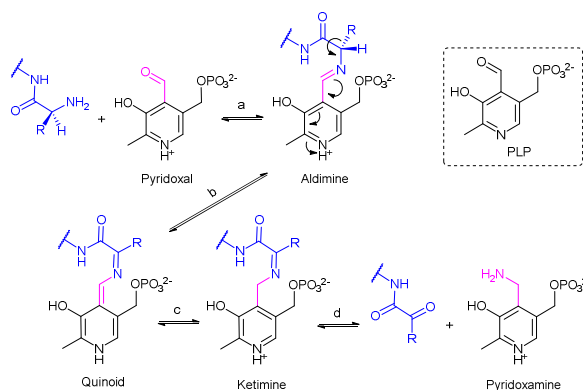
Fig. 68. Structure of PLP and mechanism of PLP-mediated transamination. Reaction pathway consists of (a) condensation reaction between pyridoxal and the amine; (b-c) tautomerisation of the obtained aldimine being favourable because of a much lower intrinsic pKa values of \alpha -proton (shown in blue); (d) hydrolysis of the resulting ketimine, accompanied by decarboxylation in the case of aspartic acid ( \text{R} = -\text{CH}_2\text{COOH} ). 601
