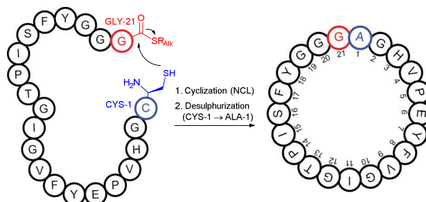
Fig. 84. Synthesis of 21-residue cyclic antibiotic peptide Microcin J25 via NCL-desulfurisation strategy resulting in ananyl-linked polypeptide chain developed by Yan and Dawson. 712 Reaction conditions: cyclisation – Tris-HCl, 6 M GndCl; desulfurisation – NaOAc, pH 4.5, 6 M GndCl, H 2 (Pd/Al 2 O 3 ).
