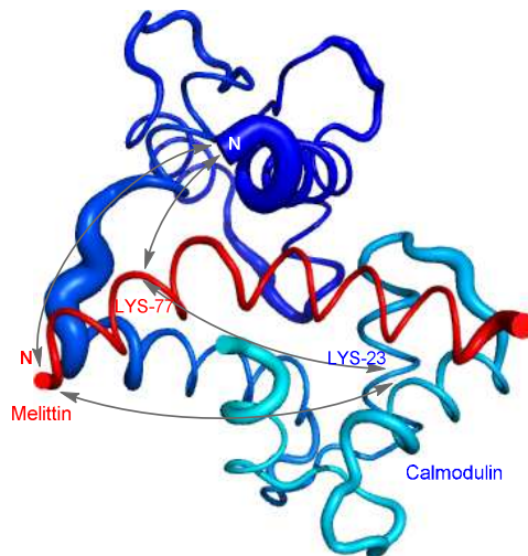
Fig. 7. Mode of binding of melittin in the calmodulin-melittin complex (pdb: 2MLT and 1CDL) calculated from ambiguous distance restraints derived from the cross-linking data by Sinz and associates. 114
