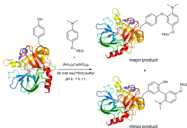
Fig. 56. PEGylation of four solvent-accessible Tyr residues of chymotrypsinogen (pdb: 1EX3) reported by Francis et al. 509 (only Y171 residue is shown for simplicity reasons). Intermediate tyrosyl radical, generated in the presence of cerium(IV) ammonium nitrate (CAN), gives two addition products with electron-rich aniline derivative ( O - is preferred over C -arylation).
