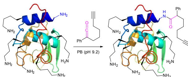
Fig. 66. Selective labelling of lysozyme (pdb: 2LYZ) described by Che. 603 Moderate-to-high level of selectivity towards N -terminal residue (K1) was achieved in the presence of 5 other in-chain lysines (LYS-13, LYS-33, LYS-96, LYS-97 and LYS-116). The ketene was synthesised from the corresponding acid by a two-step protocol: transformation into a mixed anhydride (oxalyl chloride, DCM) followed by the transformation thereof into ketene upon the reaction with a base (TEA, THF).
