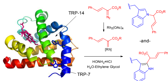
Fig. 44. Modification of horse heart myoglobin (pdb: 1YMB) with rhodium carbenoids described by Francis et al. 450 A 100 \mu\text{M} solution of myoglobin was exposed to stabilised vinyl diazo precursor (10 mM) and \text{Rh}_2(\text{OAc})_4 (100 \mu\text{M} ) for 7 h. N - and C -derivatization of indole rings of both Trp residues - TRP-14 and TRP-7 - were identified by the mass reconstruction. An excess of hydroxylamine hydrochloride (75 mM) is crucial for the efficiency of the conjugation, although its mode of action was not elucidated.
