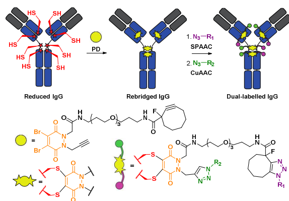
Fig. 33. Dual labelling of IgG antibody using dibromopyridazinediones (PD, shown in orange). 384 The construct obtained after rebridging of a reduced IgG with a PD-probe containing a strained alkyne (reactive in strain-promoted azide-alkyne cycloaddition, SPAAC) and a terminal alkyne (reactive in Cu-catalysed azide-alkyne cycloaddition, CuAAC) was subsequently labelled with two azide-containing probes ( N_3-R_1 and N_3-R_2 ).
