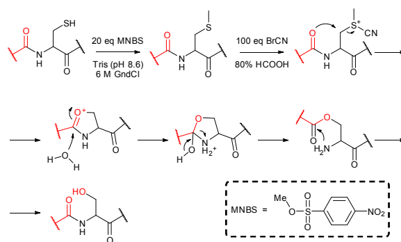
Fig. 77. Conversion of a Cys into a Ser residue by transforming the former into a corresponding methyl cysteine and following thereof by CNBr. 657 Methionine must be protected by transforming into corresponding sulfoxide form, because this is inactive for the CNBr reaction. 658
