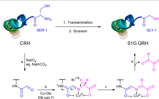
Fig. 75. Preparation of S1G mutant of corticotropin-releasing hormone (GRH) by regioselective transformation of N -terminal serine to glycine 604 Reaction steps: (a) selective serine oxidation by periodate; (b) formation of imine with amino group of glutamic acid precomplexed with Cu 2+ (Cu-Glu); (c) base-assisted isomerisation of imine; (d) hydrolysis of imine, completed when aspartate and copper ions are removed.
