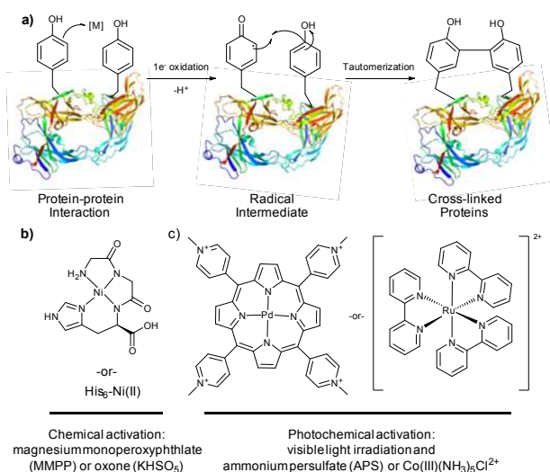
Fig. 55. Transition metal catalysed oxidative cross-linking. (a) Schematic representation of the protein-protein cross-linking, described by Burlingame et al. 506 The tyrosyl radical generated from ecotin (pdb: 1ECZ) D137H mutant after the abstraction of an electron with Ni(II)-GGH complex reacts with additional tyrosine residue on nearby protein that are in close proximity due to a significant protein–protein interaction to give a dimer. (b) Chemically activated by MMPP or oxone as stoichiometric oxidants, Ni(II)–peptide complexes can be used as efficient catalysts of cross-linking. (c) Photochemically activated by visible light in the presence of (NH 4 ) 2 S 2 O 8 or Co(III)(NH 3 ) 5 Cl 2 2+ as electron acceptors, transition metal complexes are used as catalysts of cross-linking.
