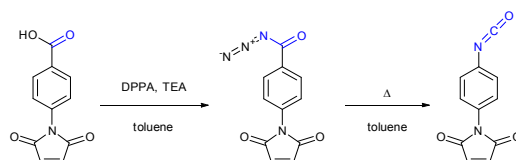
Fig. 2. Synthesis of p -maleimidophenyl isocyanate crosslinker via Curtius rearrangement proposed by Palumbo and associates. 33
