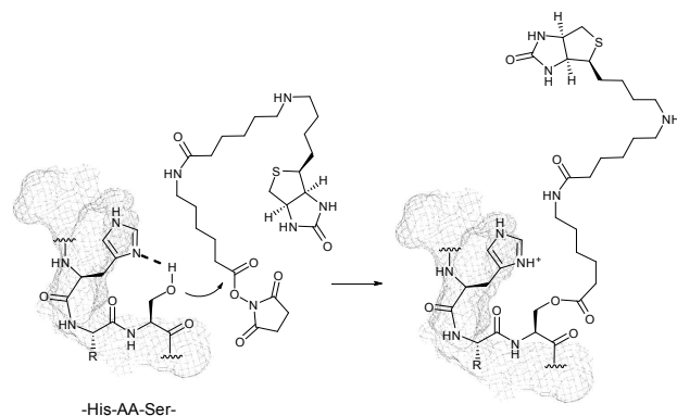
Fig. 18. Nucleophilic attack of serine on the NHS-activated ester gives the stable O -acylated derivative. In addition to His-AA-Ser, this stable intermediate can be formed in the presence of linear sequences of His-AA-Thr and His-AA-Tyr, where AA refers to any amino acid.
