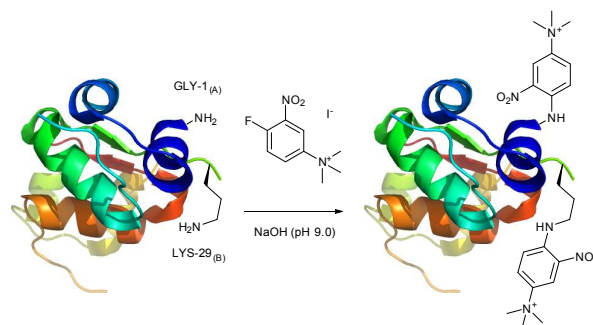
Fig. 14. Derivatization of bovine insulin with 1-fluoro-2-nitro-4-trimethylammoniumbenzene iodide described by Sutton et al. 195 Only amine-containing residues of A1 and B1 chains are shown. Two of the four tyrosine residues present in chains A1 and B1 (not shown) also react with the probe under described conditions.
