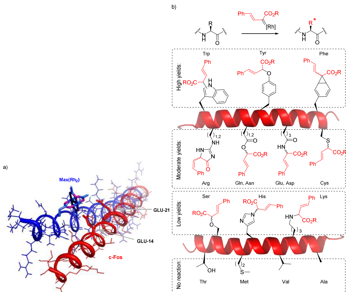
Fig. 96. a) Modification of c-Fos (shown in red) catalysed by Max(Rh 2 ) (shown in blue) metallopeptide described by Popp and Ball. 818 Two possible coiled-coil alignments result in modification of GLU-14 and GLU-21 residues, located in close vicinity to dirhodium catalytic center. b) Proposed product bond connectivity and
