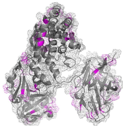
Fig. 10. Structure of Prevnar 13 vaccine. The bacterial capsule sugars, a characteristic of the pathogens, are linked to CRM197, a nontoxic recombinant variant of diphtheria toxin (pdb: 4AE0), by reductive amination at lysine residues and N -terminus (shown in magenta).
