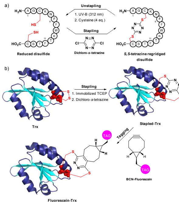
Fig. 34. Protein stapling-unstapling using dichloro- s -tetrazine described by Smith et al. a) Rebridging of a disulfide bond of a 14-mer peptide using dichloro- s -tetrazine and recovering of the starting product by photocleavage of the resulting S,S -tetrazine macrocycle (irradiation at 312 nm) followed by quenching of the thiocyanate intermediate with an excess of cysteine. b) Rebridging of thioredoxin (Trx, pdb: 2F51) after the disulfide bond reduction followed by tagging of the resulting S,S -tetrazine with a strained alkyne containing probe (BCN-Fluorescein).
