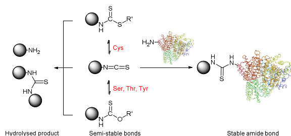
Fig. 4. Reaction of isothiocyanates with nucleophilic amino acid residues present in proteins. Only the reaction of lysine and N -terminal residues (considerable at pH > 5) results irreversibly in obtaining the thiourea. Although the reactions of thiol and alcohol groups with isothiocyanates are reversible, they can largely accelerate the rate of isothiocyanate hydrolysis.
