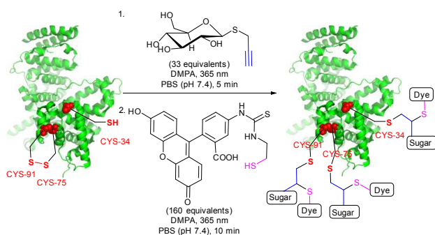
Fig. 28. Glycosylation and fluorescent labelling of bovine serum albumin (BSA, pdb: 3V03) by TYC (first step) followed by TEC (second step) with 2,2-dimethoxy-2-phenylacetophenone (DMPA) as photoinitiator. 345
