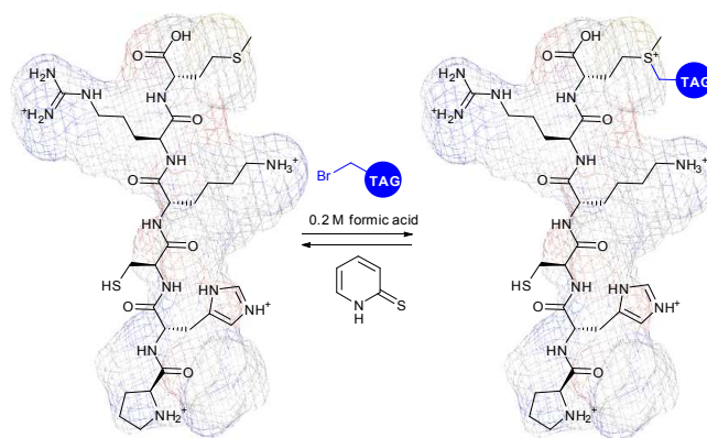
Fig. 65. Selective reversible modification of a 6-amino-acid peptide (PHCRKM) via methionine alkylation reported by Kramer and Deming. 588 No reaction with other amino acids were detected.
