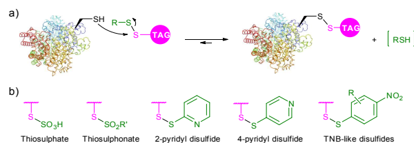
Fig. 29. a) General scheme of protein labelling via the formation of disulfide bond. b) Most relevant examples of activated thiols: thiosulfate, thiosulfonate, 2-pyridyl disulfide, 4-pyridyl disulfide, TNB-like thiol.
