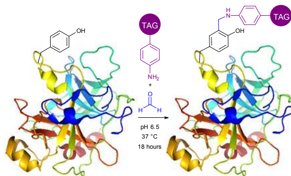
Fig. 58. Three-component Mannich-type selective modification of Y154 Tyr residue of \alpha -chymotrypsinogen A (pdb: 1EX3) by a rhodamine dye, described by Francis et al. 521
