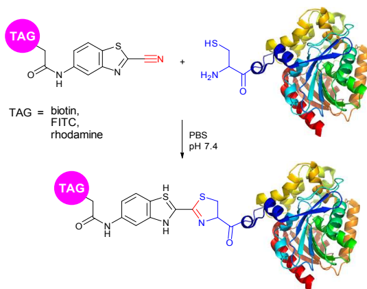
Fig. 88. Labelling of Renilla luciferase (pdb: 2PSD) by CBT-based probes. 777 N -terminal cysteine was generated by protease processing of the fusion protein.
