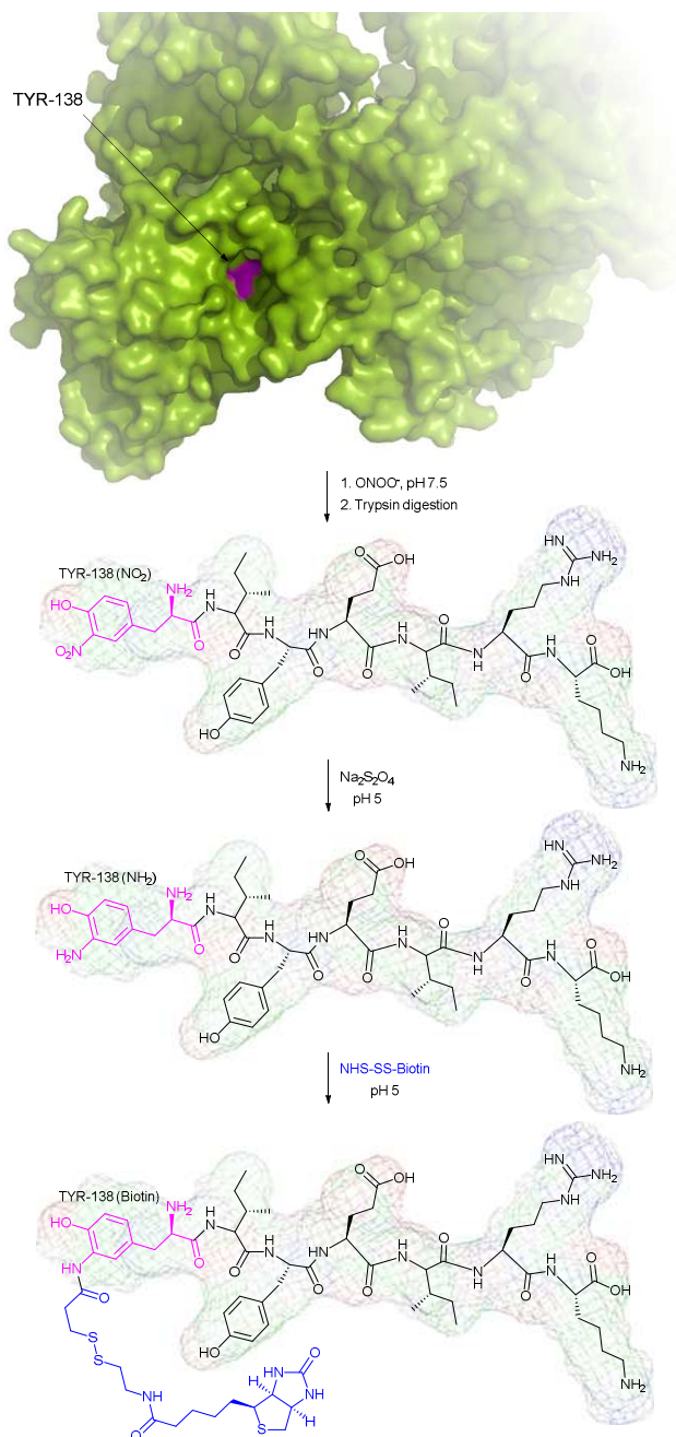
Fig. 53. Two-step biotinylation of HSA (pdb: 1AO6) described by Nikov et al. 492 a ) Preferential nitration of TYR-138 (shown in magenta) and TYR-411 residues of HSA with peroxynitrite was achieved using protocol described by Jiao and colleagues. 490 b ) Aminotyrosine of the peptide 138 YIYEIARK 144 , obtained after the step of reduction with sodium dithionite and following digestion of nitrated HSA with trypsin, were selectively modified with a cleavable biotin-containing reactant at pH 5.0.
