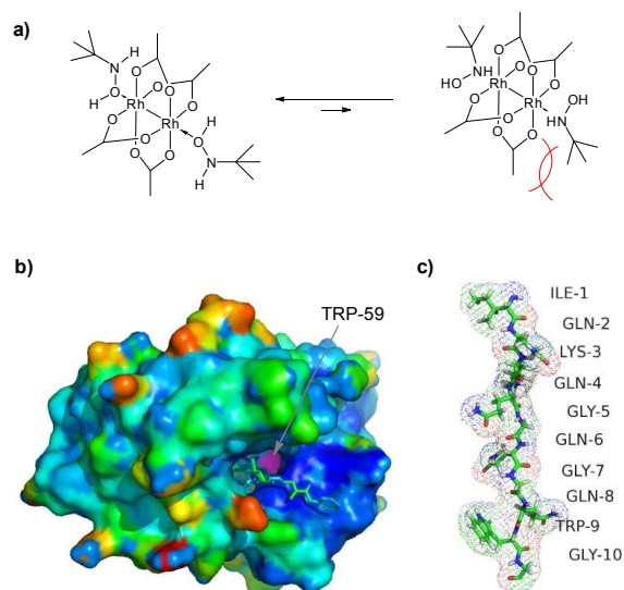
Fig. 45. Optimised metallocarbenoids-based approach, described by Francis and collaborators. 452 a) Proposed binding of t BuNHOOH with \text{Rh}_2(\text{OAc})_4 at pH 6.0. O -coordination is favoured due to a lowered sterical hindrance of tert -butyl groups with acetate ligands. b) Crystal structure of wild type FKBP (pdb: 1A7X), containing a single, buried tryptophan residue TRP-59 (shown in magenta), which is unavailable for modification under non-denaturing conditions. c) A peptide tag (IQKQGQGWG) incorporated into fusion FKBP protein expressed in E. coli as C -terminal intein fusion. The total level of modification was estimated to be in excess of 40%.
