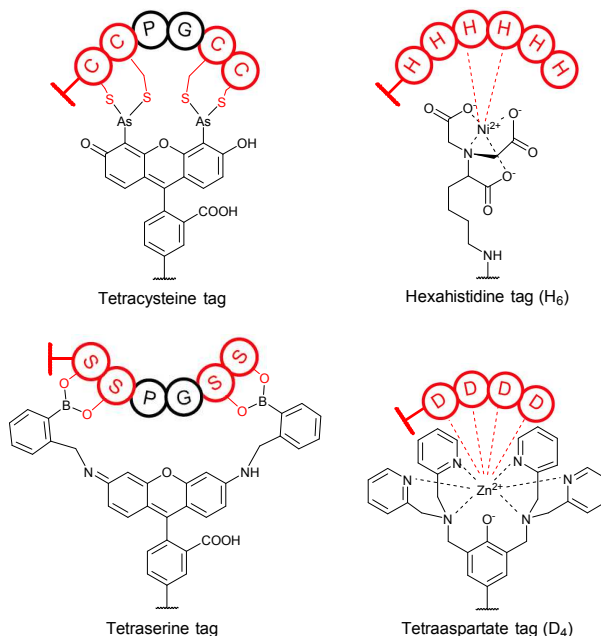
Fig. 94. Strategies for the selective conjugation of proteins based on metal-chelation: tetracysteine/biarsenical system, oligohistidine/nickel-complex system, tetraserine-borate system, oligo-aspartate/zinc-complex system. 27
