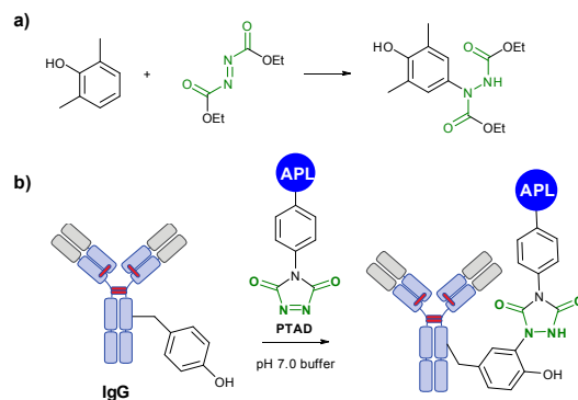
Fig. 59. Reaction of electron-rich arenes with azodicarboxyl compounds (shown in green). a ) First example described by Schroeter in 1969. b ) Conjugation of an HIV entry inhibitor apilaviric (APL) containing a cyclic diazodicarboxamide derivative - 4-phenyl-3H-1,2,4-triazoline-3,5(4H)-dione (PTAD) – with IgG antibody demonstrated by Barbas. 537
