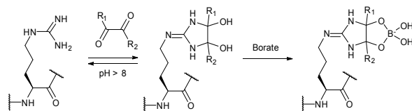
Fig. 62. Reaction of 2,3-butanedione with arginine residues of Carboxypeptidase A (pdb: 1HDU) in the presence of borate described by Riodan. 560
