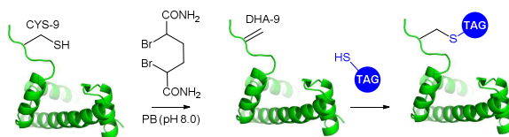
Fig. 38. Dehydroalanine-mediated conjugation on histone 3 mutant H3. 393
