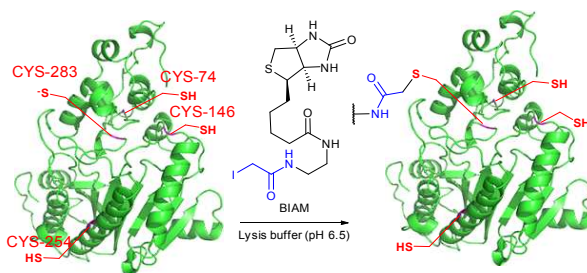
Fig. 19. Biotinylation of low- pK_a cysteine residue of rabbit muscle creatine kinase (CK, pdb: 2CRK) by BIAM. 249 The charge interaction between the negatively charged thiolate and the positively charged amino acid residues nearby results in significantly lower pK_a value of the CYS-283 residue (6.5). Consequently, selective alkylation thereof becomes possible in the presence of three other cysteine residues with higher pK_a values (8.0-9.0).
