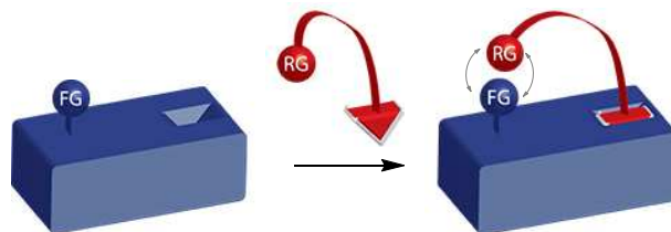
Fig. 95. Schematic representation of the proximity-driven approach for selective modification of macromolecules. Combining of promiscuous reactivity of the reactive group (RG, shown in red) with specific molecular recognition results in specific modification of the functional group of interest (FG, shown in blue).
