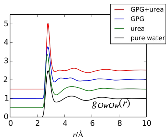
Fig. 3 RDF for water oxygens (Ow) from the GPG:urea:water EPSR fits to the neutron data compared with the same function in pure water 33 , gpg:water, 16 and urea:water 51 solutions.
