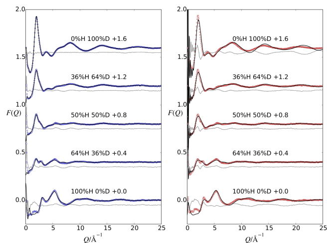
Fig. 2 Measured diffraction data ( F(Q) ) for GPG and urea in aqueous solution compared with the EPSR fits to the diffraction data and MD simulations. The data and corresponding fits have been shifted for clarity.
