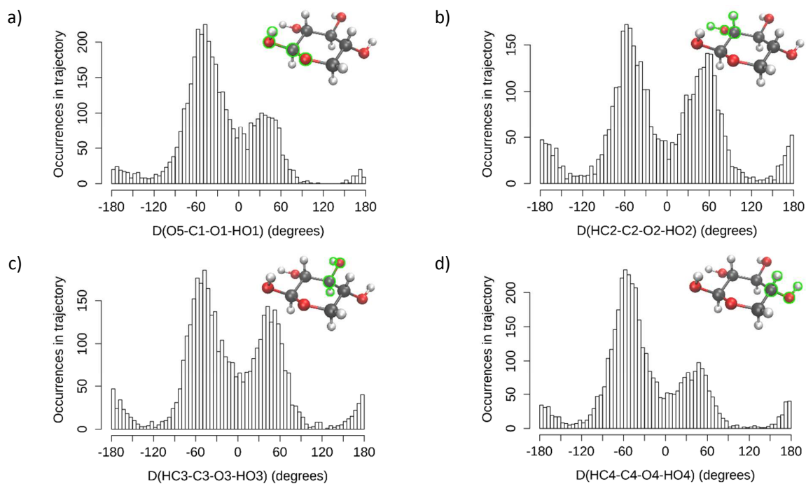
Figure 3: Values distribution of the selected dihedral angles along the MD trajectory (NVT production run), purged of the “inverted” chair ring conformation: a) D(O5-C1-O1-HO1) , b) D(HC2-C2-O2-HO2) , c) D(HC3-C3-O3-HO3) and d) D(HC4-C4-O4-HO4) .
