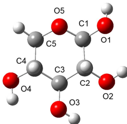
Figure 1: Ball and stick representation of \beta -D-xylose with the numbering scheme used herein. Carbon, hydrogen, and oxygen atoms are shown in grey, white, and red, respectively. Hydrogens are referred to by adding the atom label it is linked to as suffix, e.g. HO3 for the hydrogen linked to O3.
