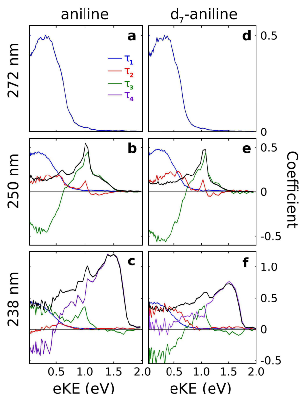
Fig. 3 Spectral components of C_i(\text{eKE}) extracted from the time-resolved photoelectron spectra (Fig. 2) using the decay times listed in Table 1 and eq. (2). The sum of C_i(\text{eKE}) (black lines) represents the photoelectron spectrum of the initially excited state.
