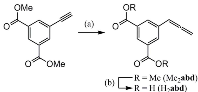
Scheme 1 Synthesis of H_2\mathbf{abd} via Me_2\mathbf{abd} . a) CuI (0.5 equiv), (CH_2O)_n (2.5 equiv), iPr_2NH (1.8 equiv), dioxane, reflux; b) NaOH (10 equiv), THF, 4h, RT, acidic workup.
