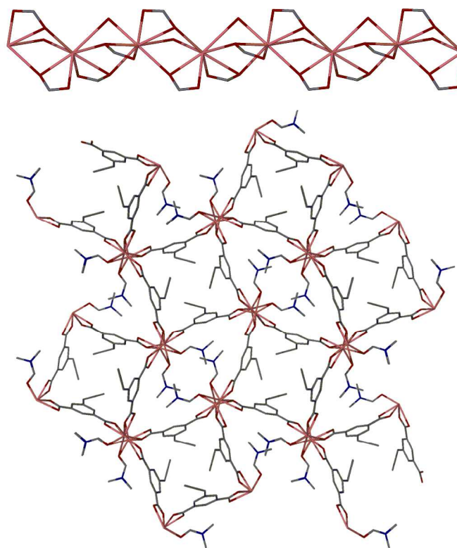
Fig. 4 (Top) Bridging carboxylates link Pb(II) atoms into a chain motif. (Bottom) Bridging abd ligands link the cluster chains into a complete 3D network.
