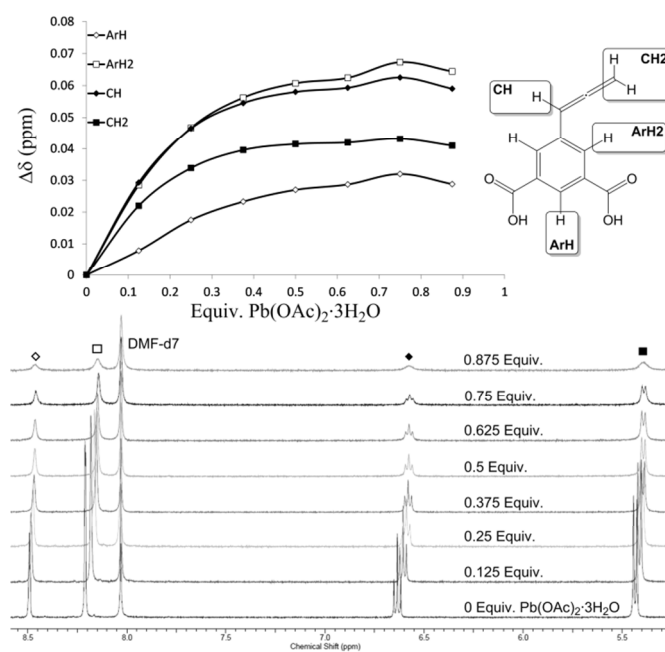
Fig. 2 Titration isotherm and 1 H-NMR spectroscopic titration stack plot for the interaction between H 2 abd and Pb(OAc) 2 ·3H 2 O in DMF- d 7 .
