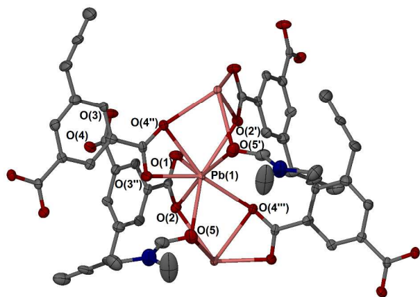
Fig. 3 Coordination environment about the Pb(II) atom in 2 . Thermal ellipsoids are shown with 50% probability. Symmetry operators: (') = \frac{1}{2} + y, x - \frac{1}{2}, z - \frac{1}{2} , (')' = 1 - y, x, -z , (''') = \frac{1}{2} + x, \frac{1}{2} - y, \frac{1}{2} - z .
