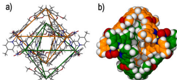
Figure 11 Taken from the crystal structure of the triply-interlocked [2]catenane ( \pm )- [\text{Zn}_6(\mathbf{8})_4(\text{NO}_3)_6]^{6+} , in which the two mechanically interlocked metallo-cryptophanes are a) displayed in skeletal form with the topological crossing points denoted by the green and orange wire frames, and b) colour-coded and displayed in space filling mode. 54
