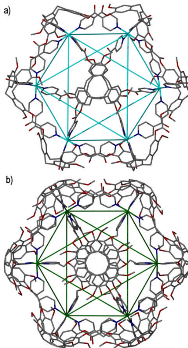
Figure 14 The solid state structures of a) enantiopure [Pd 6 ( 11 ) 8 ] 12+ and b) mixed enantiomer [Pd 6 ( 13 ) 8 ] 12+ ‘stella octangula’ cage assemblies, in
