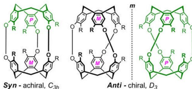
Figure 3 Molecular cartoons depicting the possible stereochemical configurations that result from the synthesis of traditional, organically-linked cryptophanes. Enantiomers of the tribenzo[ a,d,g ]cyclononatriene core are given the descriptors M and P and colour-coded for clarity.
