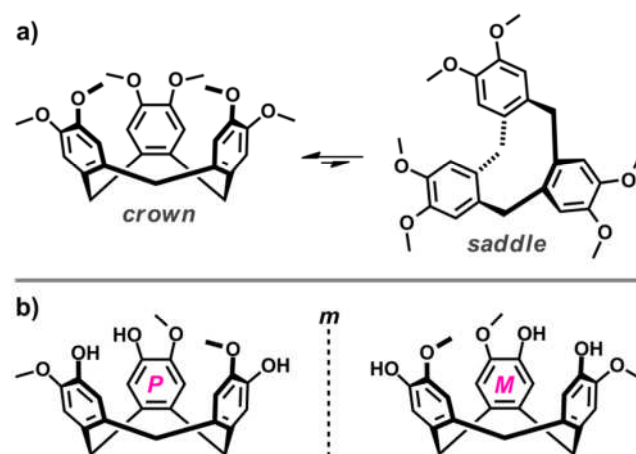
Figure 1 The molecular structures of a) cyclotrimeratrylene (CTV) and b) cyclotrimeratrylene (CTG). The bowl-to-bowl inversion of CTV is indicated by the biased equilibrium between the crown and saddle molecular conformations. The two enantiomers ( M and P ) of CTG are shown and separated by a mirror plane ( m ).
