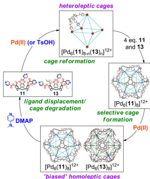
Figure 16 The complex assembly/disassembly cycle determined for the chirality and speciation control experiments between all accessible 'stella octangula' coordination cages. 64
