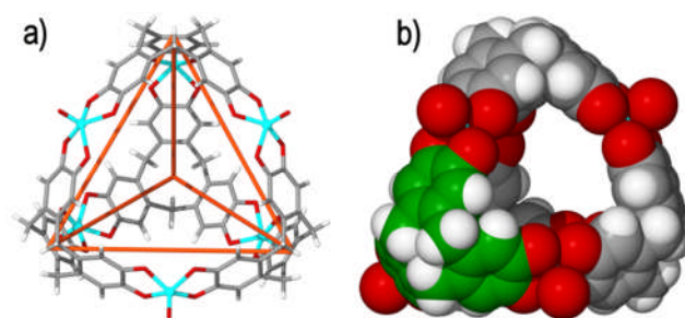
Figure 4 The solid state structure of Robson's [(VO) 6 (CTC-6H) 4 ] 12- tetrameric assembly, depicting a) the tetrahedral cage framework, as indicated by the orange lines that connect each deprotonated CTC ligand, and b) the space filling model, highlighting the internal void space. One CTC ligand of the assembly is colour-coded for clarity. 31
