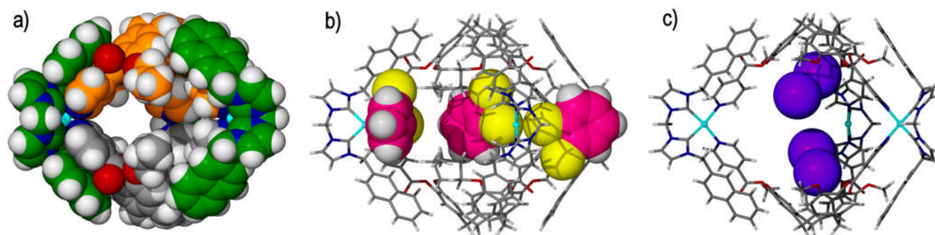
Figure 13 Taken from the crystal structure of a) the parent syn -[Pd 3 (Nap) 3 ( 13 ) 2 ].6(BF 4 ) metallo-cryptophane, displayed in space-filling mode and with each 13 ligand of the head-to-head assembly distinguishable by colour and the cis -protecting NHC auxiliary coloured green for clarity. Host-guest inclusion complexes are displayed in b) syn -[Pd 3 (Nap) 3 ( 13 ) 2 ].6(BF 4 ).3(DCB) and c) syn -[Pd 3 (Nap) 3 ( 11 ) 2 ].6(BF 4 ).3(I 2 ), in which the metallo-cryptophanes are shown in skeletal form and the DCB and iodine guests (some disordered positions excluded) are shown in space-filling mode and coloured pink and purple, respectively. 73
