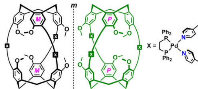
Figure 9 Cartoon depictions of the two enantiomers of Shinkai's anti - [\text{Pd}_3(\mathbf{6})_2]^{6+} metallo-cryptophane, as separated by a mirror plane ( m ). 45
