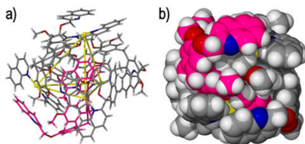
Figure 7 The solid state structure of the tetrameric [Ag_4(4)_4]^{4+} twisted tetrahedron, depicting a) the tetrahedral arrangement of silver(I) cations by use of solid, yellow lines and b) the resultant cubic structure, as
