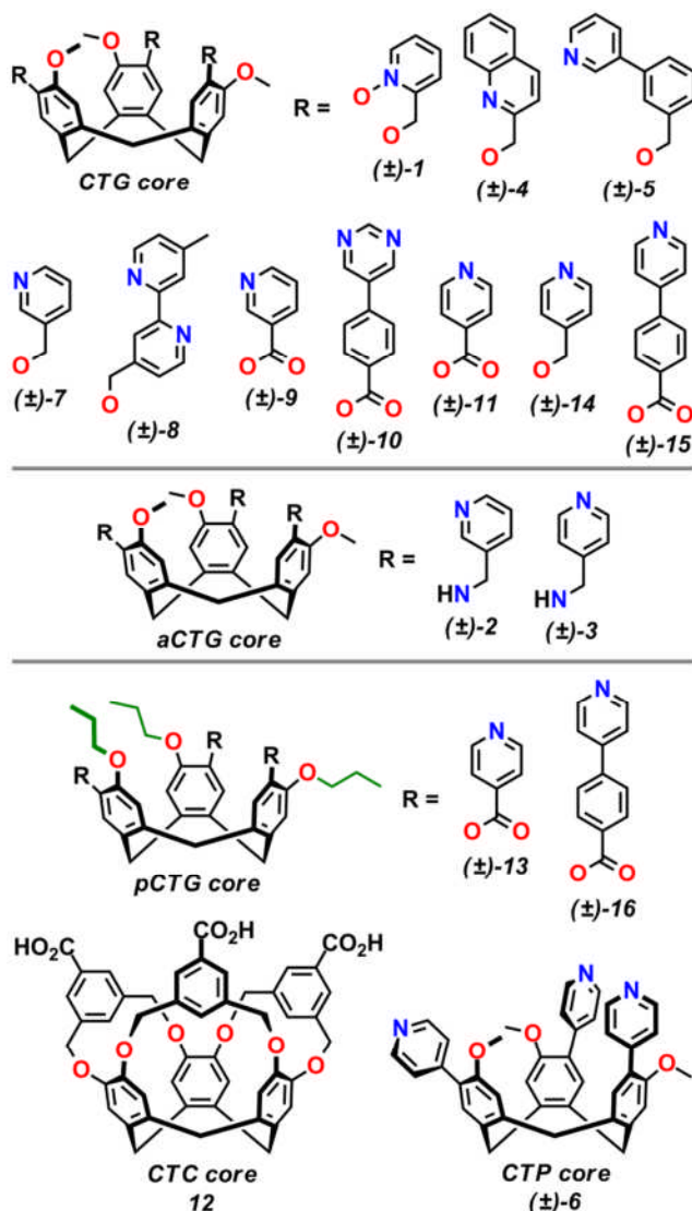
Figure 2 The molecular structures of ligands 1–16 referred to in this review article. Ligands are categorised according to the upper-rim functionality of the tribenzo[ a,d,g ]cyclononatriene core.
