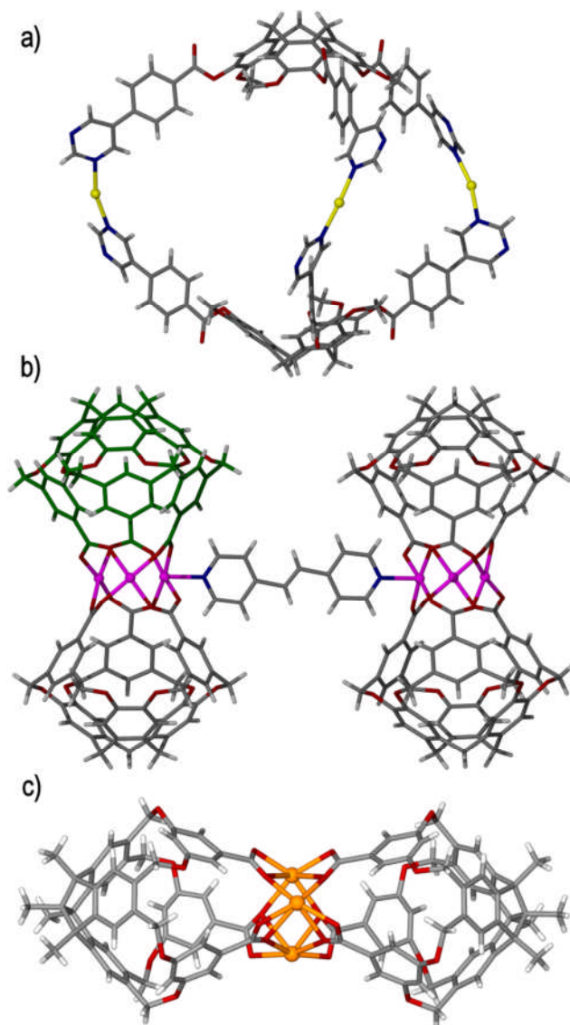
Figure 12 The solid state structures of a) the chiral anti -[Ag 3 ( 10 ) 2 ] 3+ metallo-cryptophane, 47 b) the 'bow-tie' metallo-cryptophane, [Cu 3 ( 12 ) 2 (DMF)(H 2 O) 2 ] 2 (BPE), 59 and c) tribenzotriquinacene triacid based [Cd 3 L 2 ] metallo-cryptophane. 63
