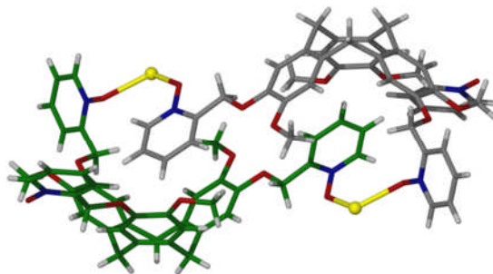
Figure 5 The skeletal structure of complex [Ag 2 ( 1 ) 2 ] 2+ , evidencing the flattened 'handshake' motif. One of the two 1 ligands is colour-coded and all solvent molecules and anions are omitted for clarity. 33
