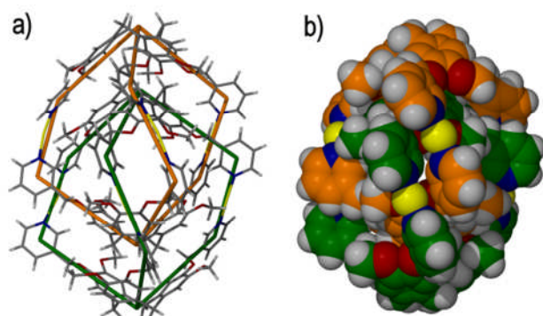
Figure 10 The solid state structure of the triply-interlocked [2]catenane [\text{Ag}_6(\mathbf{7})_4]^{6+} , in which only the ( \Delta,\Delta )- [\text{Ag}_6(\mathbf{7})_4]^{6+} enantiomer is shown. The mechanically interlocked components are shown as a) wire frames and b) in space filling mode. In both illustrations the two chemically independent metallo-cryptophanes are colour-coded for clarity. 47
