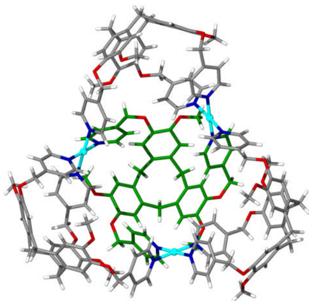
Figure 15 The skeletal structure of the [\text{Pd}_3(\mathbf{14})_4]^{6+} half-cage, closely resembling half of a 'stella octangula' cage. The ligand at the base of the tetrameric assembly is coloured green for clarity. 83
