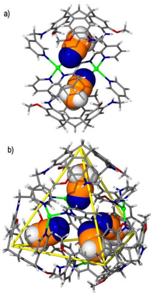
Figure 6 The solid state structures of a) the dimeric capsular assembly [Ag_2(2)_2(MeCN)_2]^{2+} and b) the [Ag_4(3)_4(MeCN)_4]^{4+} tetrahedral cage. Non-covalently bound MeCN guests are coloured orange and displayed in space-filling mode in each case for clarity. The tetrahedral framework of [Ag_4(3)_4(MeCN)_4]^{4+} is denoted by the use of solid, yellow lines that connect the base of each 3 ligand. 37
