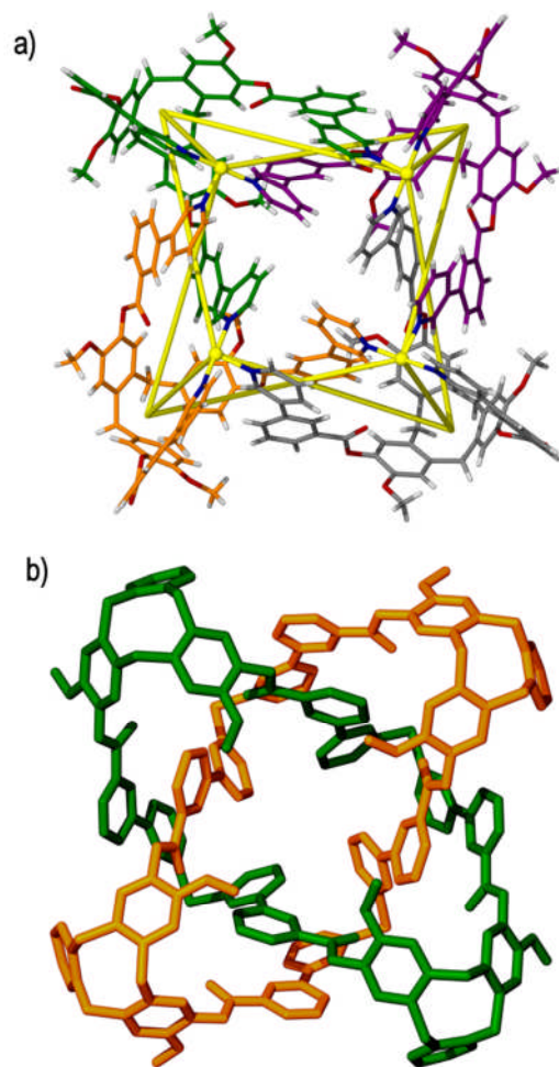
Figure 8 The topologically complex [\text{Pd}_4(\mathbf{5})_4(\text{NO}_3)_2(\text{H}_2\text{O})_2]^{6+} Solomons cube, highlighting a) the molecular structure and four topological crossing points within the assembly (shown as yellow lines bridging the
