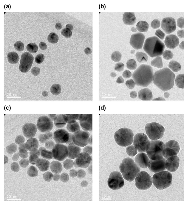
Fig. 2. Exemplar TEM images of (a) AgNP@( 3 ) using 10 mM Tollens' and 10 mM ( 3 ), \phi = 15 \pm 4 nm. (b) AgNP@( 4a ) using 10 mM Tollens' and 10 mM ( 4a ), \phi = 18 \pm 7 nm. (c) AgNP@( 4b ) using 10 mM Tollens' and 10 mM ( 4b ), \phi = 17 \pm 5 nm. (d) 10 mM Tollens' and 25 mM ( 4b ), \phi = 38 \pm 7 nm.
