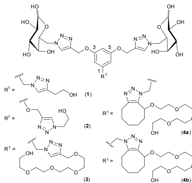
Fig. 1. Structures of sugar triazole ligands ( 1-4 ).
