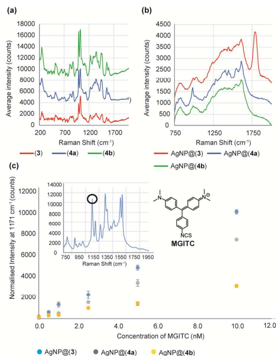
Fig. 3. (a) Stacked Raman spectra of sugar ligands (785 nm excitation; 1 accumulation; 1 s scan (3) ; 10 s scan (4a) ; 5 s scan (4b) ). (b) Stacked SERS spectra of \text{AgNP@}(3) , \text{AgNP@}(4a) and \text{AgNP@}(4b) (532 nm excitation; 1 s scan; 1 accumulation). (c) Plot of the intensity of the 1171 \text{ cm}^{-1} peak of MGITC using \text{AgNP@}(3, 4a-b) at decreasing concentrations of MGITC. Inset- SERS spectrum of MGITC using \text{AgNP@}(4a) highlighting the peak of interest.
