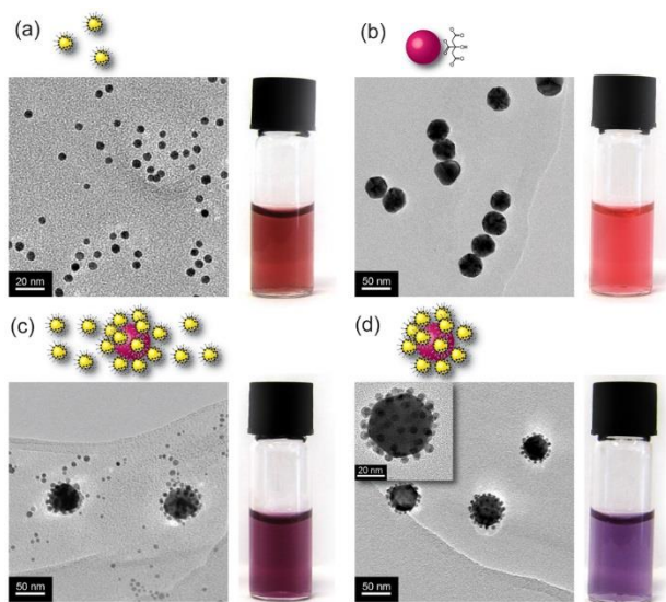
Fig. 2 TEM and visual characterization of component NPs and planet-satellite NP assemblies. (a) AuNP-1; (b) citrate-stabilized AuNPs (40 nm); (c) AuNP-1:citrate-NP (280:1); (d) purified planet-satellite assemblies. Photographs show the aqueous dispersions obtained at each stage.
