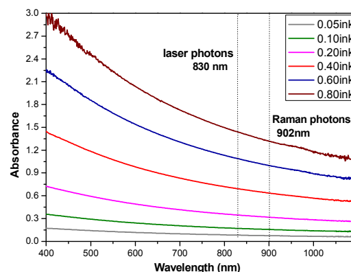
Figure 4: Absorbance spectra of different Indian ink aqueous solutions concentrations (in microliters/ml) in the range of 400-1100 nm. The cuvette path length in the measurements is 1 cm.
