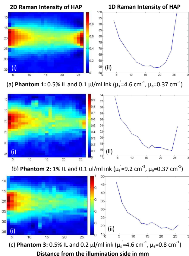
Figure 3: Raman scattering 2D(i) and 1D(ii) plots of different Intralipid/ink concentration HAP tissue phantoms.
