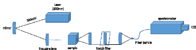
Figure 8: Diagram of the deep Raman setup in a transmission mode used.
