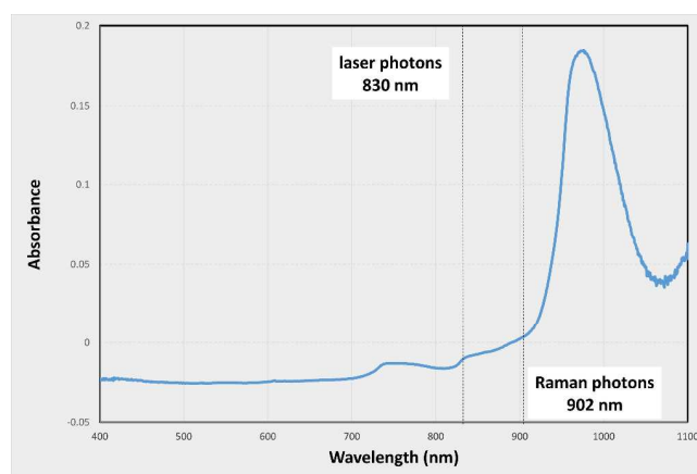
Figure 2: Absorbance spectra of water in the range of 400-1100 nm. Negative absorbance values are due to the difference in refractive index between air (used as a blank in the cuvette) and water. The cuvette path length in the measurements is 1 mm.
