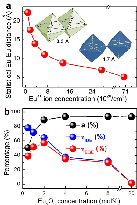
Figure 3. (a) Average statistical \text{Eu}^{3+} - \text{Eu}^{3+} distance as a function of volumetric ion concentration of \text{Eu}^{3+} . The inset of (a) exemplarily shows edge and corner-sharing octahedral [\text{EuO}_6] species through a linear Eu-O-Eu group. The labels indicate the corresponding minimum Eu-Eu-distance. (b) Variation of absorbance (a), internal quantum efficiency ( \eta_{IQE} ) and external quantum efficiency ( \eta_{EQE} ) of red PL of \text{Eu}^{3+} under excitation at 394 nm in YAB-xEu glasses versus doping concentration of \text{Eu}_2\text{O}_3 . The drawn lines in the inset of (a) and (b) are to guide the eye.
