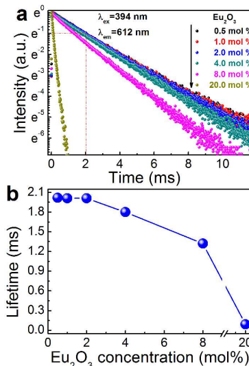
Figure 2. (a) Decay kinetics of the Eu^{3+}: {}^5D_0 \rightarrow {}^7F_2 emission at 612 nm as a function of Eu_2O_3 doping concentration under excitation at 394 nm. (b) Variation of the effective lifetime \tau_{1/e} ( \lambda_{em}=612 nm and \lambda_{ex}=394 nm) as a function of doping concentration.
