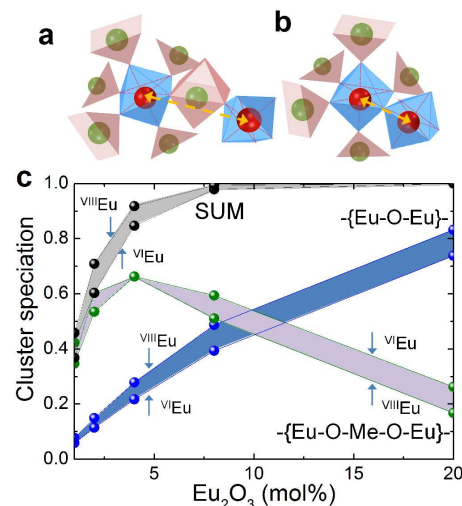
Figure 4. (a-b) Schematic illustration of the -\{\text{Eu-O-Eu}\} - and -\{\text{Eu-O-Me-O-Eu}\} (Me = B, Y, Al) linkages in the first and second coordination shell, respectively, of the \text{Eu}^{3+} ion. (c) Probability of cluster speciation P_{\text{Eu-Eu}} and P_{\text{Eu-Me-Eu}} , and sum of ( P_{\text{Eu-Eu}} + P_{\text{Eu-Me-Eu}} ), calculated for the two extremes of coordination number (six- and eight) as a function of \text{Eu}_2\text{O}_3 concentration. The drawn lines in (c) are to guide the eye.
