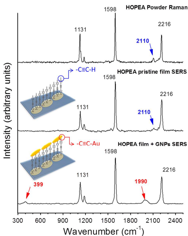
Fig. 6 Raman spectrum of HOPEA powder, SERS spectrum of a pristine HOPEA monomolecular LB film, and SERS spectrum of a HOPEA monomolecular LB film after incubation in a dispersion of GNPs.
