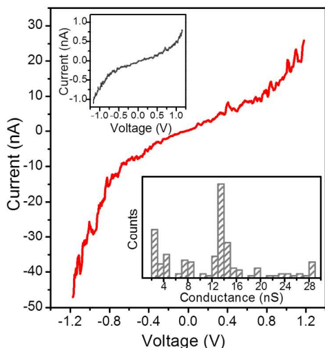
Fig. 8. Representative I - V curve obtained experimentally by positioning the c-AFM tip on top of a GNP when a set-point force of 16.7 nN was applied. Inset bottom: conductance histogram built by adding all the experimental data from -0.45 to 0.45 \text{ V} for each I - V curve obtained (ca. 550 curves). Inset top: representative I - V curve
