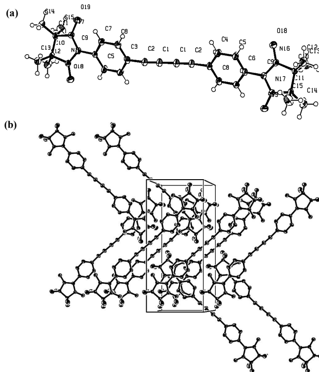
Figure 4 X-ray structure and the crystal packing of 3c with ORTEP drawn at the 50% of the probability level: (a) molecule; (b) crystal packing. View along the c axis of the crystal packing of compound 3c .
