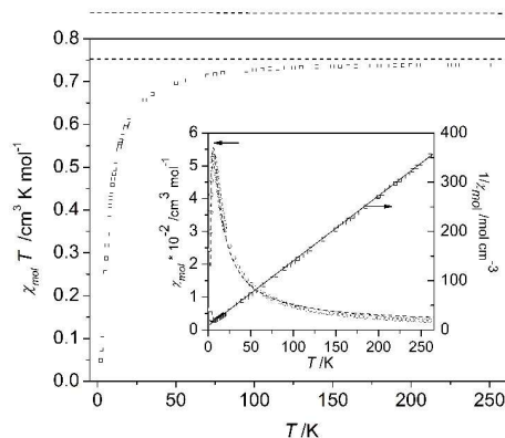
Figure 6 Magnetic susceptibility in a representation \chi_{mol} \cdot T of biradical 4c . The broken line indicates the theoretical value of 0.75 cm 3 K mol -1 for a dimer system formed by two spin S = 1/2 entities. Inset: molar susceptibility \chi_{mol} (left scale) and its inverse 1/\chi_{mol} (right scale) as a function of temperature together with fits performed by using a Curie-Weiss expression (solid line) and a Bleaney-Bowers equation 26 (broken line). For fitting parameter and details see text.
