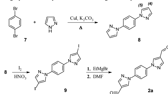
Scheme 2 Synthetic route towards dialdehyde 2a .
