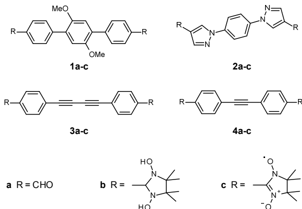
Figure 1 Model compounds 1-4 with emphasized bridging units.
