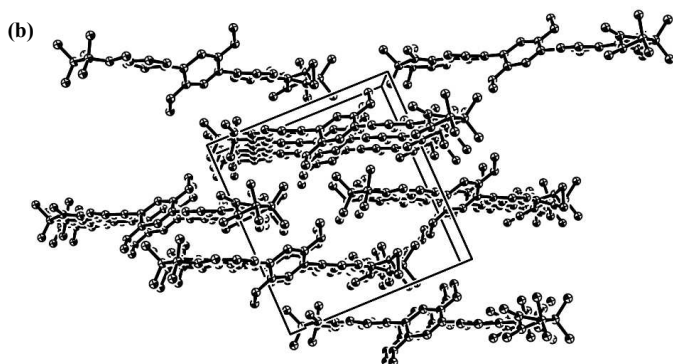
Figure 3 X-ray structure and the crystal packing of 1c with ORTEP drawn at the 50% of the probability level: (a) molecule; (b) crystal packing.
