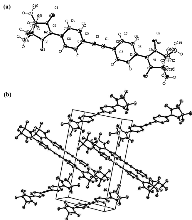
Figure 5 X-ray structure of 4c with ORTEP drawn at the 50% of the probability level: (a) molecule; (b) crystal packing.
