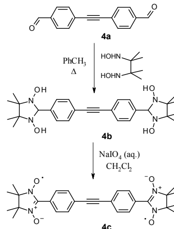
Scheme 4 Synthesis of the imidazolidine 4b and biradical 4c .
