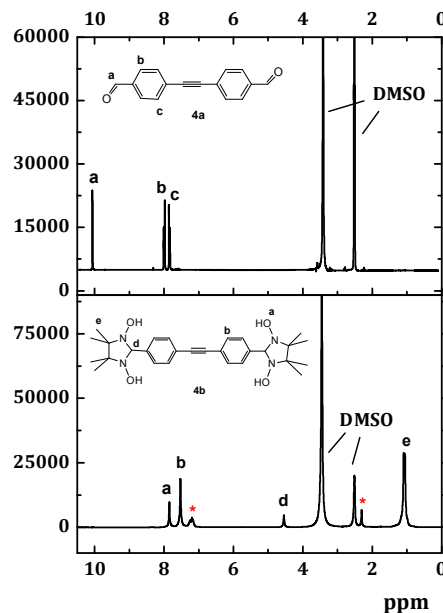
Figure 2 NMR spectrum of 4a,b in DMSO at 250 MHz (128 and 105 scans, respectively). The intensities of the solvent signals differ so much due to the significantly lower solubility of the dialdehyde 4a in DMSO. The asterisk indicates toluene.
