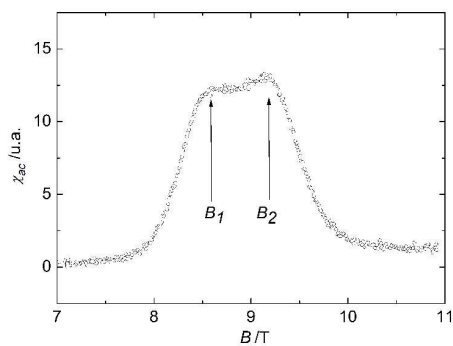
Figure 7 AC-susceptibility of the biradical 4c at T = 191 \text{ mK} . The data feature rounded peaks at B_1 \approx 8.6 \text{ T} and B_2 \approx 9.2 \text{ T} .
