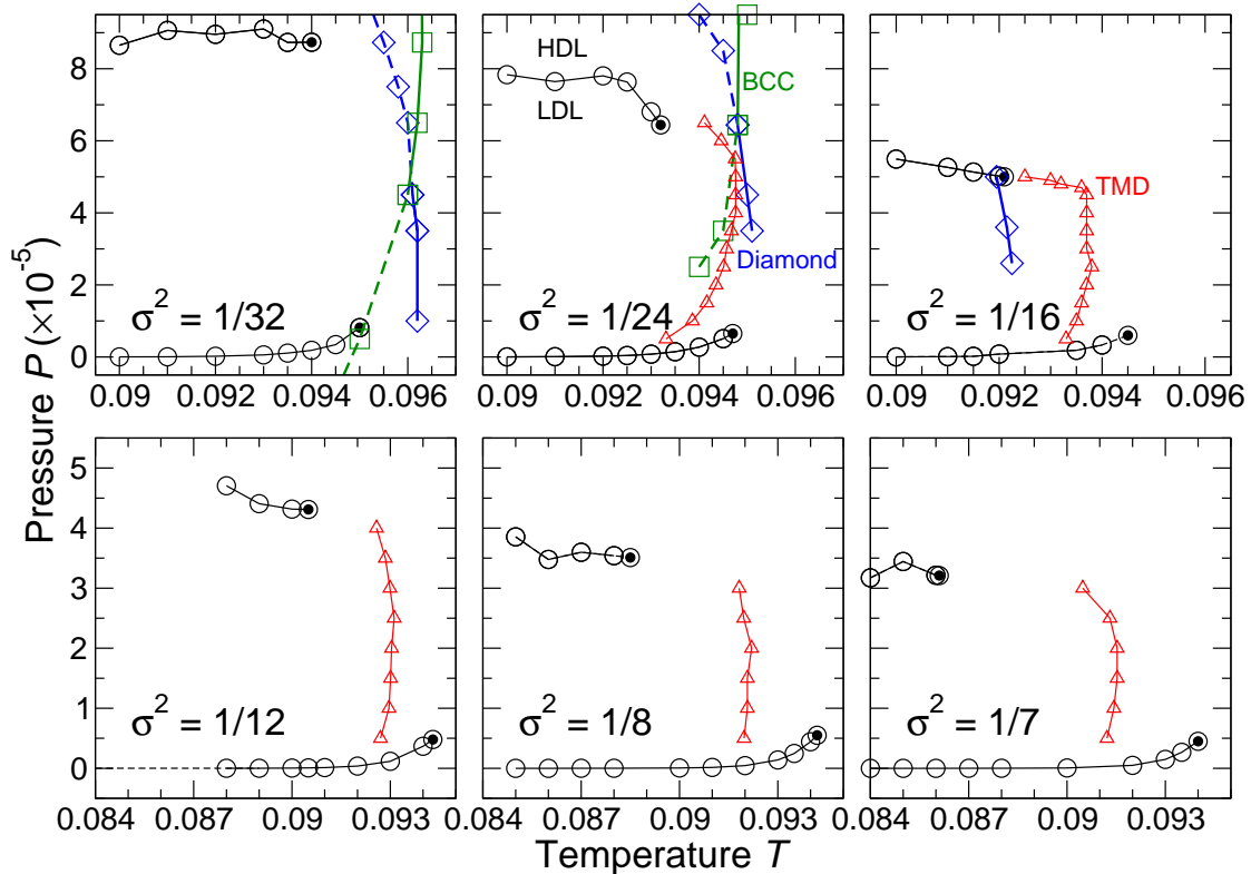
FIG. 5: T - P phase diagram for various bond orientational flexibility values \sigma^2 . For \sigma^2 < 1/16 , the liquid-liquid transition is metastable with respect to the crystals. The melting locus for the diamond lattice is shown by the blue diamonds, and for BCC by the green squares. The solid lines interpolate between points, and indicate melting of a stable crystal. The dashed lines indicate melting of the crystal, where the melting is metastable to another crystal. For \sigma^2 > 1/16 , we cannot accurately evaluate the melting locus, but confirm that crystals melt well below T_c at P_c for the LL transition. Also note that the LL coexistence line generally has a negative slope, a feature expected for water, but not present in many simple models exhibiting a liquid-liquid transition. The red triangles indicate the locus of temperature of maximum density of the amorphous phase.
