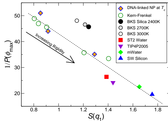
FIG. 9: Universal description of the structure of tetrahedral fluids, given by the variation of the pre-peak S(q_1) with the inverse of the peak in P(\phi_{\max}) . Data for the present study are shown by orange diamonds, at \rho_d^3/\rho_d = 1 and T_c for LL phase separation. From left to right, the \sigma^2 values for these points are 1/12, 1/16, and 1/24. The data for the other systems were taken from ref. [56].
