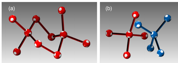
FIG. 1: Snapshot of a molecules in (a) the low-density liquid (LDL) and (b) the high-density liquid (HDL). In each case, we select two nearby NP which are not directly bonded, and draw the four neighbors to which they are bonded. For LDL, the resulting combined network is fully connected. For HDL, the higher density is achieved by interpenetration of the two locally bonded clusters.
