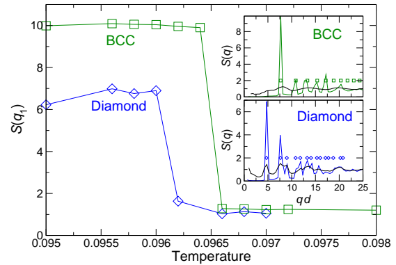
FIG. 3: Example of the identification of the melting temperature T_m for the diamond and BCC lattices for \sigma = 1/32 . The amplitude of the primary peak q_1 of the structure factor S(q_1) has an essentially discontinuous drop upon melting of the crystal, allowing to narrow the range for T_m . The insets show the full structure factors S(q) from which the first peak is extracted. For each crystal, we show S(q) immediately below (green or blue) and above (in black) T_m . The small symbols in the insets mark the expected Bragg peak locations for ideal diamond or BCC organizations. We obtain similar data for all other \sigma studied.
