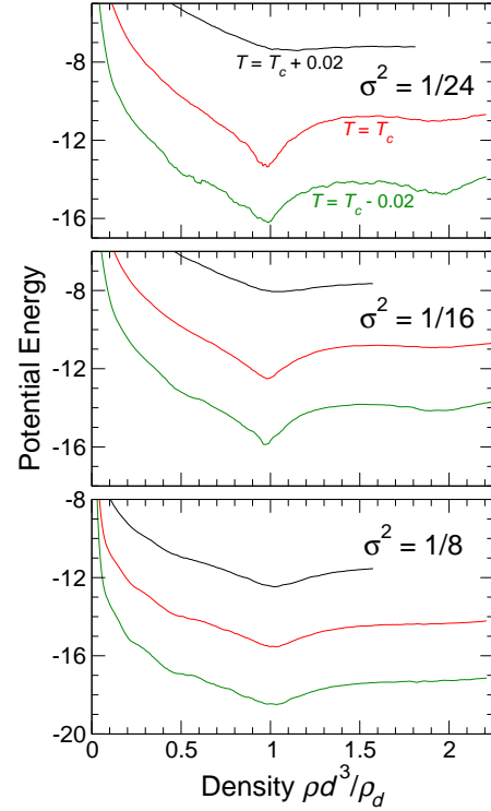
FIG. 7: Potential energy as a function of density for (a) \sigma^2 = 1/24 , (b) \sigma^2 = 1/16 , and (c) \sigma^2 = 1/8 . For each bond flexibility, we show three temperatures near T_c for the liquid-liquid phase separation.
