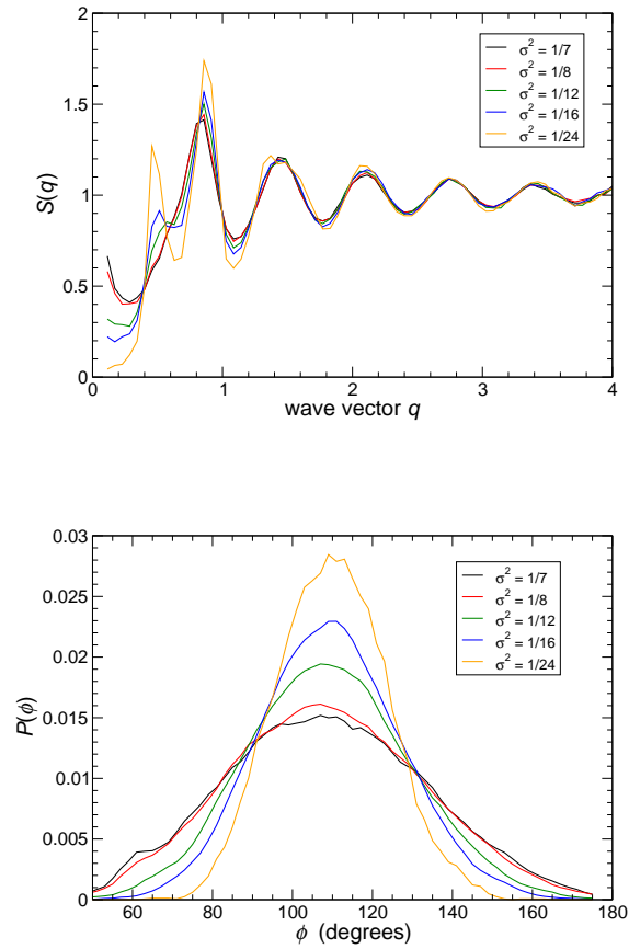
FIG. 8: Structure of the fluid at the critical temperature T_c for LL phase separation at the ideal tetrahedral density \rho_d^3/\rho_d = 1 , quantified by (a) the structure factor S(q) and (b) the distribution P(\phi) of the angle \phi defined by three bonded neighbors.
