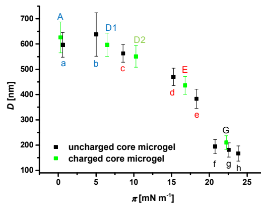
Figure 6. Mean nearest neighbor distance as a function of the surface pressure. D was determined from the position of the first peak in the g(r) functions corresponding to the AFM images in Figure 4 and 5. Error bars represent the standard deviation and were calculated from the full width of half maximum of a Gauss fit on the first oscillation of g(r) .
