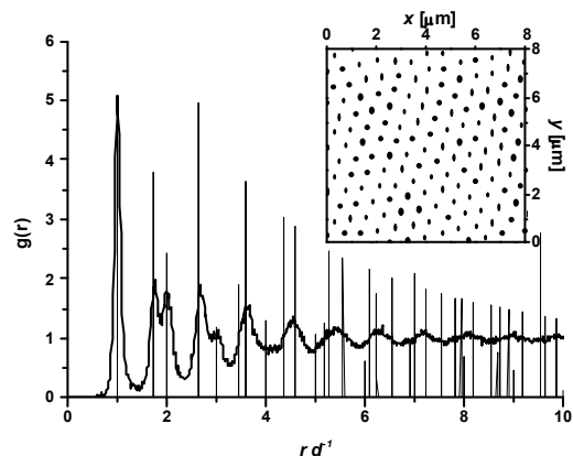
Figure 2. Example of a radial distribution function of charged core-shell microgel particles at the oil-water interface; d is the microgel diameter at the interface. Black lines indicate the peaks of a g(r) of an ideal hexagonally packed monolayer generated numerically. The inset highlights the centers of the particles as found from the automated particle location procedure.
