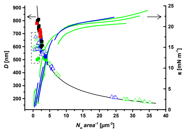
Figure 7. Nearest neighbor distance plotted versus particle density as extracted from FreSCa cryo-SEM (filled squares) and AFM images (open triangles). Green: uncharged core microgels; blue: charged core microgels; black: uncharged core-shell microgels; red: charged core-shell microgels. Compression isotherms of the uncharged (green) and the charged (blue) core microgels are also shown. The grey rectangle marks random particle arrangement and the black line shows the x^{-1/2} relation between D and N_p \text{ area}^{-1} .
