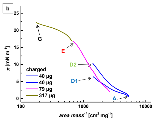
Figure 3. Compression isotherms of the a) uncharged and b) charged core microgel. The points where the microgel monolayer was transferred to a solid substrate are indicated by arrows. Same letters indicate similar amounts of spread microgels and the differently colored letters mark different particle arrangements. blue: random. green: hexagonal packing with voids. red: hexagonal packing. black: close hexagonal packing.
