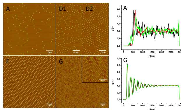
Figure 5. AFM images of the transferred microgel monolayer in the charged state at the points indicated in Figure 3b. The inset in G shows higher magnification of close packed microgels. The increasing ordering is represented by clearer oscillations in the radial distribution functions corresponding to images A and G. Each graph reports radial distribution functions from images at three different spots on the same substrate (red, green and black lines).
