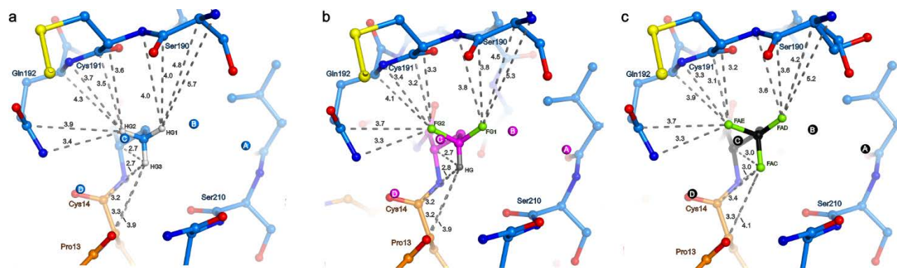
Figure 5 Distance analysis and top view of the unnatural side chain at position 15 of BPTI depicted in orange within the S1 binding pocket of \beta -trypsin drawn in blue. Values indicate the distance in Å between the individual hydrogen or fluorine atoms of the terminal ^{13}\text{C} of the side chain and the ten nearest enzyme atoms (clockwise, Gln192 NE , Gln192 CD , Gln192 CA , Gln192 N , Cys191 C , Cys191 CA , Cys191 N , Ser190 C , Ser190 CA , and Ser190 N ), as well as the five nearest BPTI atoms (from top to bottom, Xaa15 CA , Xaa15 N , Cys14 C , Cys14 CA , and Pro13 D ): a) Abu structure with side chain and structural waters A-D in light blue and the three ^{13}\text{C} hydrogen substituents HG1 (ABA HG1 ), HG2 (ABA HG2 ), and HG3 (ABA HG3 ) in light-gray; b) DfeGly structure with side chain and structural waters A-D in magenta, the two ^{13}\text{C} fluorine substituents FG1 (OBF FG1 ) and FG2 (OBF FG2 ) in green, and the single ^{13}\text{C} hydrogen substituent HG (OBF HG ) in gray; c) TfeGly structure with side chain and structural waters A-D in black and the three ^{13}\text{C} fluorine substituents FAD (3EG FAD ), FAE (3EG FAE ), and FAC (3EG FAC ) in green. Nitrogen atoms are shown in dark blue and oxygen atoms in red.
