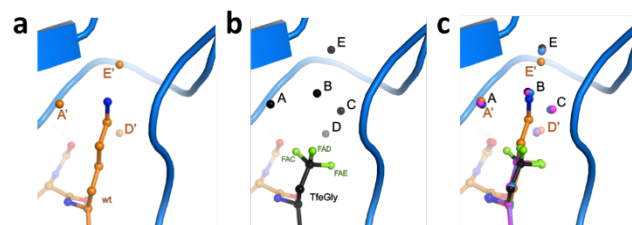
Figure 3 Structural context of the P1 side chain in the S1 binding pocket. \beta -Trypsin is shown in cartoon representation and the modified BPTI in stick representation a) Lys15 and structural water molecules A', D', and E', and b) Lys15TfeGly and structural water molecules A, B, C, D, and E, and c) superimposition of P1 side chains and structural water molecules.
