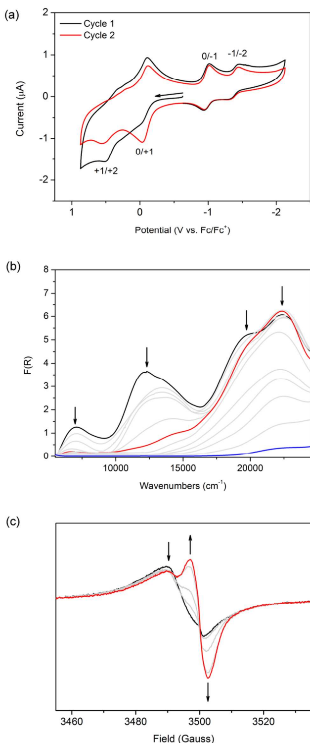
Figure 3. a) Solid state CV of [(Zn(DMF)_2)(TTFTC)(DPNI)] at 100\text{ mVs}^{-1} in a 0.1\text{ M } n\text{-Bu}_4\text{NPF}_6/\text{CH}_3\text{CN} electrolyte. The black line is the first cycle and the red line is the second cycle, after framework decomposition has occurred. Arrow indicates direction of forward scan. b) Solid state Vis-NIR SEC of [(Zn(DMF)_2)(TTFTC)(DPNI)] at 0\text{ V} (black), -0.75\text{ V} (red) and -1.00\text{ V} (blue). Grey lines show the spectral transition. c) Solid state EPR SEC of [(Zn(DMF)_2)(TTFTC)(DPNI)] at 0\text{ V} (black) and -0.80\text{ V} (red) in 0.1\text{ M } n\text{-Bu}_4\text{NPF}_6/\text{CH}_3\text{CN} . Grey lines show the spectral transition and the arrows show the direction of the spectral change.
