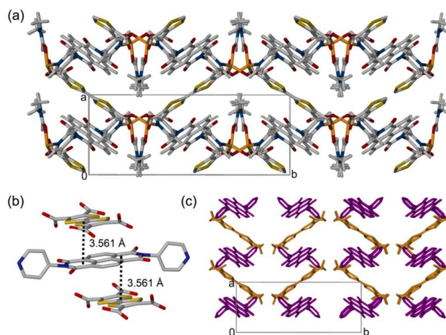
Figure 1. a) Crystal structure of [(\text{Zn}(\text{DMF})_2(\text{TTFTC})(\text{DPNI}))] viewed down the c -axis. b) Stacking of the TTFTC and DPNI ligands in the order \cdots\text{DADADA}\cdots at distances of 3.561 Å. Colour scheme: C, grey; O, red; N, blue; S, yellow; Zn, orange. c) Stacking of TTFTC (orange) and DPNI (purple) ligands in [(\text{Zn}(\text{DMF})_2(\text{TTFTC})(\text{DPNI}))] arranged in a herringbone pattern. Hydrogen atoms and solvent excluded for clarity.
