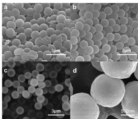
Figure 2. SEM images of (a) pure poly(MAA/EGDMA), (b) poly(MAA/EGDMA)/iron ions microspheres and (c and d) poly(MAA/EGDMA)/Fe 3 O 4 composite microcapsules at low magnification and high magnification.
