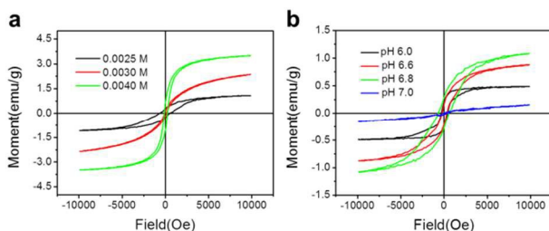
Figure 6. VSM magnetization curves of poly(MAA/EGDMA)/ \text{Fe}_3\text{O}_4 composite microspheres prepared in different (a) concentration of \text{FeCl}_2 (0.0025 M, 0.0030 M, 0.0040 M) and (b) pH values of aqueous solution during ion diffusion process.
