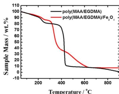
Figure 5. TGA curves of poly(MAA/EGDMA)/ \text{Fe}_3\text{O}_4 composite microcapsules with hollow structure and pure poly(MAA/EGDMA) hydrogel microspheres.
