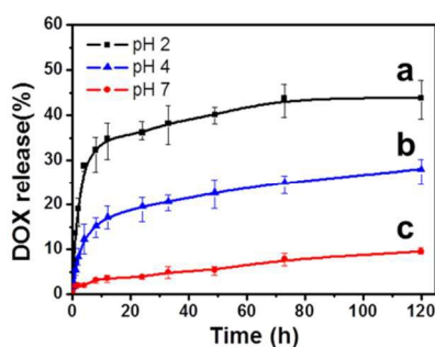
Figure 7. Doxorubicin cumulative release from the hollow poly(MAA/EGDMA)/Fe 3 O 4 composite microcapsules versus incubation time. Release profiles at different pH values (a) pH 2, (b) pH 4 and (c) pH 7.
