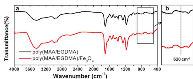
Figure 1. FT-IR spectra of (black) poly(MAA/EGDMA) and (red) poly(MAA/EGDMA)/Fe 3 O 4 composite microcapsules.
