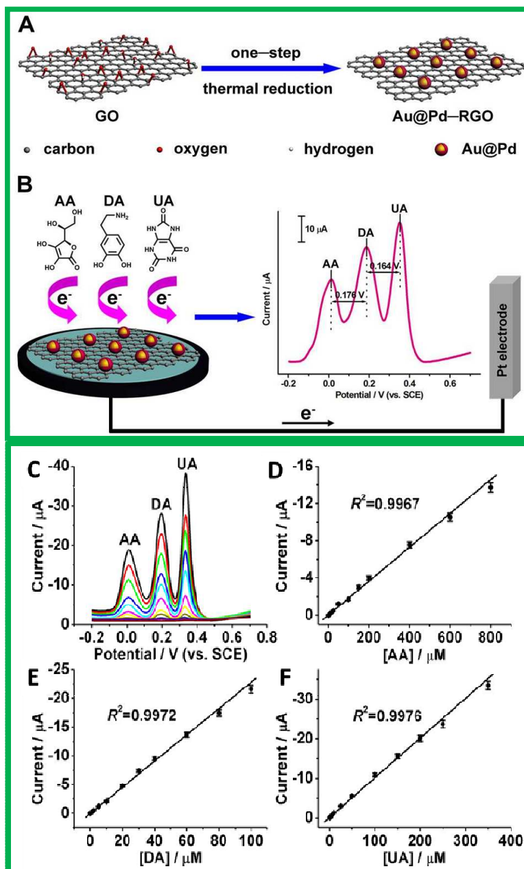
Figure 12. Schematic Illustration of preparations of (A) Au@Pd-RGO nanocomposites and (B) Au@Pd-RGO/GCE sensors for simultaneous determination of AA, DA, and UA. (C and E) From bottom to up 60 the concentrations of AA from 1 to 800 \mu\text{M} , DA from 0.1 to 100 \mu\text{M} , and UA from 0.1 to 350 \mu\text{M} . (D and F) Plots of the oxidation peak currents against the concentrations of AA, DA, and UA, respectively. The error bars represent standard deviations for five tests. Reprinted with permission from Ref 120, Copyrights (2014) Royal Society of Chemistry.
