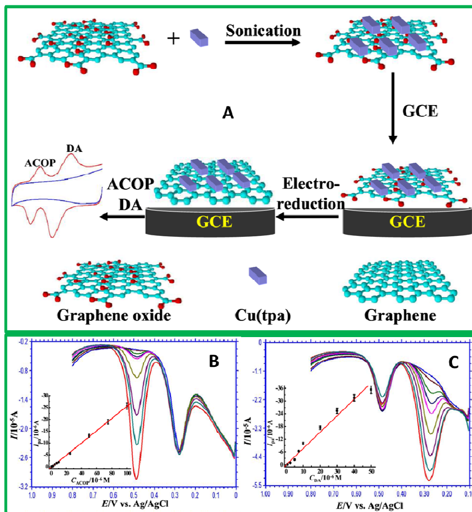
Figure 17. (A) Schematic illustration for the sonication-assisted preparation of Cu(tpa)-GO, and its application for the simultaneous determination of ACOP and DA. (B) DPVs of ACOP over a concentration range of 1.0 to 100 \mu\text{M} at Cu(tpa)-EGR/GCE in the presence of 20 \mu\text{M} DA in 0.1 M PBS (pH 5.0). (C) DPVs of DA over a concentration range of 1.0 to 50 \mu\text{M} at Cu(tpa)-EGR/GCE in the presence of 50 \mu\text{M} ACOP in 0.1 M PBS (pH 5.0). Insets in (B) and (C) are respectively the linear calibration plots of peak currents ( I_{pa} ) versus the concentration of ACOP ( C_{ACOP} ) and DA ( C_{DA} ). Reprinted with permission from Ref 162, Copyrights (2014) American Chemical Society.
