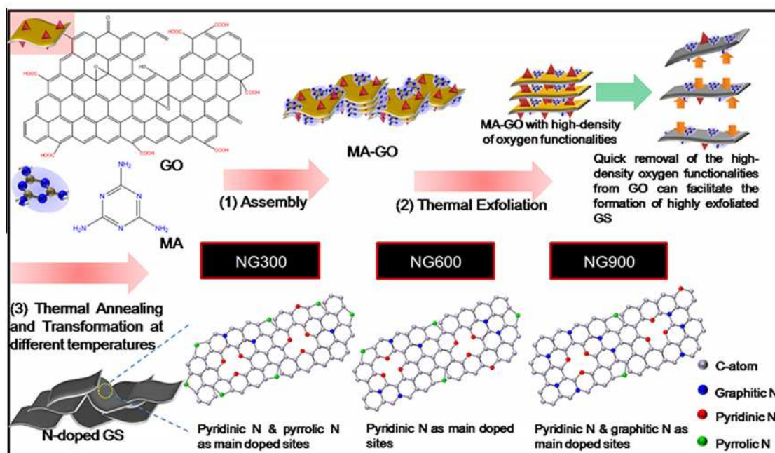
Figure 10. Schematic illustration for the synthesis of N-doped graphene with different allocation of nitrogen-doped configurations at different temperature. Reprinted with permission from Ref 88, Copyrights (2013) Elsevier Publications.
