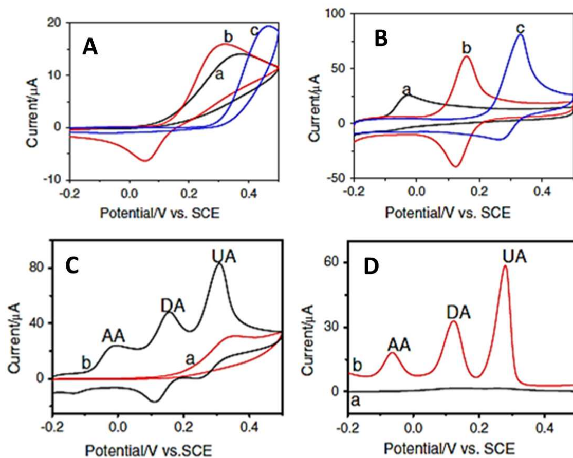
Figure 16. CVs obtained for 1 mM of AA (a), DA (b), and UA (c) individually in 0.1 M PBS at (A) bare GCE and (B) Lap/G/GCE. (C) CVs and (D) DPVs obtained for mixture of 1 mM AA, 0.7 mM DA, and 1 mM UA in 0.1 M PBS (pH 7.0) at bare GCE (a) and Lap/G/GCE (b). Reprinted with permission from Ref 158, Copyrights (2014) Springer.
