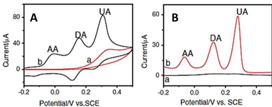
Figure 3: (A) Cyclic voltammograms and (B) DPV curves obtained for (a) bare GC and chemically modified electrode in the presence of DA, AA and UA.
