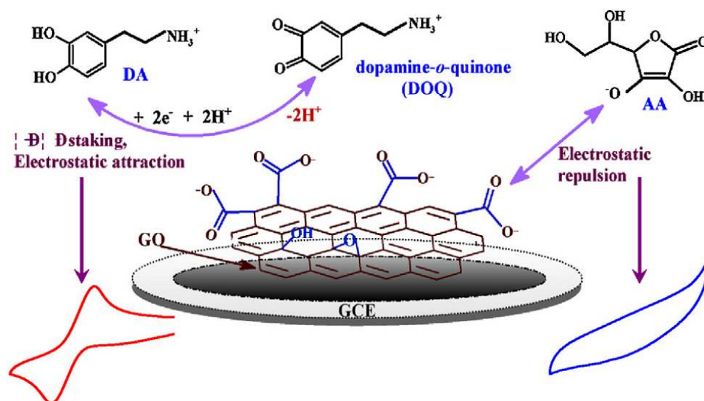
Figure 7. Different electrochemical pathway for DA and AA on the GO/GCE surface. Reprinted with permission from Ref 73, Copyrights (2013) Elsevier Publications.
