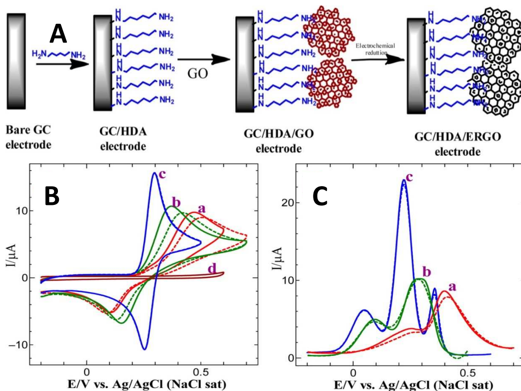
Figure 8. (A) Schematic illustration for the fabrication of ERGO modified GCE, (B) CVs obtained for the oxidation of 0.5 mM of DA at (a) bare GC, (b) GC/HDA/GO, and (c) GC/HDA/ERGO electrodes in 0.2 M PB solution (pH 5.5) at a scan rate of 50 mV s -1 . Solid line: first cycle; dotted line: eighth cycle. (C) DPVs obtained for the oxidations of each 0.5 mM of AA, DA, and UA at (a) bare GCE, (b) GC/HDA/GO, and (c) GC/HDA/ERGO electrodes in 0.2 M PB solution. Solid line: first cycle; dotted line: eighth cycle. Reprinted with permission from Ref 79, Copyrights (2013) American Chemical Society.
