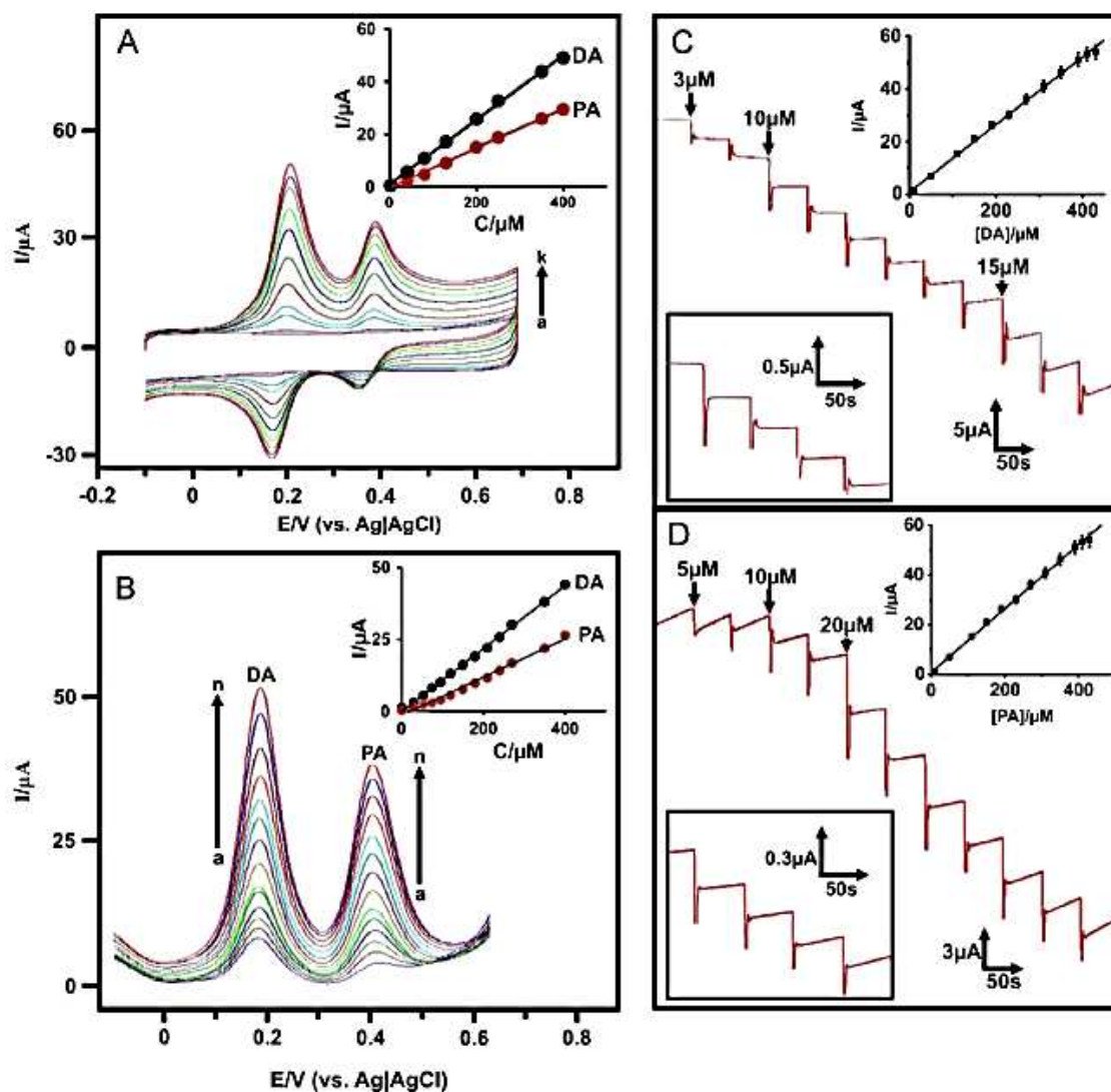
Figure 14. (A) CVs of MWCNT/GO nanocomposite film modified GCE (a) without and (b–k) with 200 nM–400 mM of DA and PA containing deoxygenated PBS at 50 mVs -1 scan rate. Inset plot shows the linear dependence of I_{pa} vs. [DA] and [PA]. (B) DPVs recorded at MWCNT/GO nanocomposite film modified GCE (a) without and (b–n) with 200 nM–400 mM of DA and PA containing deoxygenated PBS at 50 mVs -1 scan rate. Inset plot shows the linear dependence of I_{pa} vs. [DA] and [PA]. (C) Amperometric i–t response at MWCNT/GO nanocomposite film modified rotating disc GCE upon successive additions of 100 nmolL -1 –400 mM of DA into continuously stirred N 2 saturated PBS (pH = 7). Applied potential: 0.204V; inset (upper) shows the calibration curve of I_{pa} vs. [DA]. Inset (bottom) shows i–t response for each addition of 1 mM of DA. (D) Amperometric responses acquired under similar conditions for successive additions of 200 nM–400 mM of PA. Applied potential of 0.408 V; inset (upper) shows the calibration curve of I_{pa} vs. [PA]. Inset (bottom) shows i–t response for each addition of 1 mM of PA. Reprinted with permission from Ref 154, Copyrights (2013) Elsevier Publications.
