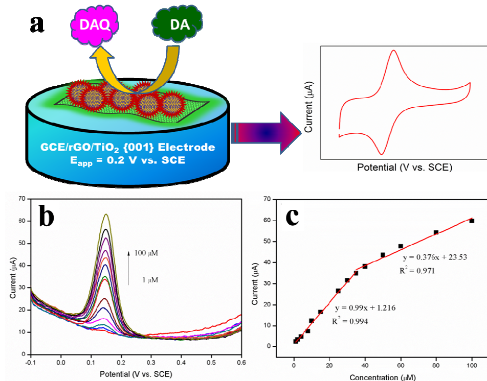
Figure 13. (a) Mechanism for the electrocatalytic oxidation of dopamine at rGO/TiO 2 {001} modified GCE. (b) DPV obtained for rGO/TiO 2 {001} modified GCEs during the addition of 1, 2, 4, 8, 10, 15, 25, 30, 35, 40, 50, 60, 80, and 100 μM DA into the 0.1 M PBS (pH = 6.5). (c) Calibration plot observed for the oxidation peak current vs. concentration of DA. Reprinted with permission from Ref 123, Copyrights (2014) Nature publishing Group.
