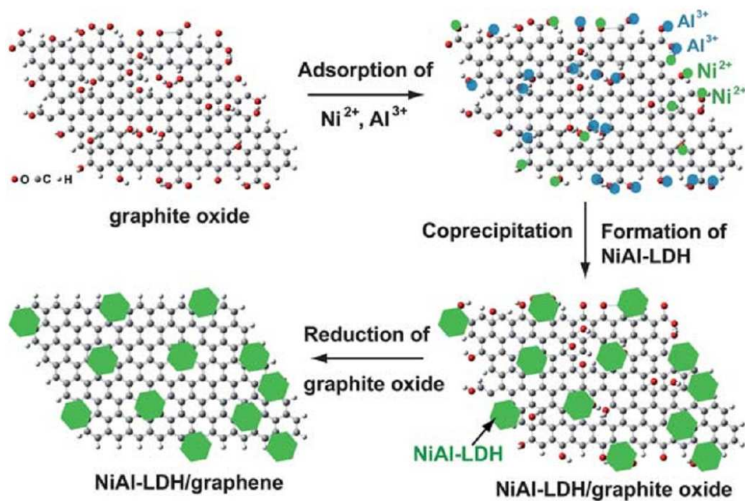
Figure 15. Schematic illustration of preparing the nanostructured NiAl-LDH/G composite Reprinted with permission from Ref 157, Copyrights (2011) Royal Society of Chemistry.
