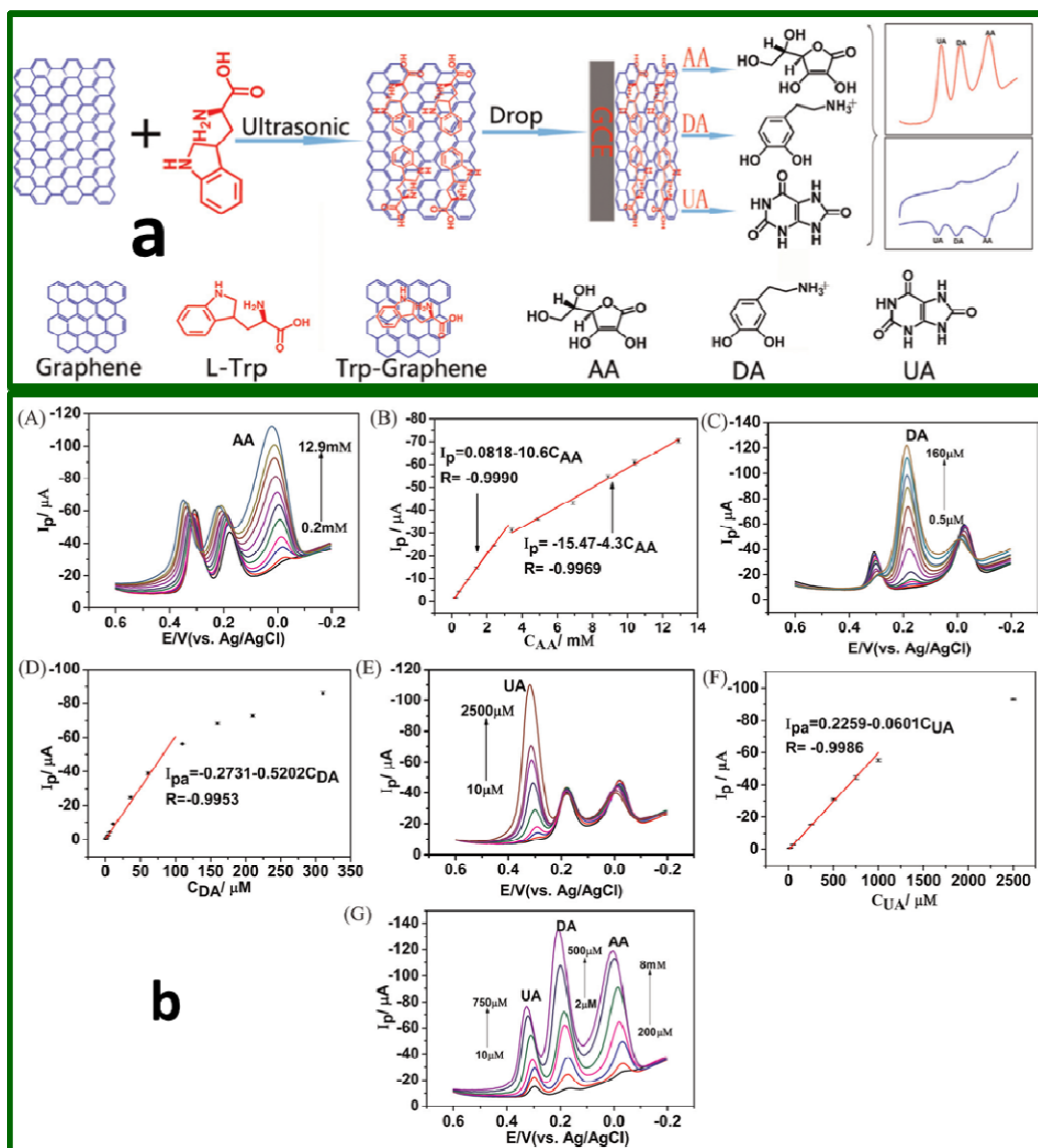
Figure 11. (a) Schematic diagram of the fabrication procedure Trp-GR, Trp-GR/GCE, and the Trp-GR/GCE was used direct determination of AA, DA, and UA. (b) DPVs of AA, DA, and UA at Trp-GR/GCE in 0.1 M PBS (pH 7.0) respectively, scan rate: 50 mV/s. (A) AA concentrations: 0.2, 0.4, 0.9, 1.4, 2.4, 3.4, 4.9, 6.9, 8.9, 10.4, and 12.9 mM in the presence of 50 mM DA and 0.5 mM UA; (B) the linear relationship between currents and AA concentration, (C) DA concentrations: 0.5, 1.0, 3.5, 6.0, 11, 36, 61, 110, 160, 210, and 310 mM in the presence of 8 mM AA and 100 mM UA; (D) the linear relationship between currents and DA concentration; (E) UA concentrations: 10, 20, 50, 100, 250, 500, 750, 1000, and 2500 mM in the presence of 50 mM DA and 8 mM AA; (F) the linear relationship between currents and UA concentration; (G) DPVs of different concentrations of AA, DA and UA (0.2, 0.45, 0.95, 2, 4, 6, 8 mM) for AA, (2, 7, 12, 50, 75, 200, and 500 mM) for DA and (10, 20, 50, 100, 250, 500, and 750 mM) for UA. Reprinted with permission from Ref 94, Copyrights (2014) Elsevier Publications.
