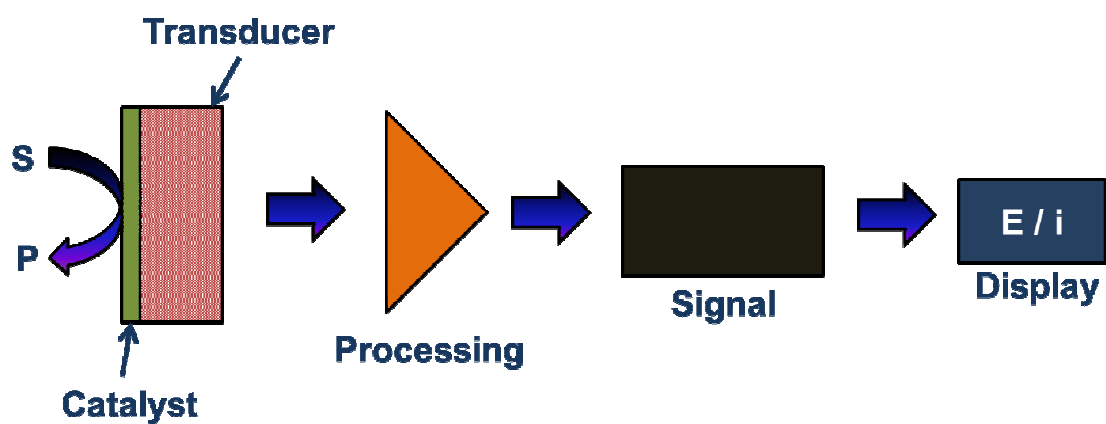
Figure 2: Principal stages in the operation of an electrochemical sensor.
