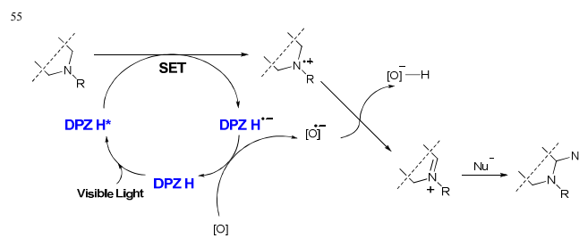
Fig. 6 Plausible mechanism of CDC reaction catalyzed by DPZ H
