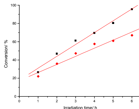
Fig. 5 Photocatalytic CDC reaction of 1a and 2a (or 2a-d 3 ) to give adduct 3a in the presence of DPZ derivative H ; reaction kinetics was monitored by using ^1H NMR spectroscopy; CH_3NO_2 (■), CD_3NO_2 (◆); DPZ H (0.05 \mu mol, 7.0 \mu L, 2.5 mg/mL), 1a (0.5 mmol), CH_3NO_2 or CD_3NO_2 (0.5 mL), reaction time: 6 h, 25 ^{\circ}C .
