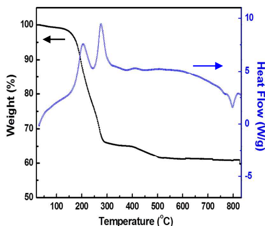
Fig. 1 TGA and DSC curves of BFO powder.
