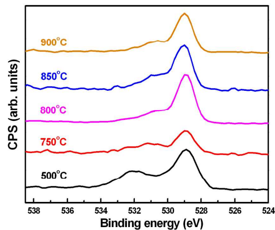
Fig. 5 XPS spectra of O1s binding energy of BFO samples prepared at different temperature.
