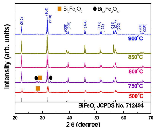
Fig. 2 XRD patterns of BFO samples prepared at different temperature.
