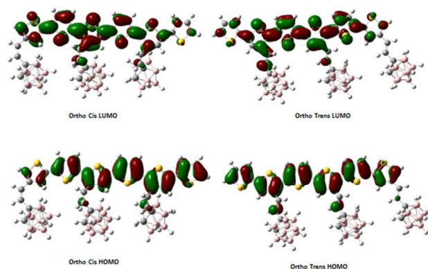
Figure 5. Visualised frontier molecular orbitals of ortholcis and ortholtrans polymers. Calculated in Gaussian09 with the B3LYP/6-31G* basis set.
