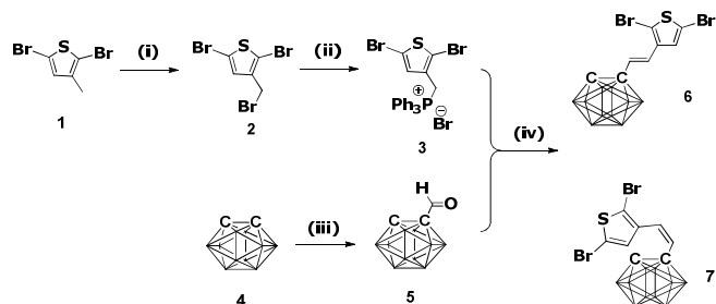
Scheme 1. Synthesis of ortho/cis and ortho/trans monomers. (i) NBS, benzoyl peroxide, 71%. (ii) Triphenylphosphine, hexane, 68%. (iii) n -BuLi then methyl formate, 66%. (iv) Potassium tert -butoxide, THF, 6% ( 6 ), 43% ( 7 ).
