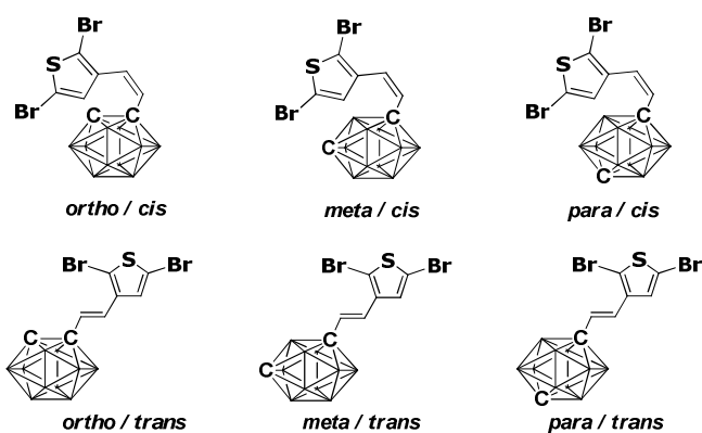
Figure 2. Structures of the six monomers investigated in this work. Non-labelled cage-vertices represent BH units, protons omitted for clarity
