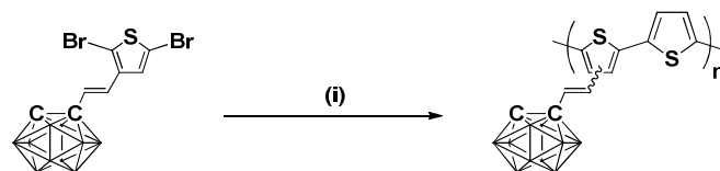
Scheme 2. Synthesis of ortho/trans polymer. (i) 2,5-bis(trimethylstannyl)thiophene, \text{Pd}_2(\text{dba})_3 , \text{P}(o\text{-tol})_3 , \mu\text{w} , 59%
