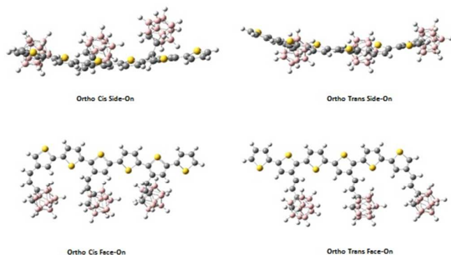
Figure 4. Energy minimised structures of ortholcis and ortholtrans polymers. Calculated in Gaussian09 with the B3LYP/6-31G* basis set.
