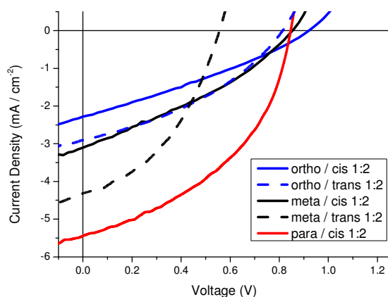
Figure 7. J-V curves of OPV devices with active layer produced from 1:2 wt% polymer:PC70BM blend ratio
