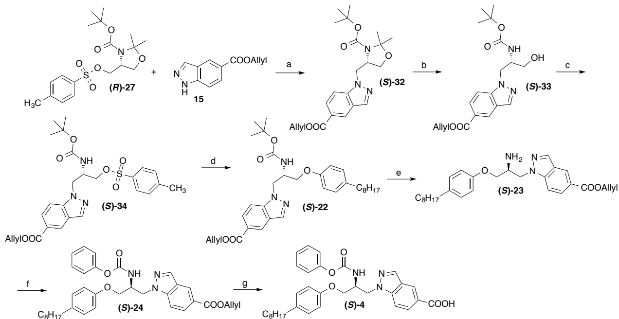
Scheme 4 Reagents and conditions: (a) NaH, DMF, 80^\circ\text{C} , 3 h; (b) 1. 1M HCl, THF, 70^\circ\text{C} , 3 h; 2. di- tert -butyl dicarbonate, triethylamine, methanol, room temp., 12 h; (c) p -toluenesulfonyl chloride, 4-dimethylaminopyridine, triethylamine, \text{CH}_2\text{Cl}_2 , room temp., 12 h; (d) 4-octylphenol, NaH, DMF, 80^\circ\text{C} , 3 h; (e) trifluoroacetic acid, \text{CH}_2\text{Cl}_2 , room temp., 2 h; (f) phenyl chloroformate, triethylamine, THF, room temp., 2 h; (g) tetrakis(triphenylphosphine)palladium(0), acetic acid, THF, room temp., 6 h.
