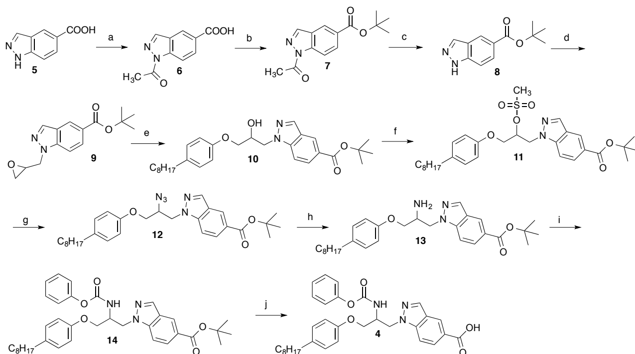
Scheme 1 Reagents and conditions: (a) Acetic anhydride, reflux, 2 h; (b) tert -butyl 2,2,2-trichloroacetimidate, cyclohexane, THF, BF 3 -etherate, room temp., 2 h; (c) 1M aqueous NaOH, ethanol, room temp., 1 h; (d) epichlorohydrin, powdered KOH, tetrabutylammonium bromide, room temp., 4 h; (e) 4-octylphenol, 4-dimethylaminopyridine, 120 °C, 2 h; (f) methanesulfonyl chloride, pyridine, room temp., 3.5 h; (g) trimethylsilyl azide, tetrabutylammonium fluoride, THF, reflux, 72 h; (h) Pd/C, H 2 , THF, room temperature, 6 h; (i) phenyl chloroformate, ethyl(diisopropyl)amine, THF, room temp., 45 min; (j) trifluoroacetic acid, CH 2 Cl 2 , room temp., 12 h.
