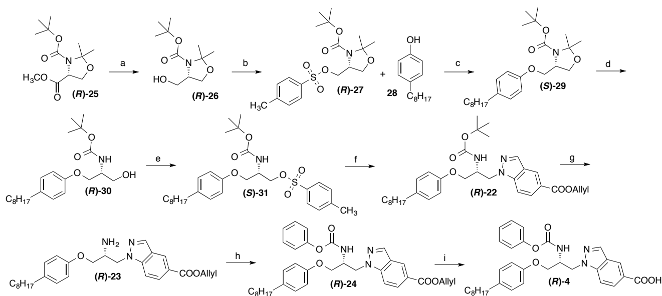
Scheme 3 Reagents and conditions: (a) \text{LiBH}_4 , THF, 0^\circ\text{C} , 3 h; (b) p -toluenesulfonyl chloride, 4-dimethylaminopyridine, triethylamine, \text{CH}_2\text{Cl}_2 , room temp., overnight; (c) NaH (dispersion in mineral oil), DMF, 70^\circ\text{C} , 3 h; (d) p -toluenesulfonic acid, room temp., 4 h; (e) p -toluenesulfonyl chloride, 4-dimethylaminopyridine, triethylamine, \text{CH}_2\text{Cl}_2 , room temp., overnight; (f) allyl indazole-5-carboxylate ( 15 ), NaH (dispersion in mineral oil), DMF, 80^\circ\text{C} , 3 h; (g) trifluoroacetic acid, \text{CH}_2\text{Cl}_2 , room temp., 2 h; (h) phenyl chloroformate, triethylamine, THF, room temp.; (i) tetrakis(triphenylphosphine)palladium(0), acetic acid, THF, room temp., 6 h.
