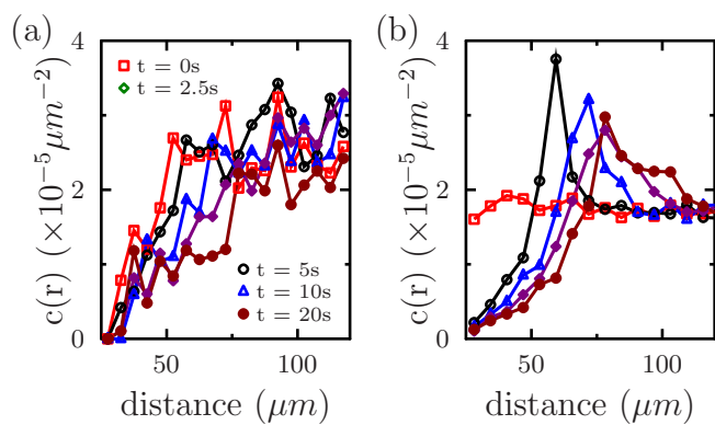
Fig. 6 Active swimmer (Au-Pt micromotor) density as a function of radial position and time: (a) experiment and (b) simulation.
