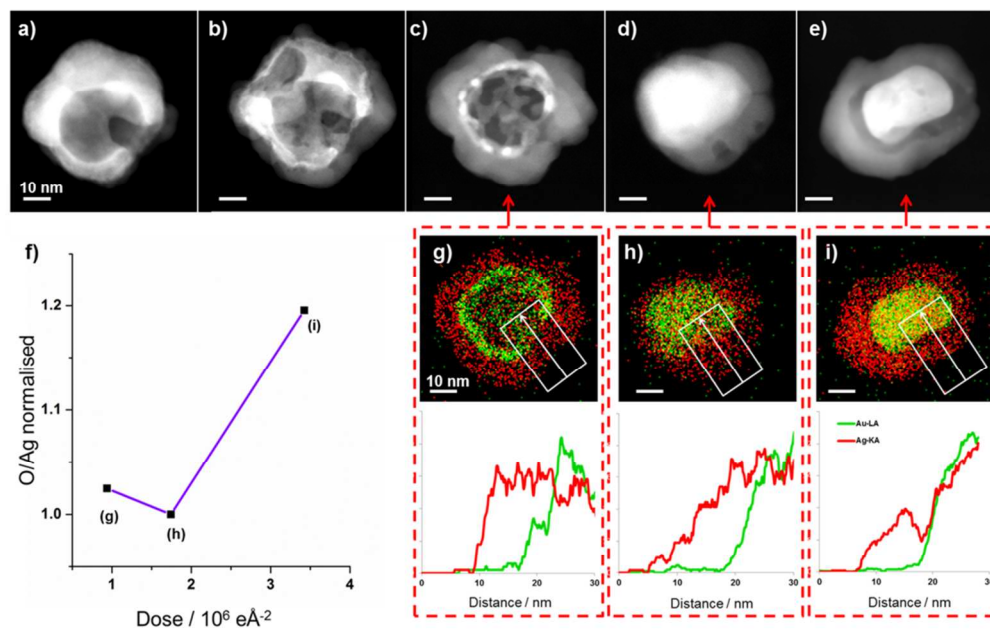
Fig. 5 (a-c) HAADF images showing an Ag-Au particle undergoing the beam induced oxidation reaction described previously, forming a hollow Au-Ag 2 O structure. Upon heating the hollow structure is lost (d), the shell shrinks and EDX data (f) shows a reduced oxygen signal suggesting some Ag 2 O is reduced to silver metal. The post heating, non-hollow, Au-core Ag-shell particle ((d) and (h)) undergoes a second beam induced oxidation reaction, in this reaction a yolk-shell (Au-yolk, Ag 2 O-shell) particle is formed ((e) and (i)).
