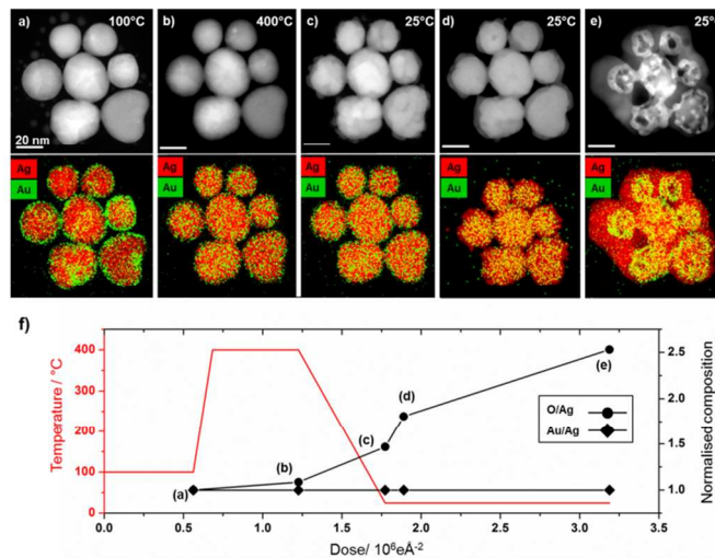
Fig. 4 Homogeneously alloyed AgAu particles, formed by in situ heating of Au surface segregated particles at room temperature (Video S3) but are unreactive at elevated temperature (400°C). (a-e) HAADF STEM images (top row) and simultaneously acquired EDX spectrum images (second row, Ag=red and Au=green). (a) At 100°C all particles initially show Au surface segregation, (b) upon heating to 400°C homogeneous alloying occurs but no oxidation reaction occurs, on quenching to room temperature a beam induced process of Ag 2 O shell growth and Au core-hollowing is observed (c-e). Heating to higher temperatures can lead to preferential loss of silver, localised melting and dramatic changes in morphology (Fig. S7).
