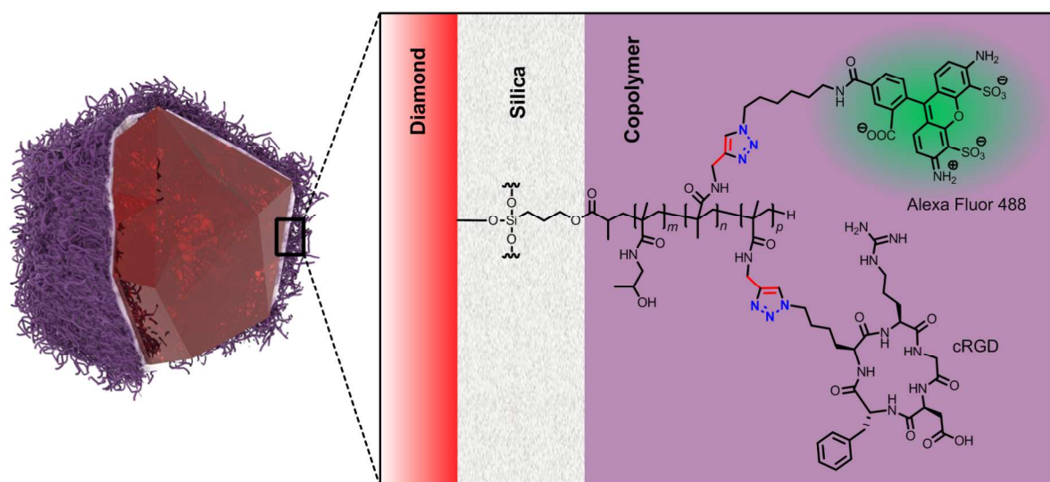
Scheme 1. Schematic structure of the fluorescent nanodiamond crystal coated with a biocompatible methacrylamide copolymer grown from an ultrathin silica shell. The copolymer bears the secondary fluorescent probe (Alexa Fluor 488) and targeting peptide (cRGD). Both molecules were stepwise attached via click chemistry, providing the conjugate marked as "FND-cRGD" (shown here in the scheme). Reaction with only the Alexa Fluor 488 provided the control particles marked in text as "FND".
