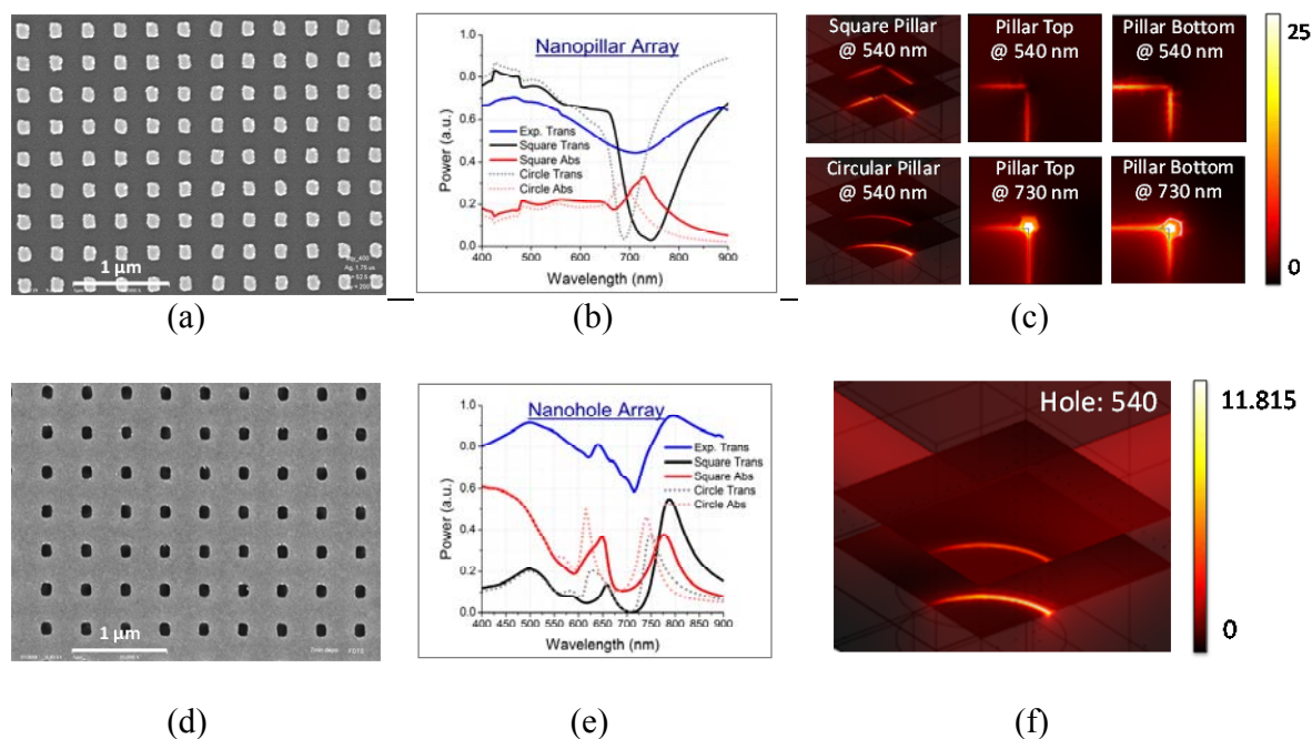
Figure 1. (a) SEM image of gold nanopillars array (320 nm pitch, 140 nm × 140 nm square) with 50 nm of gold and 5 nm of chromium. (b) Measured transmission spectrum (blue) of the fabricated nanopillar array in water, compared with the simulated (50 nm thickness of gold) transmission (black) and absorption (red) spectra for square (140 nm × 140 nm) and circular (140 nm in diameter) nanopillars. (c) Plasmonic field distributions at the wavelengths of 540 and 730 nm for the square and circular gold nanopillars. (d) SEM image of gold nanoholes (400 nm pitch, 140 nm × 140 nm square) with 50 nm of gold and 5 nm of chromium. (e) Measured transmission spectrum (blue) of fabricated nanoholes in water, compared with the simulated (50 nm of gold) transmission (black) and absorption (red) spectra for square (140 nm × 140 nm) and circular (140 nm in diameter) nanoholes. (f) Plasmonic field distributions at the wavelengths of 540 nm for circular gold nanoholes at the thicknesses of 50 nm. The light is illuminated from the gold nanoarray side in the experiments and simulations.
