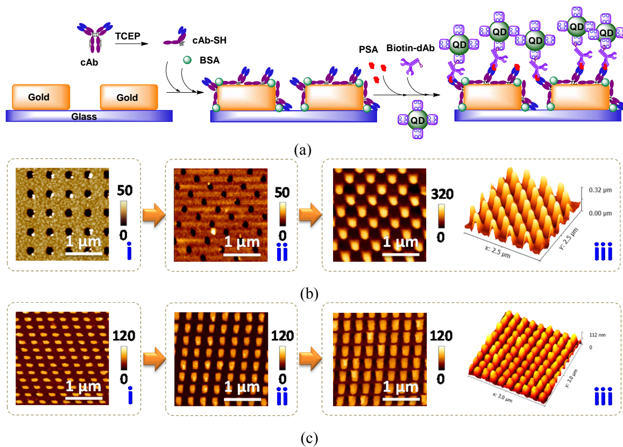
Figure 2. (a) Schematic illustration of sandwich immuno-assay for PSA detection on gold nanoarray, with QD as labeling fluorophore. i, blank gold nanoarray; ii, TCEP reduction of the cAb and self-assembly of the cAb-SH fragments on the gold nano-array, with BSA blocking; iii, PSA, biotin-dAb, and streptavidin conjugated QD-655 are applied sequentially to accomplish the sandwich immunoassay. (b) and (c) are AFM images of the layer-by-layer fabrication of the sandwich immunoassay on the gold nanohole and nanopillar arrays for i, ii and iii in (a), the concentration of PSA is 100 ng/ml.
