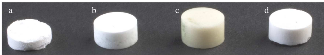
Figure 12. Micrographs of tablets made from (a) paracetamol Form I and (b to d) cocrystals of paracetamol with theophylline, naphthalene and oxalic acid respectively. Tablet (a) is poorly formed as a result of the inappropriate packing of the molecules in the lattice, whereas the cocrystal structures are amenable to deformation during tableting.(Karki et al., 2009a)
