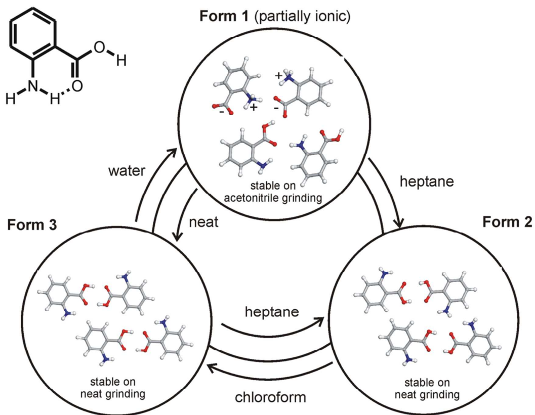
Figure 7. Schematic of the observed transformations between the three polymorphic forms of anthranilic acid with the pathways depending on the conditions under which mechanochemical treatment was performed.
