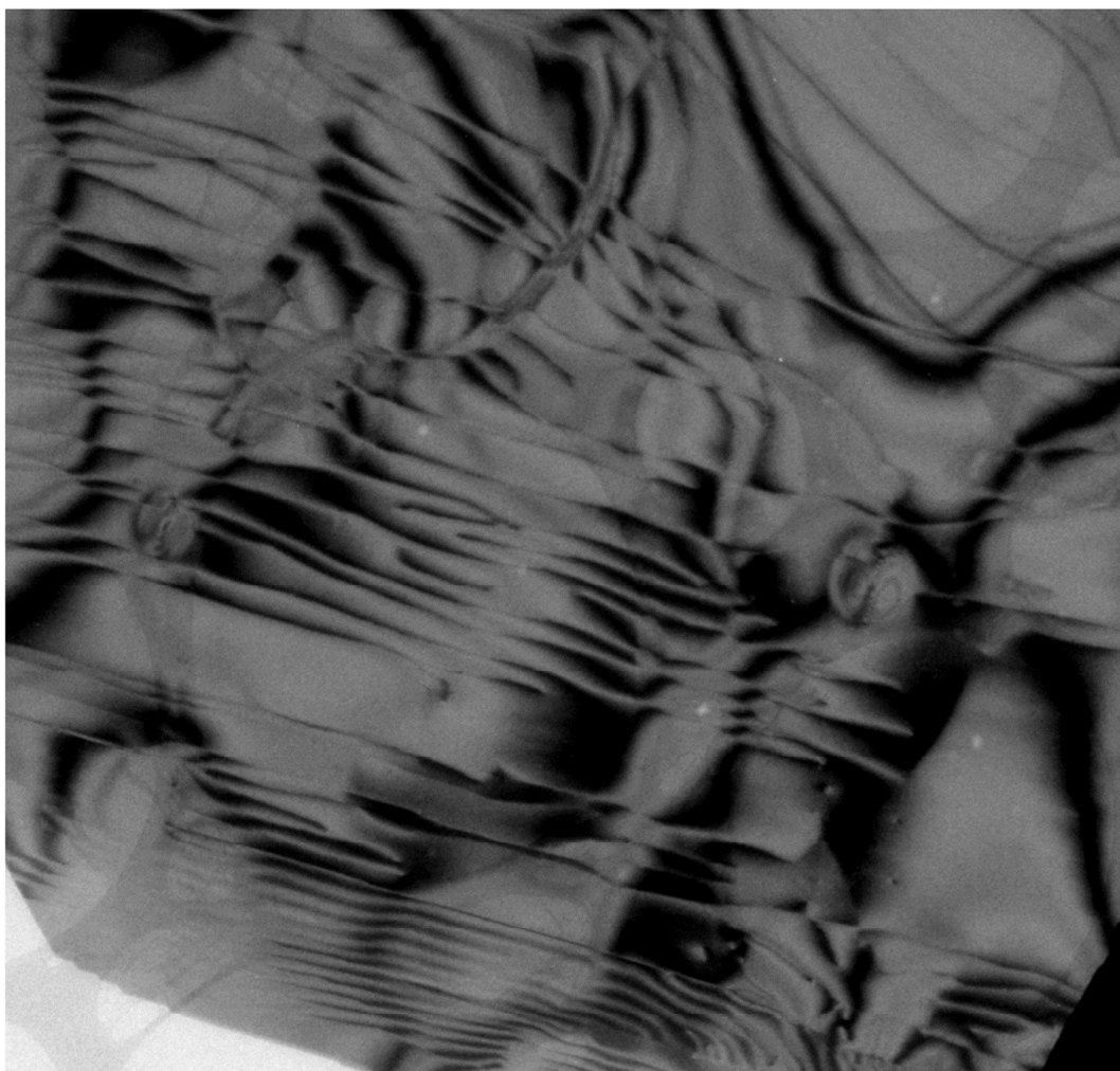
Figure 22. Extensive network of dislocations in a sample of theophylline as revealed by transmission electron microscopy. In general, such dislocations can result from the mechanical treatment of crystals.
