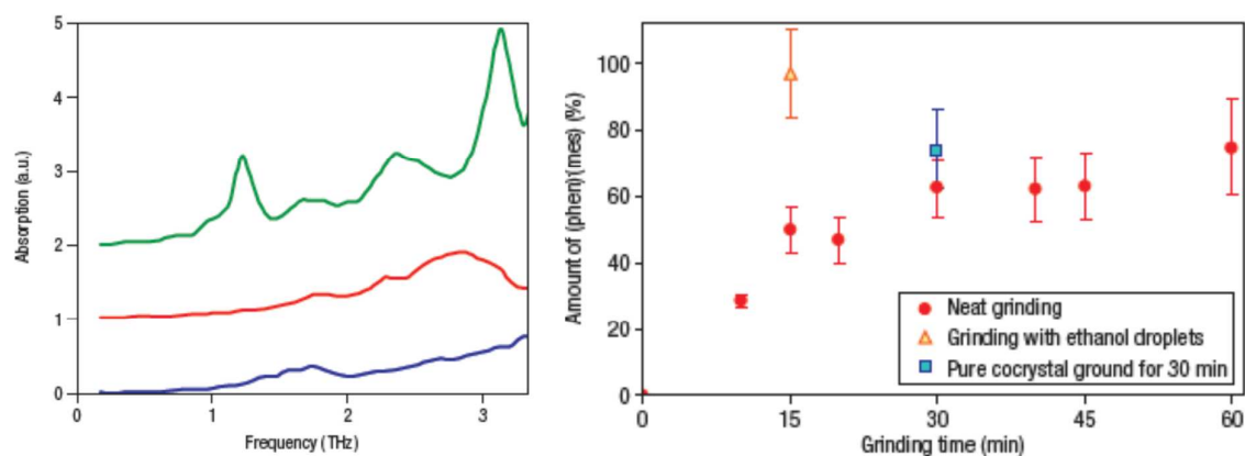
Figure 2. (a) Terahertz spectra obtained from (top to bottom): a 1:1 mesaconic acid-phenazine cocrystal; mesaconic acid; phenazine. (b) Analysis (ex situ) of the extent of formation of the cocrystal from a mixture of phenazine and mesaconic acid, as a function of neat grinding time, as measured using the characteristic cocrystal band at 1.1 THz (red circles). The orange triangle, by comparison, shows close to 100% conversion in 15 minutes as a result of the presence of liquid in a LAG experiment. The blue square represents the percentage of a cocrystal sample that remained crystalline during dry grinding. (Nguyen et al., 2007)
