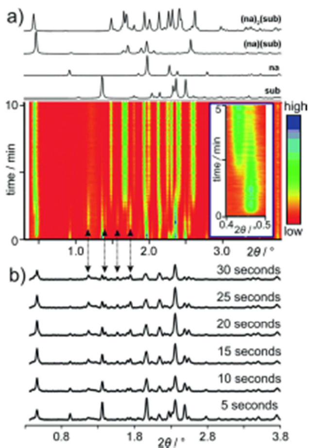
Figure 19. In situ synchrotron data for the milling of suberic acid and nicotinamide in a 2:1 ratio. (a) The PXRD patterns of the phases expected to be formed during milling along with the data obtained as a function of time. The inset shows the particular region at 0.4 to 0.5 degrees two-theta showing the initial formation of the 1:1 cocrystal followed by the 2:1 product. (b) The specific reflections indicated by arrows indicate the intermediate phase which is not detected by conventional ex situ studies. (Halasz et al., 2013)
