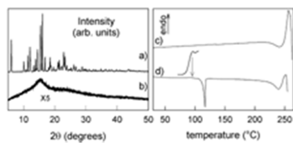
Figure 5. Demonstration of the amorphisation of trehalose as a result of milling at room temperature within a high energy planetary micro-mill. (a and b) PXRD and (c and d) DSC data before and after milling. (Descamps et al., 2007)
