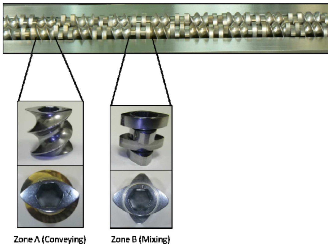
Figure 4. Typical twin extrusion configuration used for the formation of cocrystals. The conveying and mixing zones are shown. Typical output rate is approximately 0.5 \text{ g}\cdot\text{min}^{-1} . PXRD suggests comparable properties for the product to that obtained by conventional solution growth. The possibility of simultaneously blending the cocrystal product within a polymer matrix is an important additional advantage of the method.(Daurio et al., 2011)
