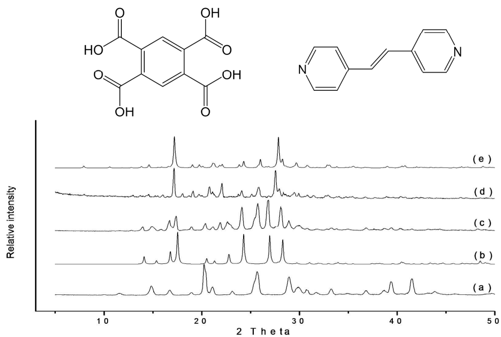
Figure 15. Demonstration of the enhanced kinetics of cocystal formation upon addition of a few drops of methanol to the grinding jar. PXRD patterns for (a) tetracarboxylic acid, (b) bipyrindyl, (c) outcome of neat grinding for 60 minutes (as the sum of the reactants), (d) the product obtained when a few drops of methanol are added and (e) the simulated pattern for the cocystal.
