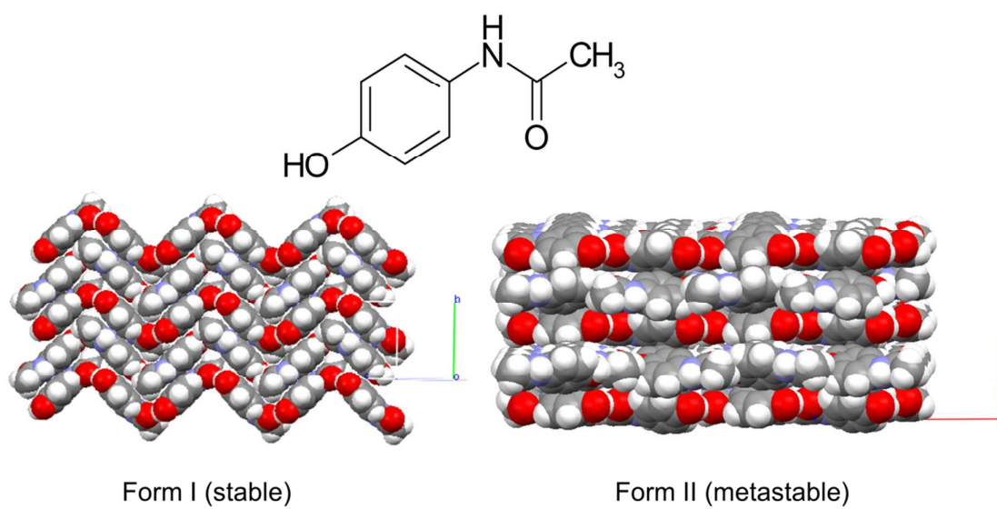
Figure 11. Packing diagrams for Form I and Form II paracetamol. Whilst Form I is the stable phase it does not compress well during tablet formation. The metastable Form II has a layered structure more appropriate for compression, but readily transforms to Form I.
