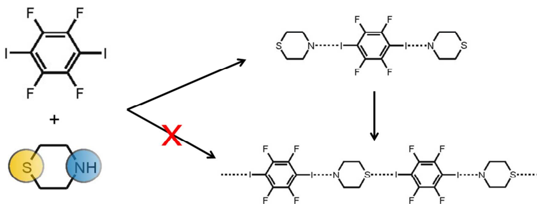
Figure 18. The discrete trimer units and extended polymer chains (based on halogen bond interactions) believed to be formed during the LAG reaction. When the strength of the halogen bond is weak the product is limited to the trimer unit.
