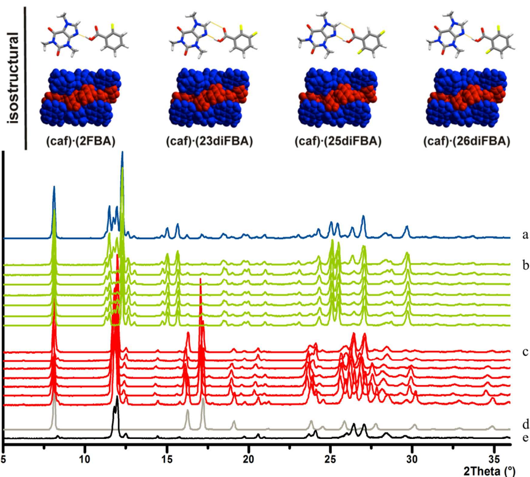
Figure 17. Top. Isostructural cocrystals of caffeine with various fluorobenzoic acids which have similar packing to that predicted for the likely structure for the caffeine-benzoic acid cocrystal. Bottom. PXRD traces of (a) product without deliberate addition of seeds, but prepared in an environment where the caffeine-benzoic acid cocrystal had previously been obtained, (b) products of various seeding reactions, (c) products of various unseeded reactions, (d) benzoic acid and (e) caffeine. The main points to note include the similarity of the patterns in (a) and (b) and that those in (c) are a simple combination of the starting materials in (d) and (e). (Bučar et al., 2013a)
