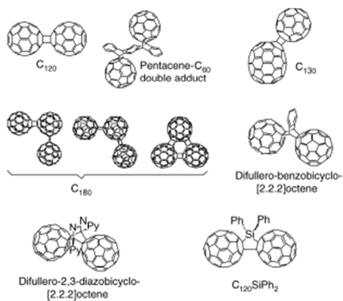
Figure 1. Various fullerene complexes generated by mechanochemical treatment of C_{60} . These products were not obtained from solution reactions. (Braga and Grepioni, 2004)
