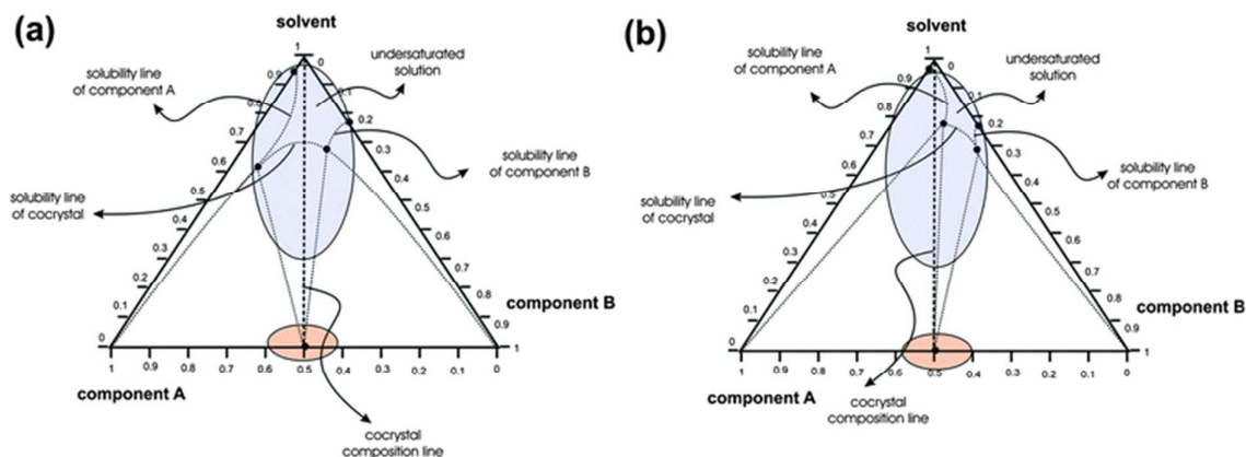
Figure 16. Typical three-component phase diagrams contrasting (a) congruent and (b) incongruent solubility profiles indicating the difficulties which will arise during conventional evaporative solution growth crystallisation. The fact that LAG experiments, with minimal amounts of solvent present, places the system close to the cocystal composition illustrates the ability of LAG to form cocystals when solids of very different solubility are investigated. (Delori et al., 2012)
