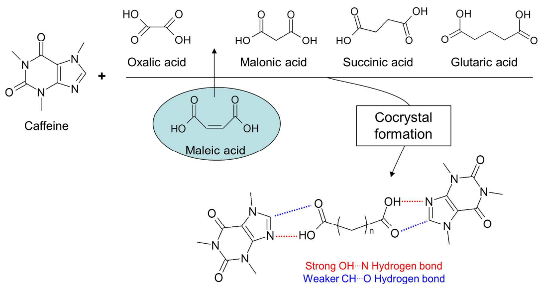
Figure 10. Supramolecular synthon approach used in the design of cocryystals of caffeine with various dicarboxylic acids. This approach lead to a variety of solid forms of caffeine which could be tested for stability under conditions of high humidity. Mechanochemistry was the technique used to both screen for cocryystal formation and also prepare powders for humidity assessment.
