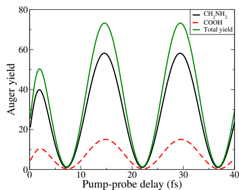
Fig. 6 Auger profile as a function of pump-probe delay. The Auger profile shows the same modulation of signal as is seen in the survival probability of the initial states, which is associated with the energy difference between the two states |a\rangle and |b\rangle that make up the superposition.
