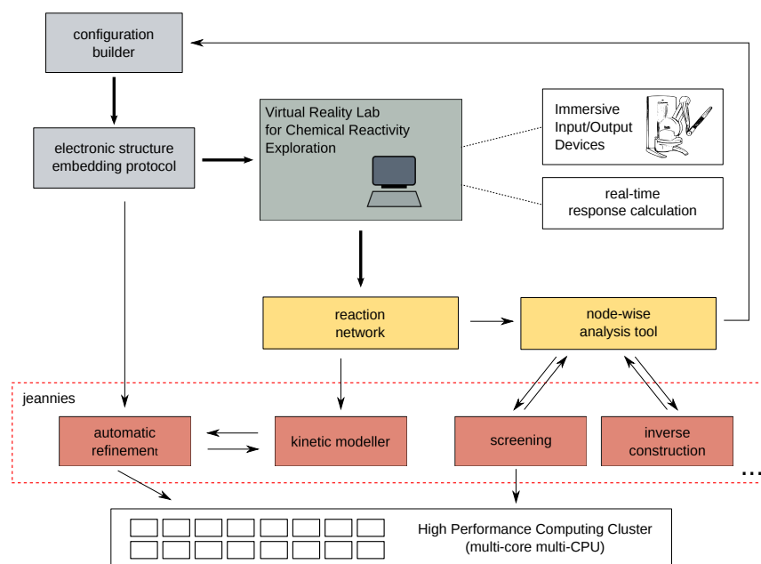
Fig. 1 Design of a virtual environment for the investigation of reaction mechanisms and networks.
