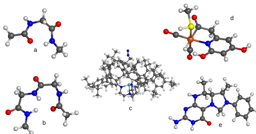
Fig. 2 Molecular systems used for the timings. (a) Alanine dimer, (b) Alanine trimer, (c) Schrock trisamidoamine Mo complex with N 2 , (d) FeGP, (e) model for HMPT. Structures a, b, e have been obtained from a DFTBA 49,50 optimisation in Gaussian 09 51 Rev. d.01. Structure d has been taken from Ref. 52, structure c from Ref. 8.
