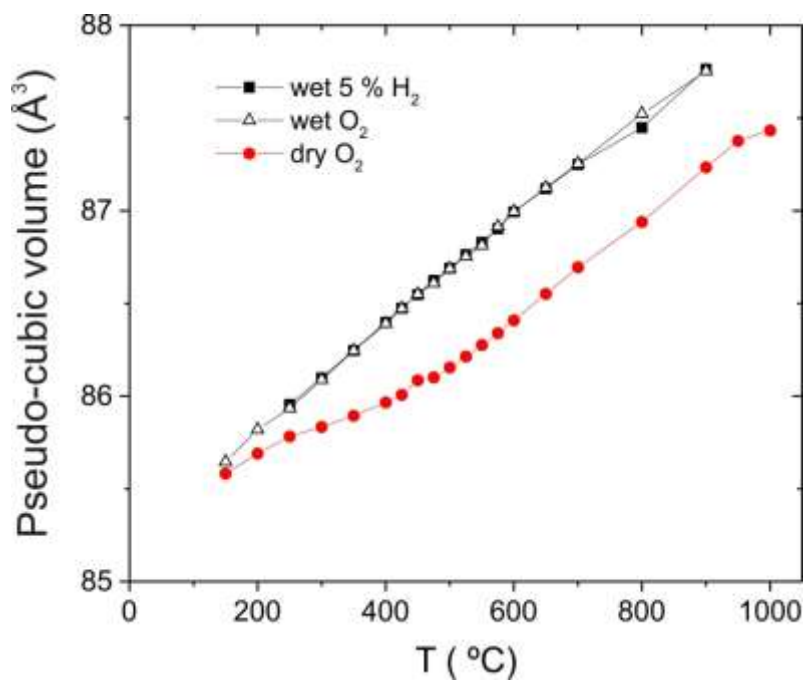
Figure 7. The pseudo-cubic cell volume of BaCe 0.8 Y 0.2 O 3-δ in O 2 , O 2 +D 2 O (g) and 5% H 2 /95 % Ar+D 2 O (g) .
