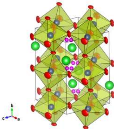
Figure 11. Possible deuteron site (purple) for the Imma structure of BCY20 at 450 °C.
