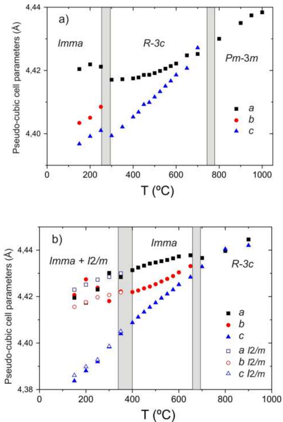
Figure 6. Phase stability fields and pseudo-cubic lattice parameters of \text{BaCe}_{0.8}\text{Y}_{0.2}\text{O}_{3-\delta} in (a) dry \text{O}_2 and (b) \text{O}_2 + \text{D}_2\text{O}(\text{g}) .
