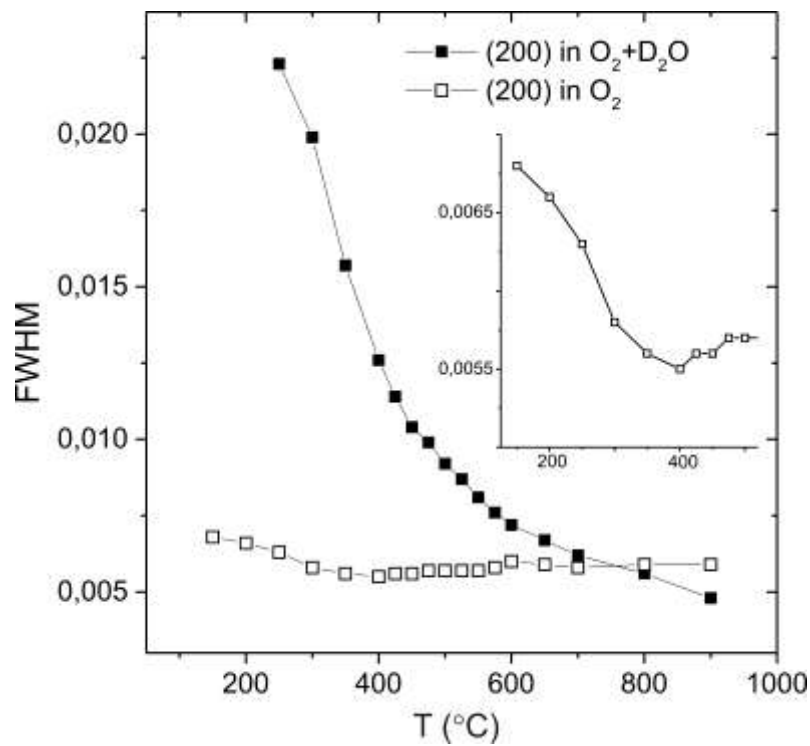
Figure 2. Analysis of the FWHM of the intensity in the region of the cubic (200) reflection in O 2 and O 2 +D 2 O (g) atmospheres. Inset shows a close-up of the dry O 2 behaviour revealing broadening linked to the appearance of the Imma phase at T < 300 °C.
