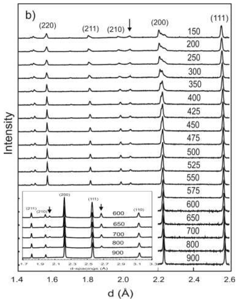
Figure 1. Neutron diffraction patterns from the high-resolution backscattering detector of HRPD collected in dry O_2 flow (a) and in O_2+D_2O_{(g)} flow (b) from 900 to 150 °C. Pseudo-cubic Miller indices are labelled. The insets show patterns from the 90^\circ detector bank where new peaks marked with arrows appear linked to the R\text{-}3c structure.
