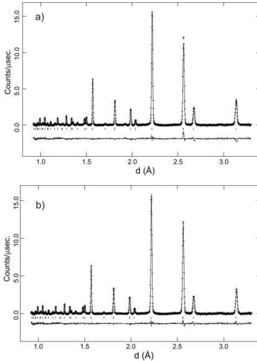
Figure 8. (a) Rietveld fit achieved, with no deuteron position defined, to the 700 °C, O 2 +D 2 O(g) data for BaCe 0.8 Y 0.2 O 3-δ . (b) Rietveld fit achieved with the deuteron position defined at the 36f site to the same data. Crosses are observed data, lines are the calculated profile and difference plot. Tick marks indicate reflection positions for the R -3 c structural model.
