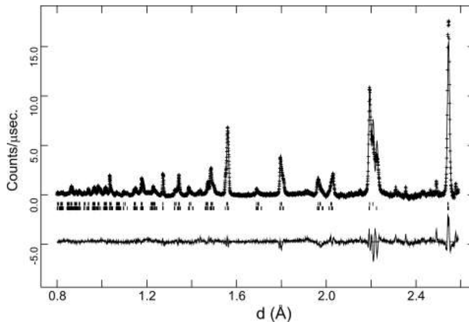
Figure 5. Rietveld fit to the high-resolution data collected at 150 °C in O 2 +D 2 O (g) for BaCe 0.8 Y 0.2 O 3-δ . Crosses are observed data, lines are the calculated profile and difference plot. Upper and lower tick marks indicate reflection positions for the Imma and I2/m structural models respectively.
