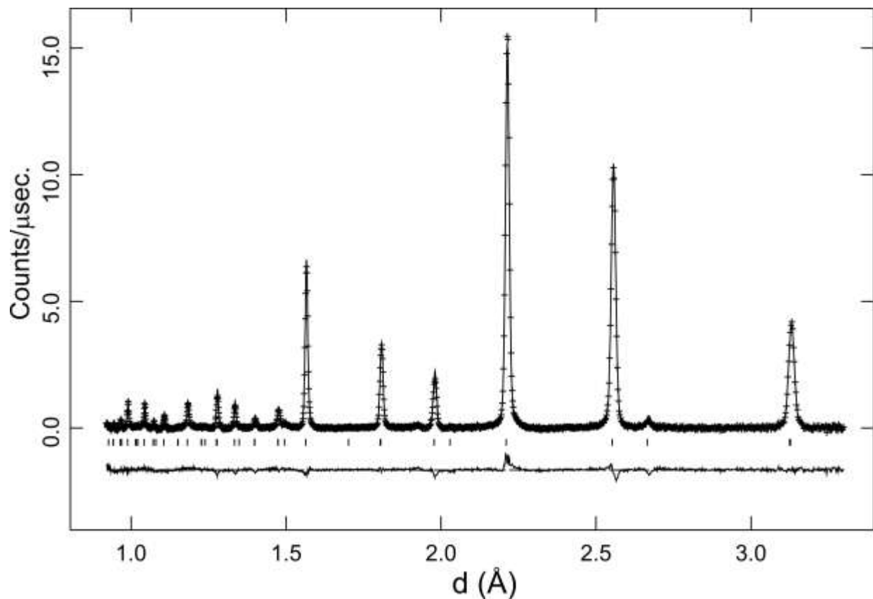
Figure 3. Rietveld fit to the 90 ° angle detector bank data for \text{BaCe}_{0.8}\text{Y}_{0.2}\text{O}_{3.8} at 700 °C in \text{O}_2 . Crosses are observed data, lines are the calculated profile and difference plot. Tick marks indicate reflection positions for the R\text{-}3c structural model.
