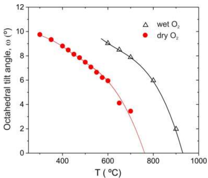
Figure 4. Antiphase octahedral tilt angle of BCY20 extracted from R-3c refinements of the data collected in dry O 2 and O 2 +D 2 O (g) . Lines are included as guides to the eye only.
