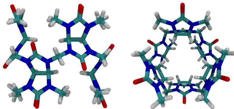
Fig. 7. Side and top views of bambus[6]uril; see Figure 4 for the molecular structure.
