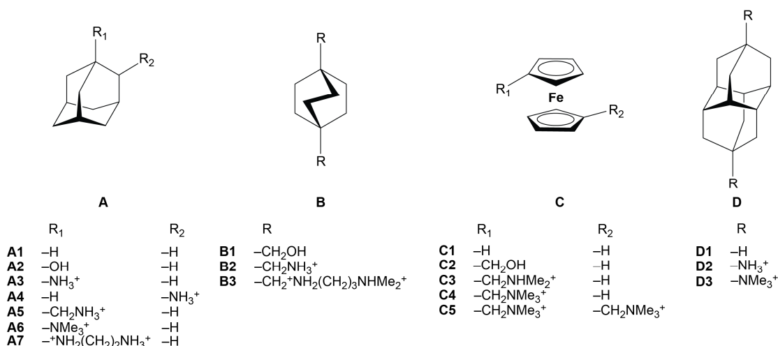
Fig. 17. Molecular structures of high-affinity binders to CB7.
