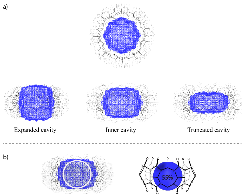
Fig. 11. a) Top and side views of different cavity definitions, taken for ref. 8. Copyright © 2011 WILEY-VCH Verlag GmbH & Co. KGaA, Weinheim. b) Schematic illustration of an ideal cavity filling of 55% by encapsulation of a spherical guest.
