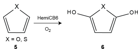
Scheme 5. Aerobic oxidation of heterocyclic ( 5 ) mediated by hemicucurbit[6]uril.
