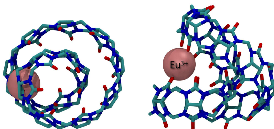
Fig. 3. Top (left) and side (right) view of the X-ray crystal structure of the Eu 3+ CB 14 complex; hydrogen atoms removed for clarity.
