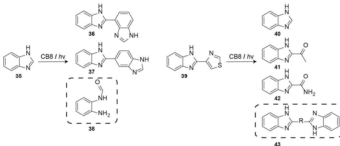
Scheme 6. CB8 modulates the phototransformation of a) benzimidazole ( 35 ) and b) thiabendazole ( 39 ); marked products were observed only in the presence of CB8.
