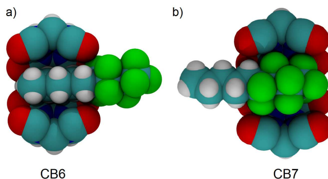
Fig. 15. Representative structures illustrating the residue-selective binding of 1-(perfluorbutyl)pentane with a) CB6 and b) CB7.
