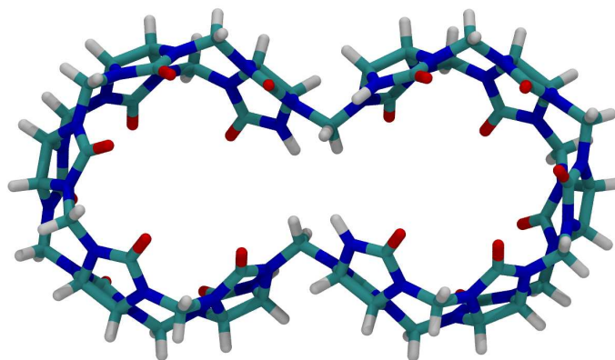
Fig. 8. Top view of bis-nor-seco-CB10; see Figure 4 for the molecular structure.
