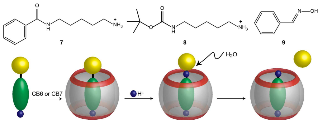
Fig. 19. Acidic hydrolysis of an amide ( N -benzoyl-cadaverine, 7 ), a carbamate (mono- N -( tert -butoxy)carbonyl cadaverine, 8 ), and an oxime (benzaldoxime, 9 ) mediated by CBn . 166
