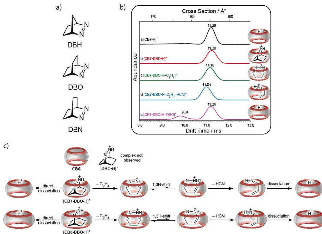
Fig. 23. A) Chemical structures of the bicyclic azoalkanes. b) Ion mobilitygrams of different CB7 complexes. c) Reaction and dissociation pathways of the inclusion complex of DBO inside CB7.
