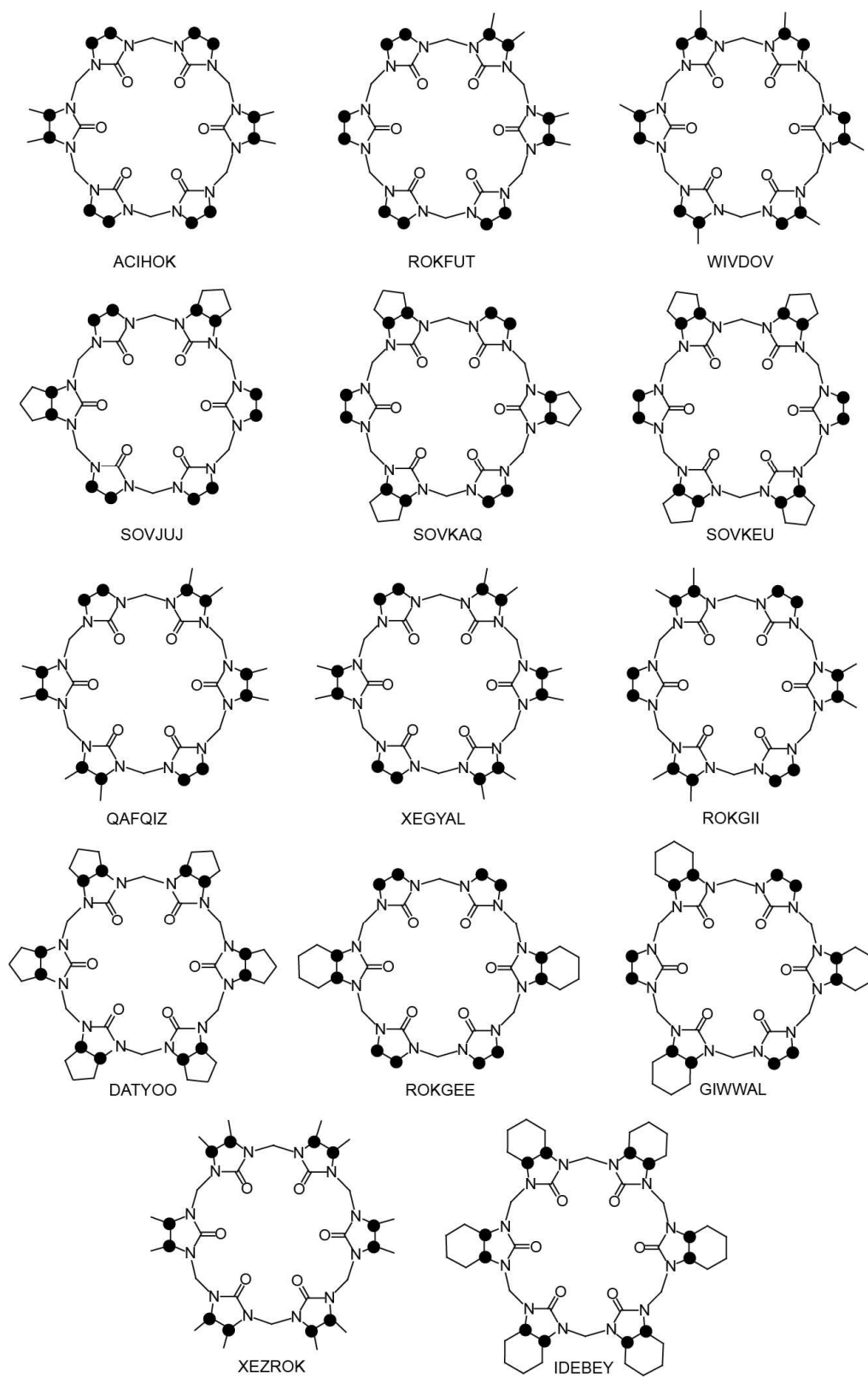
Fig. 5. Top views of the reported XRD molecular structures of substituted CB6 derivatives (codes taken from the CCDC data base); see Table 1 for references; dots mark connection points to the second identical half of the symmetric structures.
