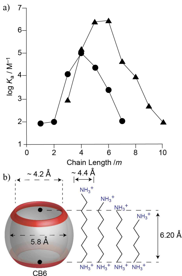
Fig. 14. a) Relationship between the binding constant ( \log K_a ) versus chain length m for \text{H}(\text{CH}_2)_m\text{NH}_3^+ (●) and ^+\text{H}_3\text{N}(\text{CH}_2)_m\text{NH}_3^+ (▲). b) Dimensional comparison between CB6 and various \alpha,\omega -alkane diammonium ions.
