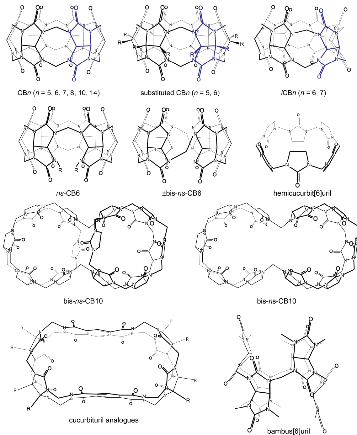
Fig. 4. Molecular structures of different cucurbit[ n ]urils and related cyclic macrocycles; colored parts indicate repetition units varying with n .
