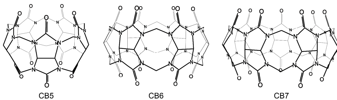
Fig. 1. Molecular structures of the three smallest CB n homologues.
