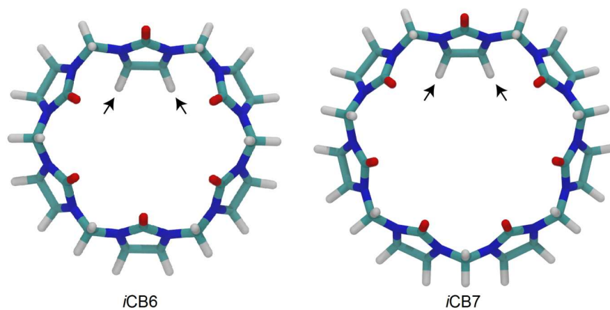
Fig. 6. Inverted cucurbiturils, iCBn ( n = 6 and 7 ); arrows indicate inverted glycoluril units; see Figure 4 for the molecular structure.
