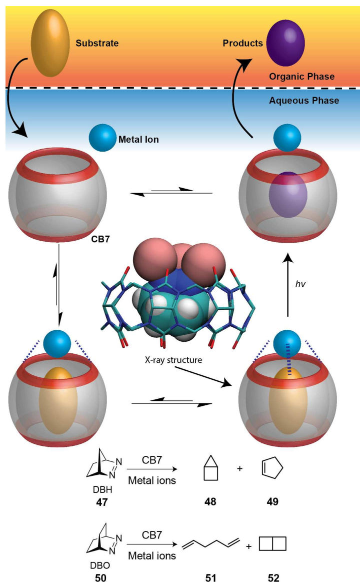
Fig. 22. Chemoselective photoreactions of bicyclic azoalkanes ( 54 and 57 ) mediated by CB7 in the presence of transition metal ions. 206
