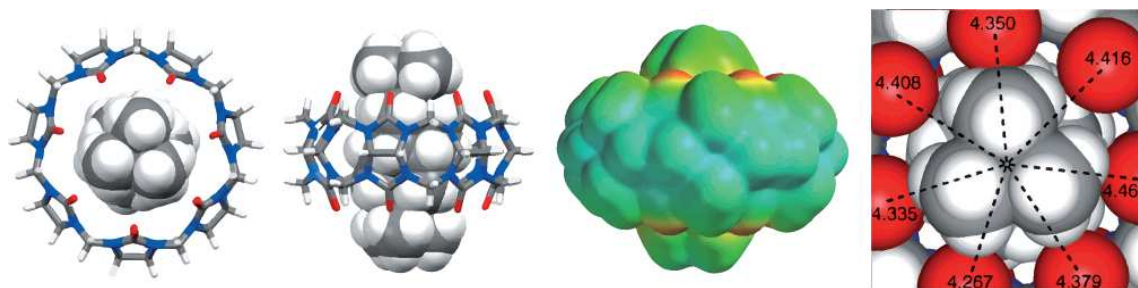
Fig. 18. Representations of the X-ray crystal structure of the CB7•diamantane diammonium complex. Taken from ref. 137. Copyright © 2014 WILEY-VCH Verlag GmbH & Co. KGaA, Weinheim.
