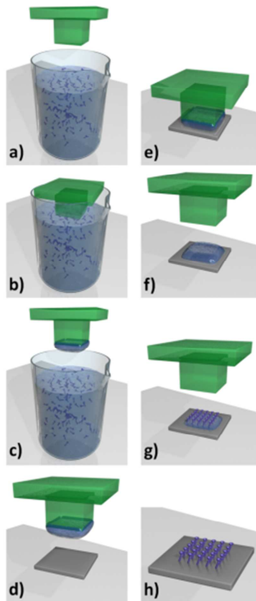
Fig. 4 Surface functionalisation by microcontact printing ( \mu\text{CP} ). a-c) A lithographed stamp is inked with solution containing the functional units. d-f) The solution is then transferred to the substrate by placing the stamp in contact with the substrate. g-h) the solvent is then allowed to evaporate, producing the self-assembled monolayer (SAM). Video animation provided as ESI.
