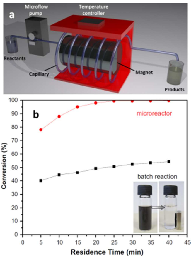
Fig. 25 (a) Schematic of the reactor used for the condensation reaction between benzaldehyde and ethyl cyanacetate using Fe 3 O 4 @ZIF-8 MFC immobilized along the tube with a magnet; (b) results of the catalytic conversion. The inset shows the fast collection of the composite with an external magnet. From Zhang et al. 216
