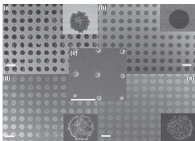
Fig. 6 SEM images of ZIF-8 crystals grown by LPE on gold substrates patterned with SAM. a) ZIF-8 dots grown on ODT and MHA background. b) ZIF-8 grown in methanolic solution to form a negative pattern. c) Single ZIF-8 crystals grown on ODT and MHA background. d) ZIF-8 grown on MHA dots and 4-methylbenzenthioi background. e) ZIF-8 grown on MHA dots with ODT background using a platinum substrate. Insets show magnified images of the dots. Scale bars are 10 \mu\text{m} for a, b, d, e and 4 \mu\text{m} for c. 77
