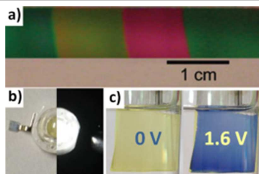
Fig. 37 (a) A series of ZIF-8 films of different thickness on a silicon substrate, from ref. 274 ; (b) photograph of a white LED fabricated using a cadmium based MOF loaded with an iridium base complex without (left) and with a 150 mA current applied (right), from ref. 273 ; (c) photos of the electrochromism of a zirconium based MOF thin film on FTO electrode before (left) and after (right) applying a 1.6 V potential, from ref. 272
