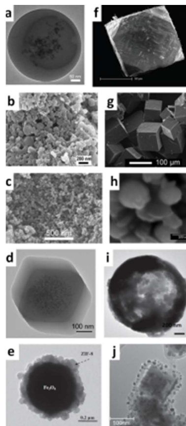
Fig. 23 Electron microscopy images of different MFCs obtained in literature. a) \text{Fe}_3\text{O}_4@\text{Zn}(\text{bix})(\text{NO}_3) from Imaz et al. 214 ; b) \text{Fe}_3\text{O}_4@\text{HKUST-1} from Ke et al. 210 ; c) \text{Fe}_3\text{O}_4@\text{HKUST-1} from Lohe et al. 204 ; d) \text{Fe}_3\text{O}_4@\text{ZIF-8} from Lu et al. 215 ; e) \text{Fe}_3\text{O}_4@\text{ZIF-8} from Zhang et al. 216 ; f) \text{Co}@\text{MOF-5} from Falcaro et al. 203 ; g) \text{NiFe}_2\text{O}_4@\text{MOF-5} from Doherty et al. 23 ; h) \text{Fe}_3\text{O}_4@\text{Cu}(\text{bpy}) from Arai et al. 217 ; i) \text{Fe}_3\text{O}_4@\text{ZIF-8} from Carné-Sánchez et al. 211 ; j) (\text{Fe}_3\text{O}_4@\text{SiO}_2)@\text{HKUST-1} from Silvestre et al. 218
