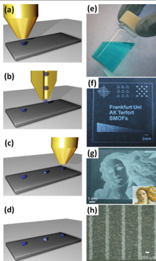
Fig. 18 a-d) Schematic showing the ink-jet printing process for depositing MOF precursor solutions onto various substrates. e) HKUST-1 ink solution containing ethylene glycol f) patterns, letters, and a gradient wedge printed onto PET foil g) Botticelli's “Venus” (original shown inset) was printed in HKUST-1, demonstrating the ability of this approach to pattern large areas. h) The resolution of this method was tested by printing an array of lines 200 \mu\text{m} wide. To enhance the contrast, pictures f), g), and h) were taken with black paper as background. Images reproduced from Zhuang et al. 184 Video animation provided as ESI.
