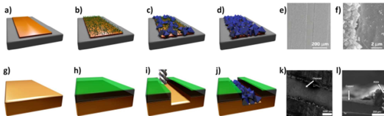
Fig. 9 (a-d) Schematic of the electrochemical method proposed by Ameloot et al. 44 for depositing HKUST-1 on copper substrates. a) A copper pattern (orange) is produced using standard lithographic techniques, and connected as the anode in an electrochemical cell. b) Voltage is then applied, releasing Cu cations into solution. c) The ligand ( H_3BTC ) in solution reacts with the metal cations concentrated near the anode surface, growing the MOF crystals (blue). d) The concentration of the metal precursor remains higher over the uncoated regions of the anode, promoting MOF growth on these areas, resulting in a dense coating. e) SEM measurements performed on the patterned regions and f) detail showing the preferential growth of HKUST-1 on metal. Images have been reprinted with permission from Ameloot et al. 44 g-j) Schematic of MOF patterns produced using precision milling combined with electrochemical deposition. g) A copper substrate is coated with h) a PEEK layer, and (i) a meandering channel is cut via a precision milling process. j) Electrochemical synthesis is then used to deposit HKUST-1 crystals in the channels. SEM images showing the k) top and l) side view of MOF-coated microchannels. SEM images reproduced from Van Assche and Denayer. 100 Video animations provided as ESI.
