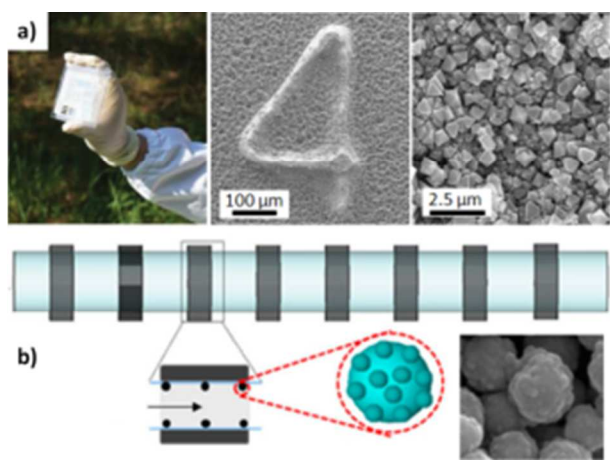
Fig. 39 (a) Sunlight driven photolithography of a Cu plated plastic board for the subsequent HKUST-1 film growth (insets), from Okada et al. 172 ; (b) Schematic of the microfluidic device used for the flow reaction using \text{Fe}_3\text{O}_4@ZIF-8 magnetic framework composite (inset), from Faustini et al. 216
