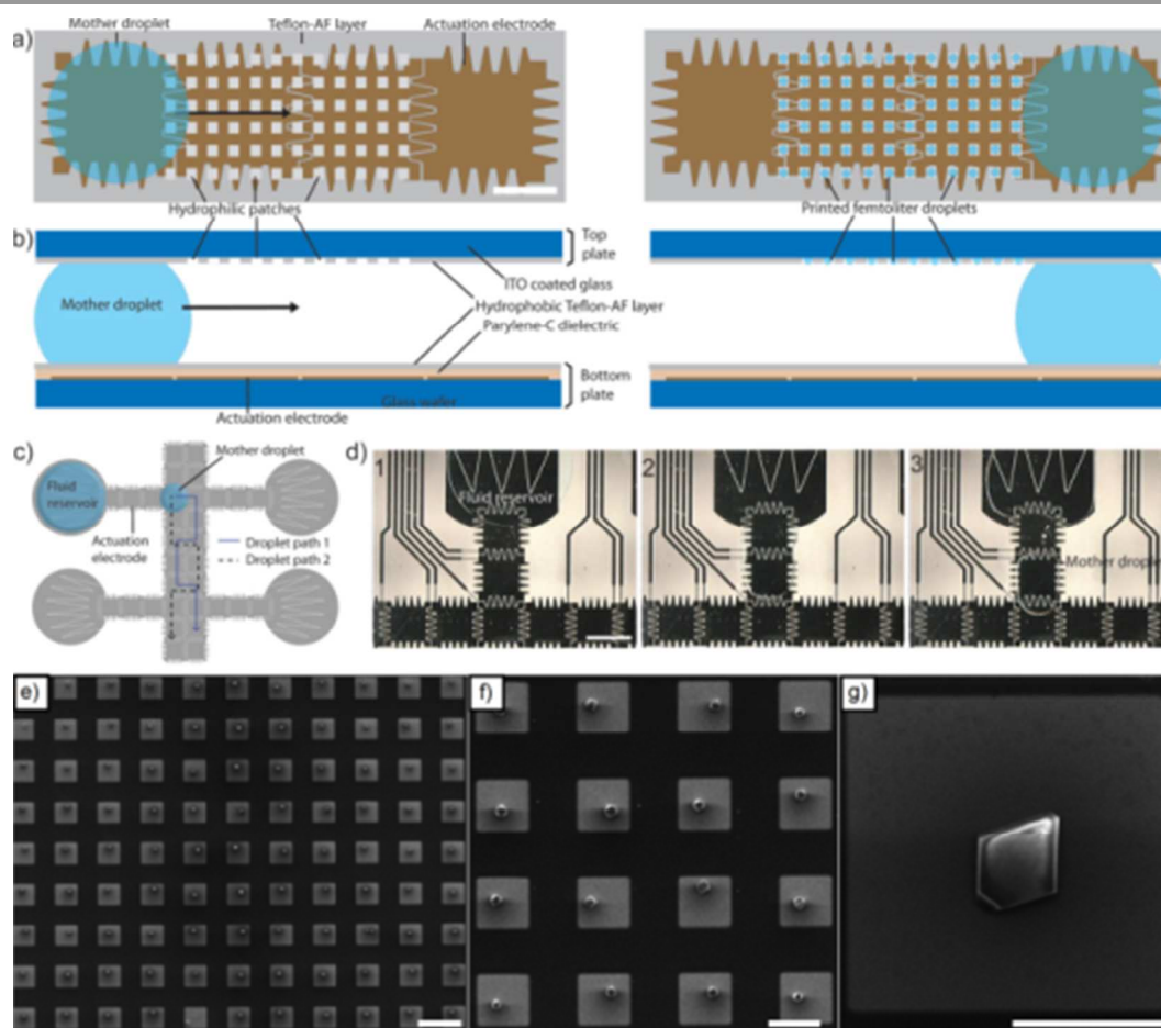
Fig. 14 a-b) Schematic of the digital microfluidic chip implemented by Witters et al. 144 for printing of MOF crystals (scale = 700 \mu\text{m} ). Mother droplets are transported over arrays of hydrophilic-in-hydrophobic micropatches, dispensing femtolitre droplets in the process. c) Schematic illustrating two different paths that could be taken by a mother droplet by applying different actuation sequences to the electrodes. d) Sequence of images from a movie showing how a mother droplet is dispensed from a fluid reservoir onto a path made from actuation electrodes (scale = 1.4 mm). e-g) SEM images of single HKUST-1 crystal arrays produced by controlled evaporation. The square-shaped micropatches (20 \mu\text{m} \times 20 \mu\text{m} ) are ITO in a hydrophobic Teflon-AF matrix, over which a mother droplet has passed. Highly monodisperse single crystals can be observed after controlled evaporation of the solution. Scale bars represent 40 \mu\text{m} (e), 20 \mu\text{m} (f), and 10 \mu\text{m} (g). Reproduced with permission from Witters et al. 144
