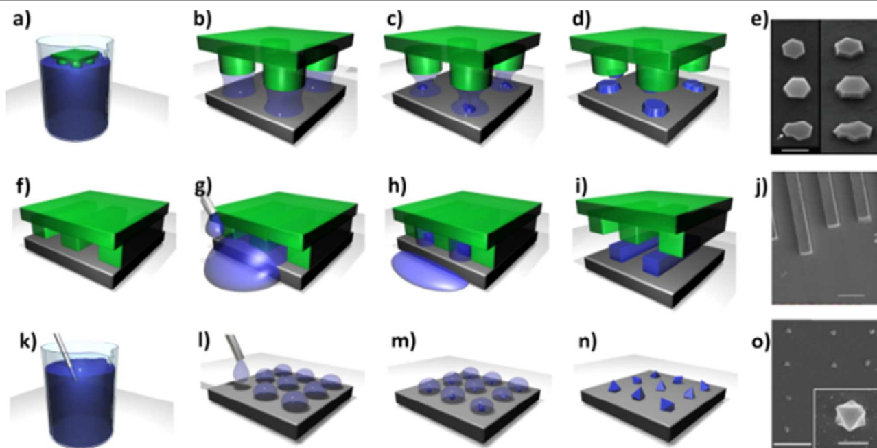
Fig. 12 a-d) Schematic showing the formation of HKUST-1 crystals within confined volumes, using \mu CP combined with controlled solvent evaporation. a-b) A lithographed stamp is wet with a stable precursor solution and placed in contact with the substrate. c-d) The stamp is left in contact with the substrate while the solvent evaporates, producing well-defined MOF crystals. e) SEM image of the HKUST-1 crystal patterns obtained (scale bar 1 mm). Reproduced with permission from Ameloot et al. 102 f-i) Schematic showing the coordination polymer line patterns obtained using the MIMIC process. f) A dry stamp is placed in contact with the substrate. g-h) a droplet of solution is dispensed at the edge of the stamp, filling the channels by capillary forces. i) The solvent is allowed to evaporate, leaving a pattern which follows the contours of the stamp. j) FESEM image of coordination polymer line patterns (scale bar 10 \mu m). Reproduced with permission from You et al. 136 k-o) Schematic of the pen-type lithography method for fabricating single crystal MOF arrays. l) Droplets are dispensed by bringing a microfluidic pen into contact with a substrate. m-n) MOF crystals are then grown by controlled evaporation of the solvent. h) FESEM image of an array of HKUST-1 single crystals formed on a gold substrate prepared with \text{CH}_3 -terminated functional groups. Scale bar 5 \mu m and inset 500 nm. Reproduced with permission from Carbonell et al. 137 Video animations provided as ESI.
