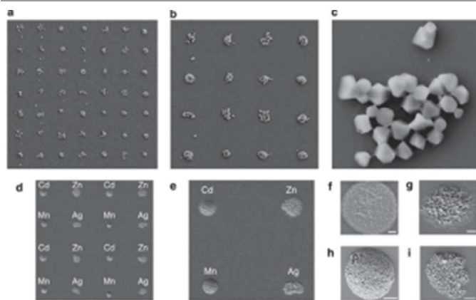
Fig. 13 a-c) FESEM images of an HKUST-1 crystal array (feature distance = 25 \mu\text{m} ), produced using pen-type lithography. d-e) FESEM images of a multiplexed 4x4 array of crystalline PBAs with general formula \text{M}_3[\text{Co}(\text{CN})_6]_2 , where M is Cd(II), Zn(II) and Mn(II), and \text{Ag}_3[\text{Co}(\text{CN})_6] (feature distance = 25 \mu\text{m} ), illustrating the mixing capabilities of this technique. (f-i) FESEM images of individual deposits of f) Cd(II)-PBA, g) Zn(II)-PBA, h) Mn(II)-PBA, and i) Ag(I)-PBA nanocrystals (scale bars, 2 \mu\text{m} ). Reproduced from Carbonell et al. 140
