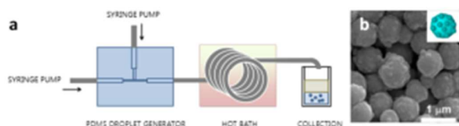
Fig. 26 Microfluidic production and immobilization of Fe 3 O 4 @ZIF-8. a) Schematic of the device used; b) SEM images of magnetic iron oxide nanoparticles successfully coated with ZIF-8 MOF. From Faustini et al. 150
