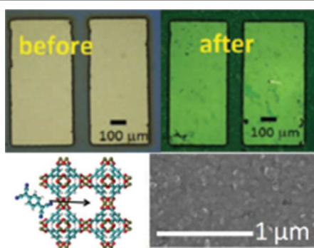
Fig. 35 Optical image of thin MOF film devices before and after TCNQ infiltration (above), schematic of TCNQ molecule entering a HKUST-1 MOF pore, and SEM of the MOF coating (below). Reproduced from Talin et al. 16
