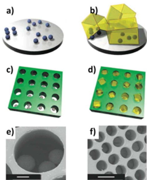
Fig. 11 a-b) Schematics of ceramic particles used for the nucleation of MOF-5 particles. c) A ceramic particle suspension was positioned on the patterned substrate. d) A standard MOF-5 growing medium is introduced for the MOF formation within the membrane holes. SEM images of e) Ceramic particles located in a hole of the substrate (scale bar, 10 \mu\text{m} ), and f) MOF-5 crystals growing within each one of the lithographed holes (scale bar, 50 \mu\text{m} ). 125 Video animation provided as ESI.
