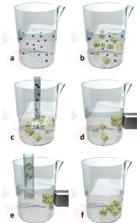
Fig. 22 General synthetic route for MFCs 32 a) dispersion of magnetic particles in the precursors mix; b) reaction mixture after solvothermal or hydrothermal reaction; c) extraction of unreacted magnetic particles after sedimentation of MOFs and MFCs; d) collection of MFC with an external magnet; e) separation of MOFs from MFCs; f) magnetic responsive MFC isolated and purified. Video animation provided as ESI.
