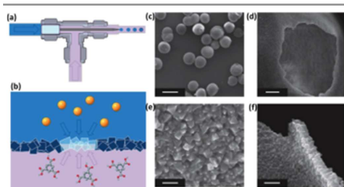
Fig. 16 a) Schematic showing the T-junction used by Ameloot et al. to synthesise hollow MOF spheres. Individual droplets of an aqueous metal-ion-containing solution (blue) are suspended within a flowing organic ligand solution (purple) using a tapered capillary positioned within the T-junction. b) The metal cations encounter the organic linkers at the surface of the droplet, resulting in the localised formation of MOF crystals. c-f) SEM of the hollow HKUST-1 spheres. c) The capsules retain their spherical shape upon drying and are highly monodisperse in size (scale bar 500 \mu\text{m} ). d) The hollow interior of the sphere is revealed by creating a hole with a needle (scale bar 25 \mu\text{m} ). e) Detail of the defect-free capsule wall. The gaps between larger crystals are sealed by smaller crystals (scale bar 2 \mu\text{m} ). f) Cross-sectional view of the capsule wall, showing its thin and uniform thickness (scale bar 2 \mu\text{m} ). 152
