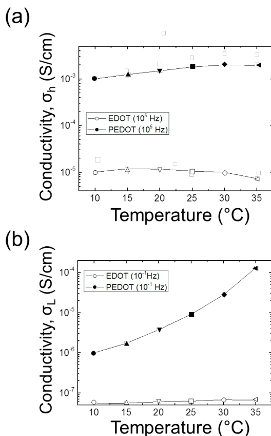
Figure 14. Effective conductivity comparison between EDOT and PEDOT gels at 10^5 Hz (top) and 10^{-1} Hz (bottom).
