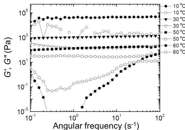
Figure 9. Storage modulus ( G' , filled circles) and loss modulus ( G'' , empty circles) as a function of frequency ( \omega ) during heating sweep (from low to high frequency) of EDOT gels.
