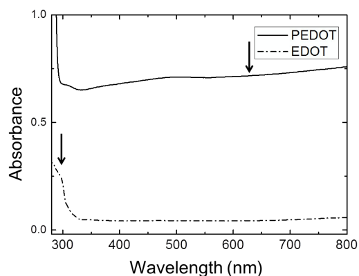
Figure 4. UV-vis absorbance spectrum of PEDOT gel (solid line) and EDOT gels (dot-dashed line).
