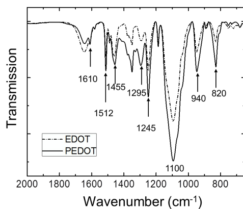
Figure 5. FT-IR spectrum of PEDOT gel (solid line) and EDOT gel (dot-dashed line).
