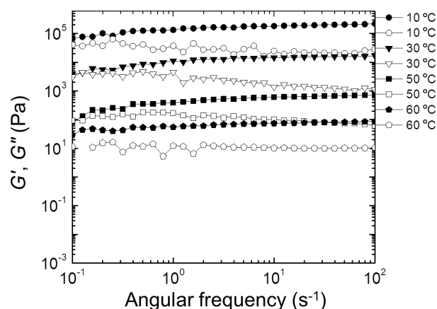
Figure 10. Storage modulus ( G' , filled circles) and loss modulus ( G'' , empty circles) as a function of frequency ( \omega ) during heating sweep (from low to high frequency) of PEDOT gels.
