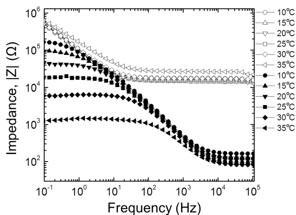
Figure 12. AC impedance of EDOT gels (open symbols) and PEDOT gels (filled symbols).
