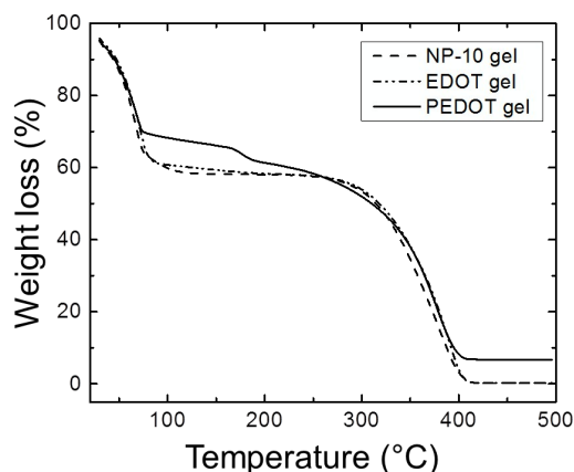
Figure 6. TGA spectrum of NP-10 gel (dashed line), EDOT gel (dot-dashed line), and PEDOT gel (solid line).
