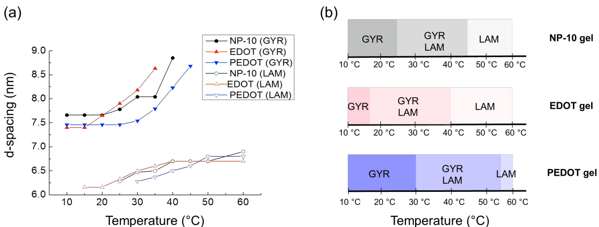
Figure 8. (a) Change of d-spacings determined from the primary (211) cubic peak q^* and the lamellar peaks from each synchrotron SAXS pattern (Figure 7), (b) nanostructure changes as a function of temperature.
