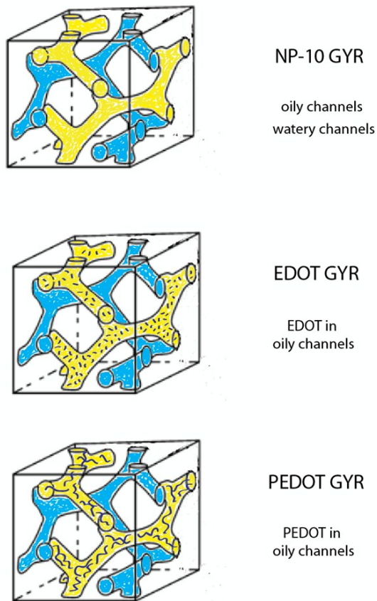
Figure 1. Schematic diagram of the bicontinuous cubic phases (gyroid, GYR, with Ia\bar{3}d lattice symmetry) formed by chemical polymerization of EDOT in an ordered NP-10 surfactant mesophase. The original NP-10 GYR phase (top) is infiltrated with EDOT monomer in the oily channels (middle), and then polymerized to PEDOT (bottom).
