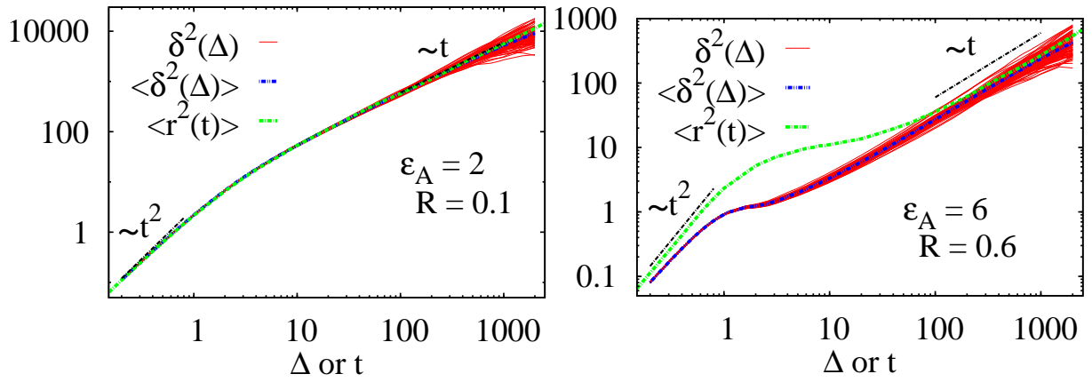
Figure 7: MSD \langle r^2(t) \rangle (green curves) and time averaged MSD \overline{\delta^2(\Delta)} defined in Eq. (16) (red curves), as well as the ensemble average \langle \delta^2 \rangle (blue curves) over the simulated trajectories. Parameters are as indicated in the panels, the number of traces used for averaging is N = 100 , and the length of the trajectories is T = 10^4 corresponding to 10^7 simulation steps.
