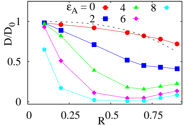
Figure 4: Long-time diffusivity D(\phi)/D_0 in the terminal Brownian regime as function of the obstacle size, plotted for varying tracer-obstacle attraction strengths. Other parameters are the same as in Fig. 3. The dotted line represents the prediction by Eq. (10) for inert obstacles. The data sets for varying adsorption strength are shown as filled symbols.
