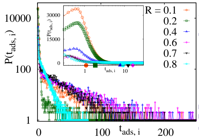
Figure 5: Histograms P(t_{ads,i}) of individual binding times t_{ads,i} spent in the obstacle-adsorbed state by the tracer particles, plotted for the parameters of Fig. 3 with attraction strength \epsilon_A = 6k_B\mathcal{T} . The mean values \langle t_{ads} \rangle for each crowder radius are indicated as the dots on the horizontal axis of the inset with the corresponding colour, indicating a non-monotonic behaviour with R . The main graph is shown in log-linear scale to show the exponential tails of the distributions, whereas the inset features a linear-log scale. The total length of the simulated trajectories is 10^7 steps. The obstacle radius R is given in the legend in terms of R_{\max} = a/2 .
