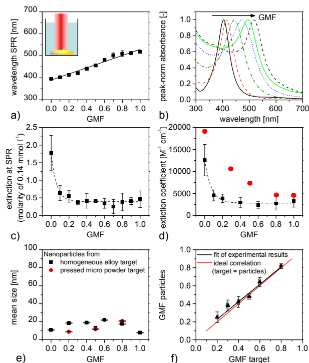
Fig. 6 PLAL of bulk alloy targets in pure water causes homogeneous alloy NP formation a) Wavelength of surface plasmon resonance peak of Ag-Au nanoparticle colloids generated during 60 s PLAL of alloy bulk as a function of GMF and b) Peak-normalized UV-Vis spectra of colloids; c) extinction at SPR at the molarity of 0.14 mmol l -1 and d) extinction coefficient as a function of GMF. Red circles present values taken from Link et al. 6 e) Number weighted particle size as a function of GMF. These values were taken from the peak maxima of log normal-fitted particle size distributions from TEM images f) Correlation of GMF of laser-generated nanoparticles measured by TEM-EDX with GMF of the bulk alloy targets.
