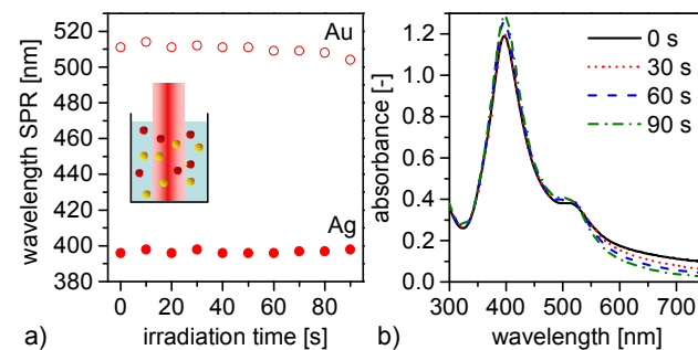
Fig. 4 Post-irradiation of Au and Ag colloidal mixtures reveals no alloy formation but isolated particle fractions a) Wavelength of surface plasmon resonance of Ag and Au, respectively, as a function of irradiation time; b) spectra of Ag and Au colloidal solution after different times of post-irradiation.
