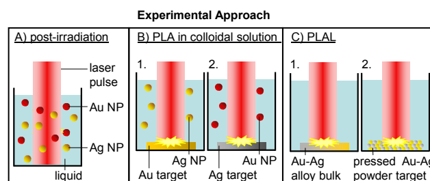
Fig. 3 Experimental approach divided in A) post-irradiation, B) pulsed laser ablation in colloidal solution and C) pulsed laser ablation of 1. bulk alloy and 2. pressed Ag-Au microparticle powder target.
