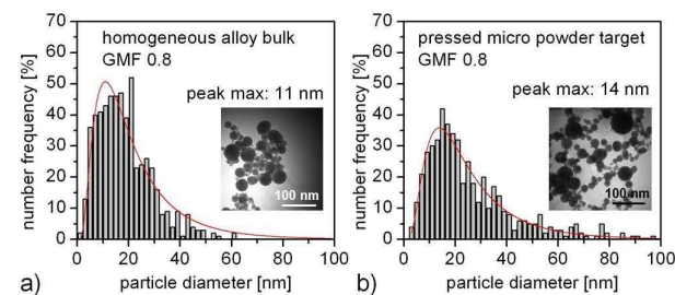
Fig. 9 Representative TEM images and size distribution of NPs generated during PLAL of homogeneous alloy bulk (a) and of pressed micro powder target (b) with GMF 0.8.
