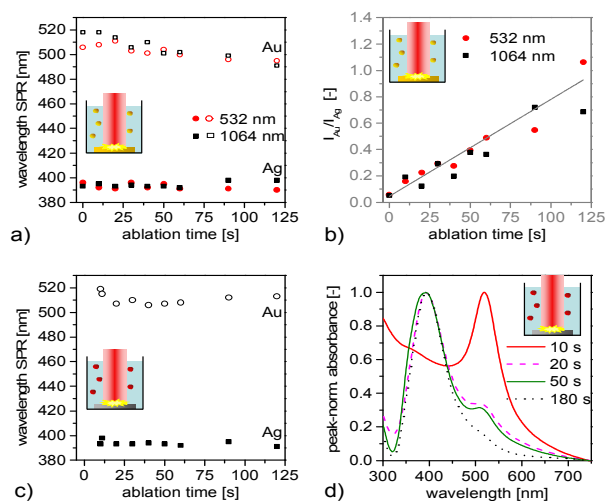
Fig. 5 Nanosecond laser ablation of metal targets in the presence of colloidal nanoparticles (a, b: Au targets + Ag colloids; c, d: Ag targets + Au colloids) shows no significant alloying. a) Wavelength of SPR peak position of Au in relation to Ag as a function of ablation time during PLAL (at laser wavelength of 1064 nm and 532 nm) of Au in Ag NP colloidal solution; c) Wavelength of SPR of Au and Ag as a function of ablation time during PLAL of Ag in Au NP colloidal solution; d) Peak-normalized spectra of Ag and Au NP colloidal solution during PLAL of Ag in Au NP colloidal solution at different ablation times.
